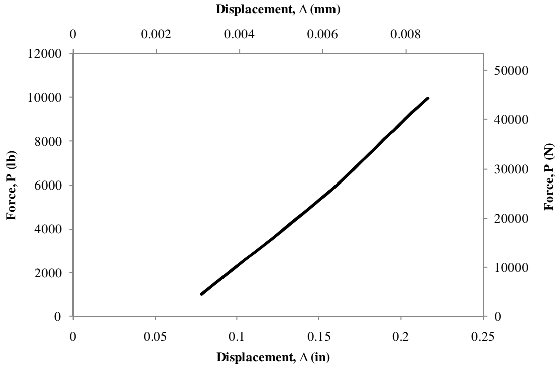
Figure 5.27: Stiffness of the strengthened slab
