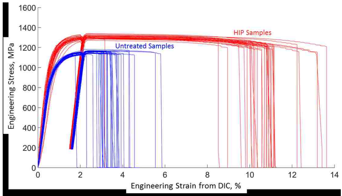
Figure 19: Engineering stress strain curves of 33 HIP processed (red) and 34 untreated (blue) AM tensile bars.
