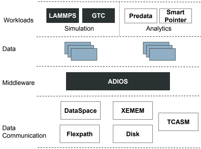
Figure 2.1: System software support for in situ analytics
