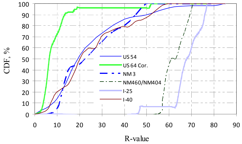
Figure 4.4 Cumulative distribution function (CDF) plot for field R-value data
