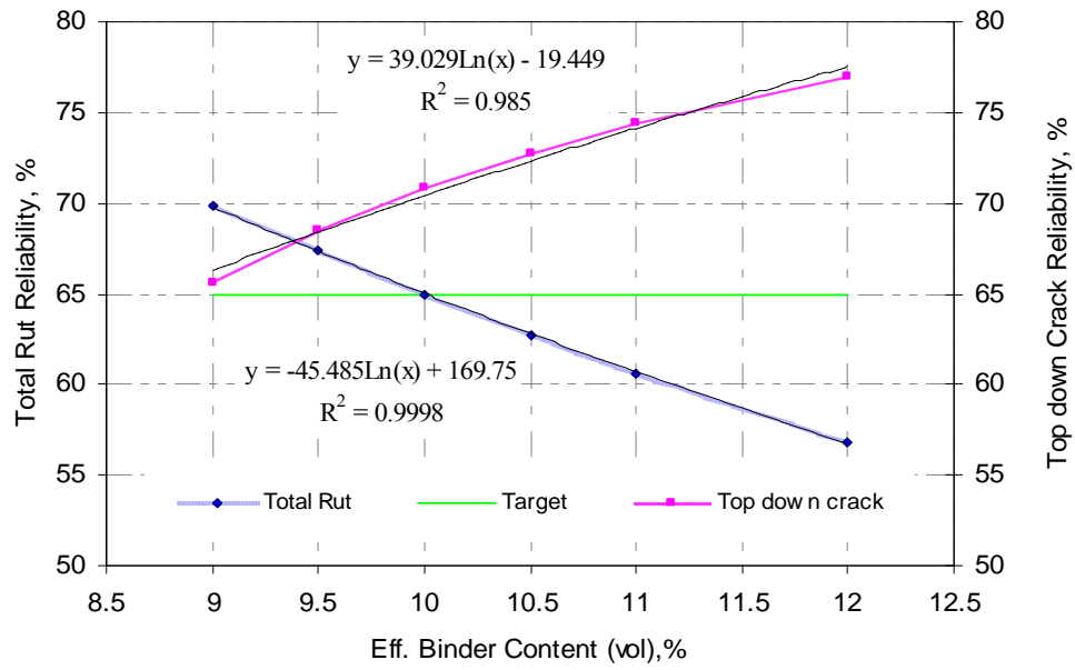
Figure 5.7 Effect of volumetric effective binder content on total rutting and top-down cracking reliability (NM 460/ NM 404)
