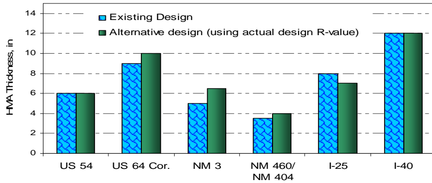
(a) Existing design vs. alternative design (using actual design R-value )
