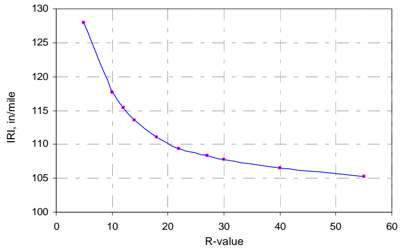
(b) International roughness index (IRI)
