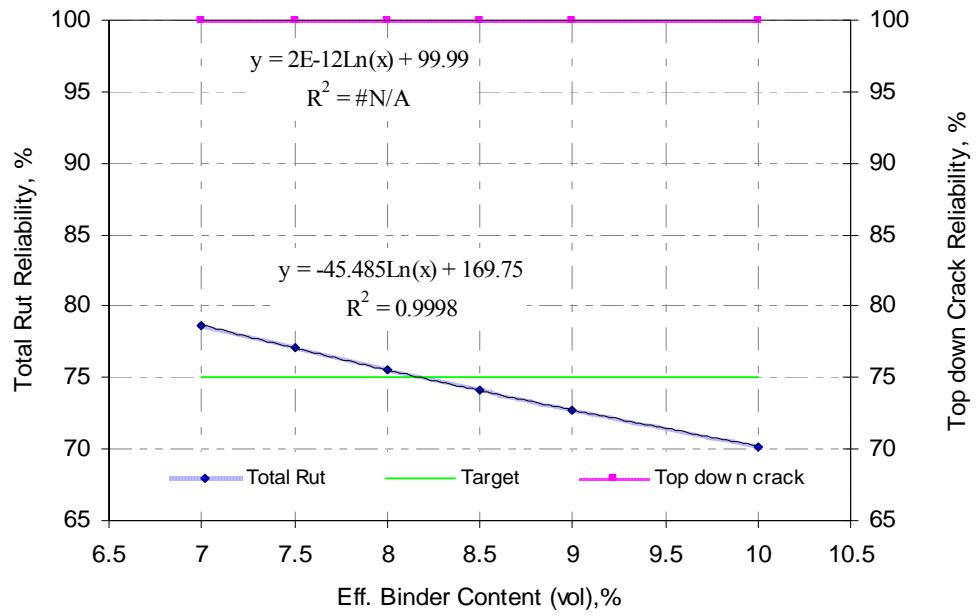
Figure 5.5 Effect of volumetric effective binder content on total rutting and top-down cracking reliability (US 64 Corridor)
