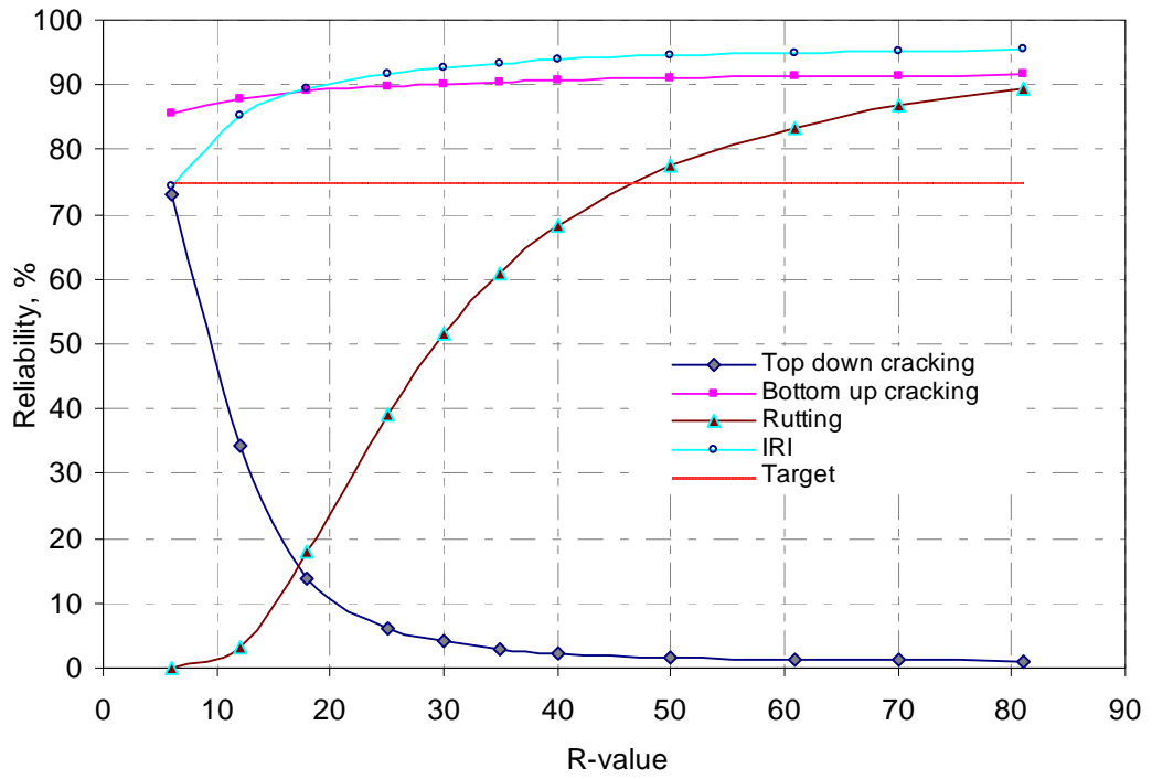
Figure 4.7 Evaluation of minimum R -value with MEPDG reliability output for US 54
