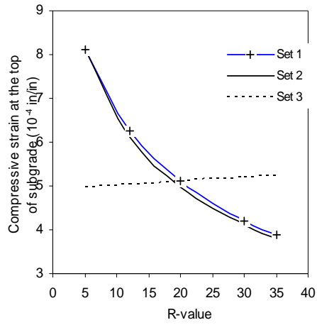
(a) Compressive strain vs. R-value
