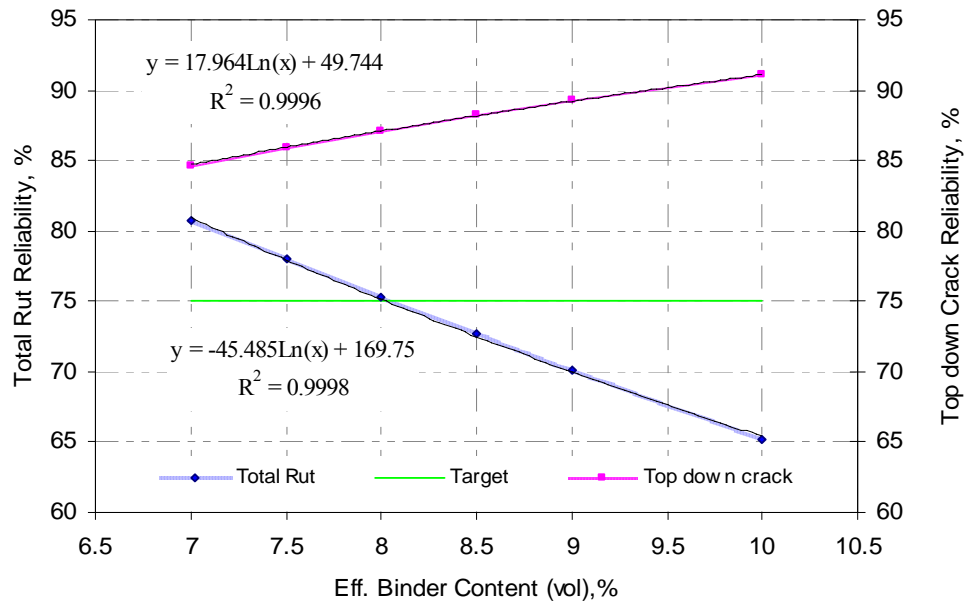
Figure 5.4 Effect of volumetric effective binder content on total rutting and top-down cracking reliability (US 54)
