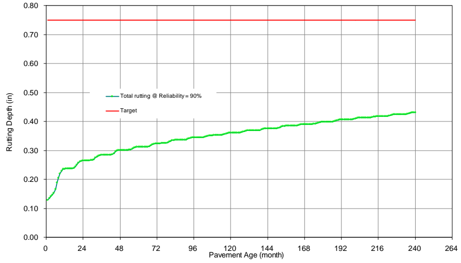
(a) Total rutting
