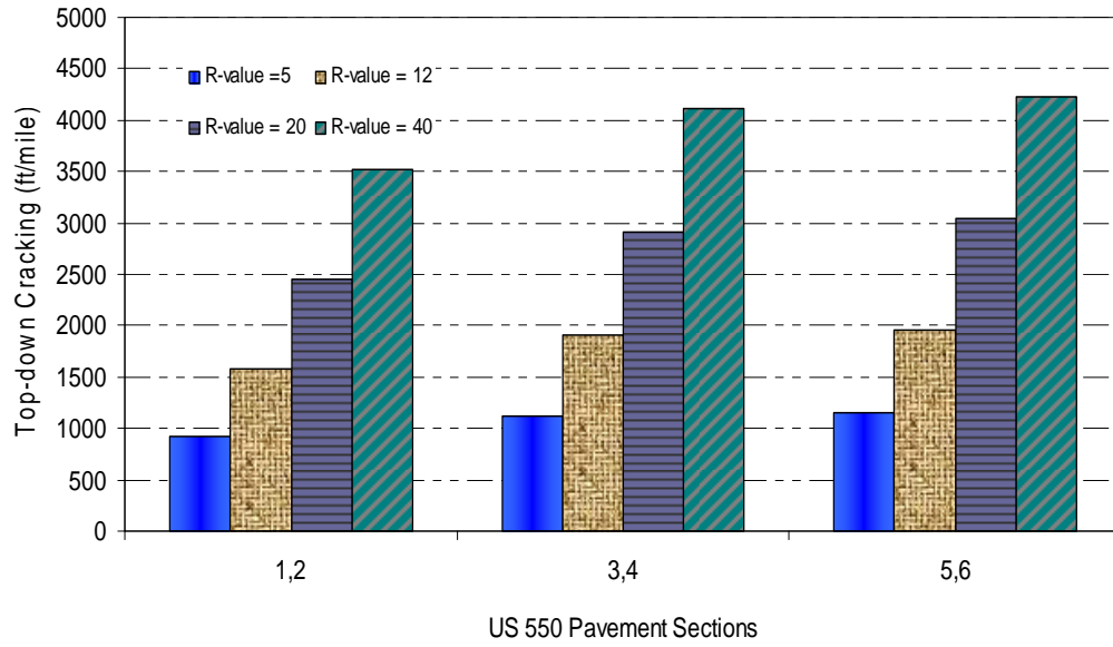
Figure 3.6 Effect of R-value on top down cracking
