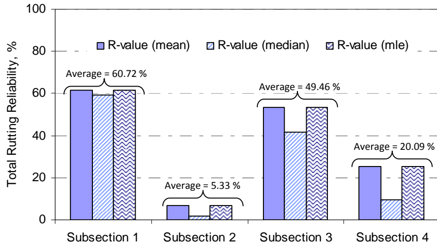
Figure 4.6 Comparison of total rutting reliability between sub-sections (US 54)
