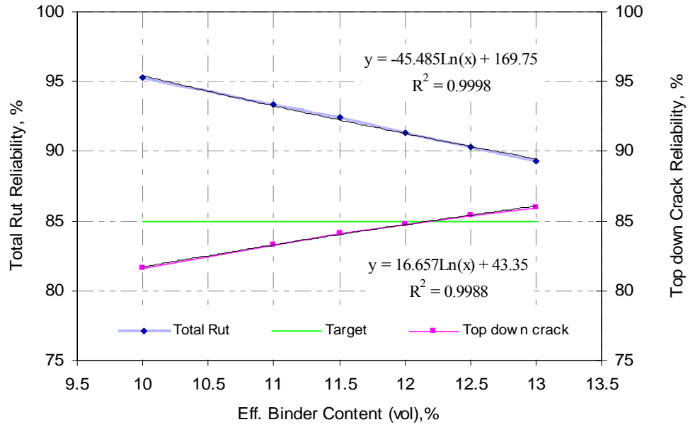
Figure 5.8 Effect of volumetric effective binder content on total rutting and top-down cracking reliability (I-25)
