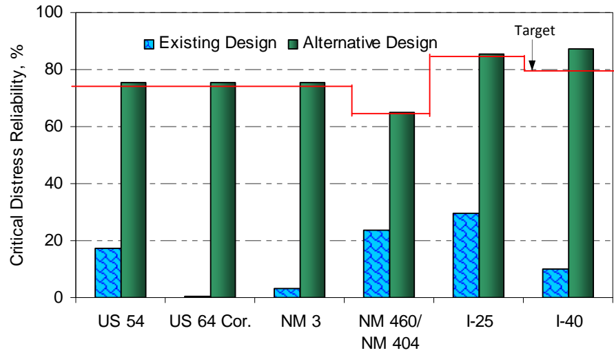
Figure 5.14 Comparison of reliability for existing design and alternative design
