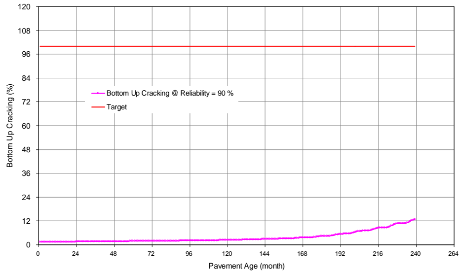
(b) Bottom up cracking
