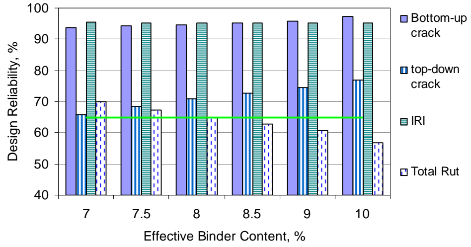
Figure 5.2 Effect of effective volumetric binder content on reliability (NM 460/NM404)
