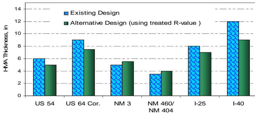
(b) Existing design vs. alternative design (treated subgrade: considering mean R-value )
