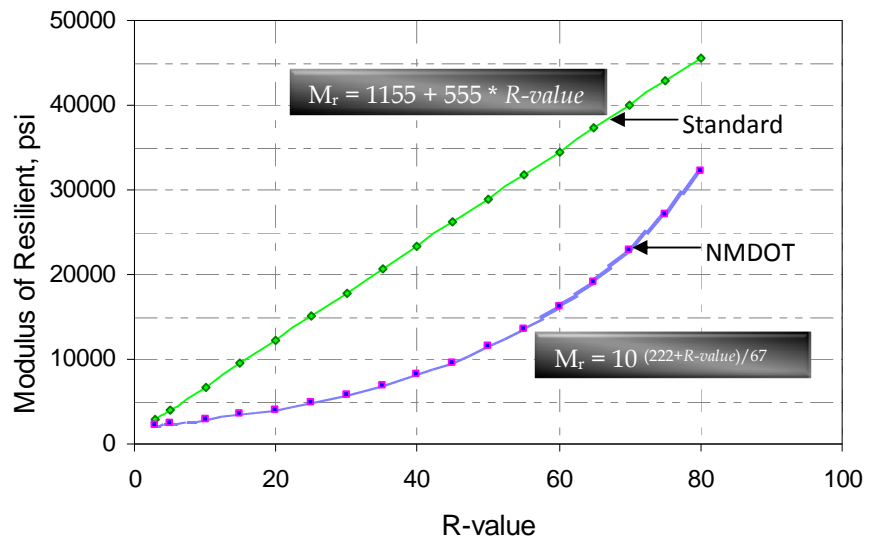
Figure 2.1 Comparison of standard and NMDOT equation for R -value- M_r conversion
