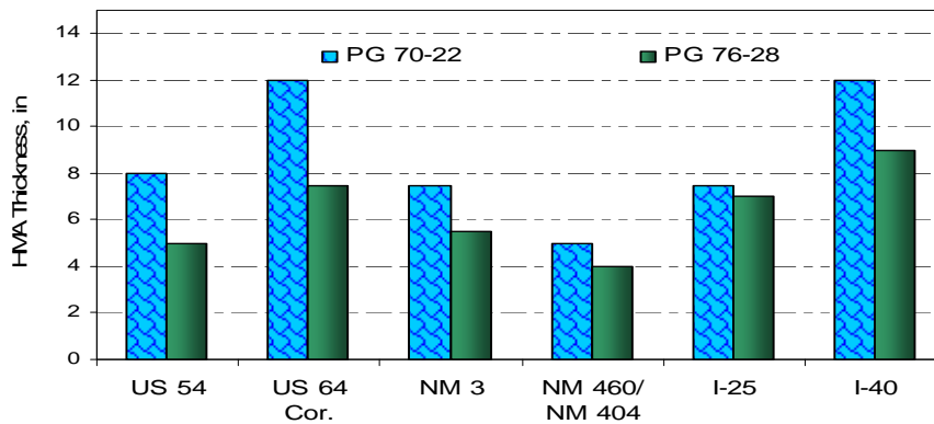
(c) Alternative designs: PG 70-22 vs. PG 76-28
