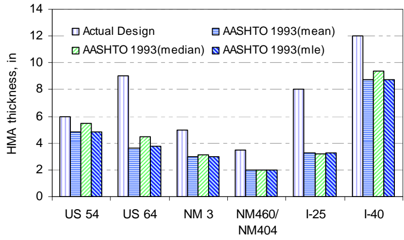
Figure 5.1 Comparison of HMA thicknesses for statistical R-value with actual designed thickness
