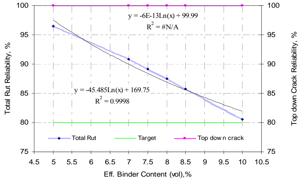
Figure 5.9 Effect of volumetric effective binder content on total rutting and top-down cracking reliability (I-40)
