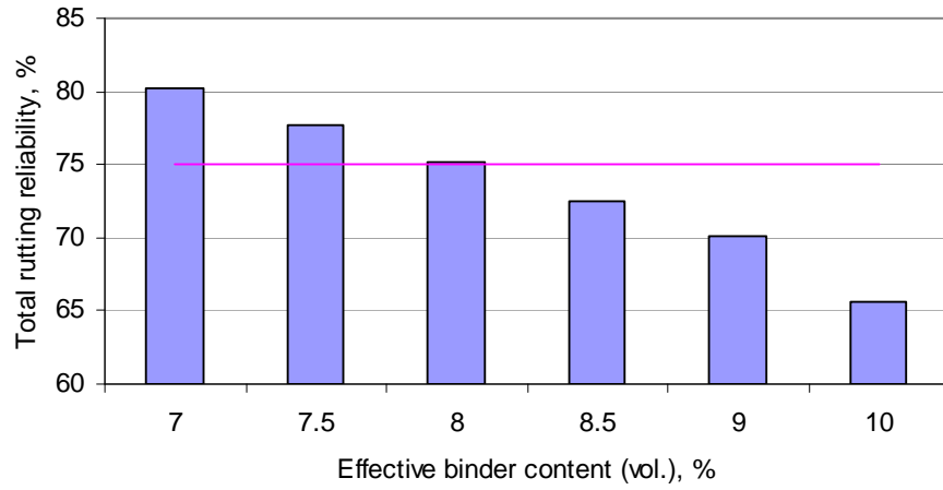
Figure 5.3 Effect of volumetric effective binder content on total rutting reliability (US 54)
