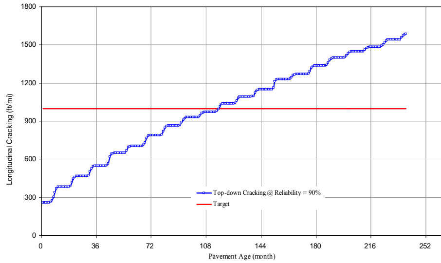
(a) Top down cracking
