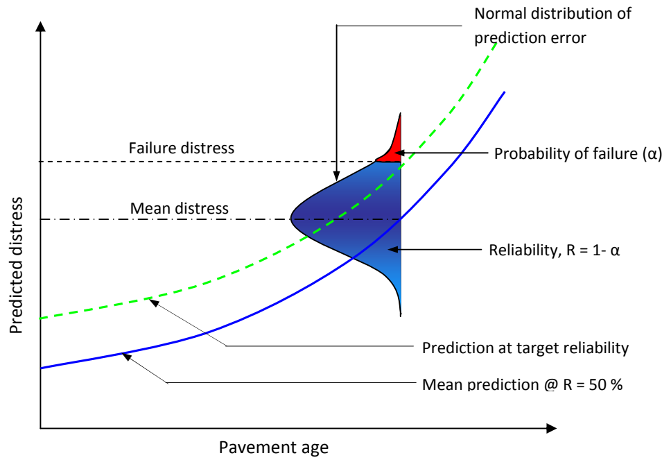
Figure 2.2 Design reliability concept of MEPDG for a given distress
