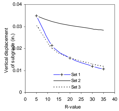
(b) Vertical displacement vs. R-value
