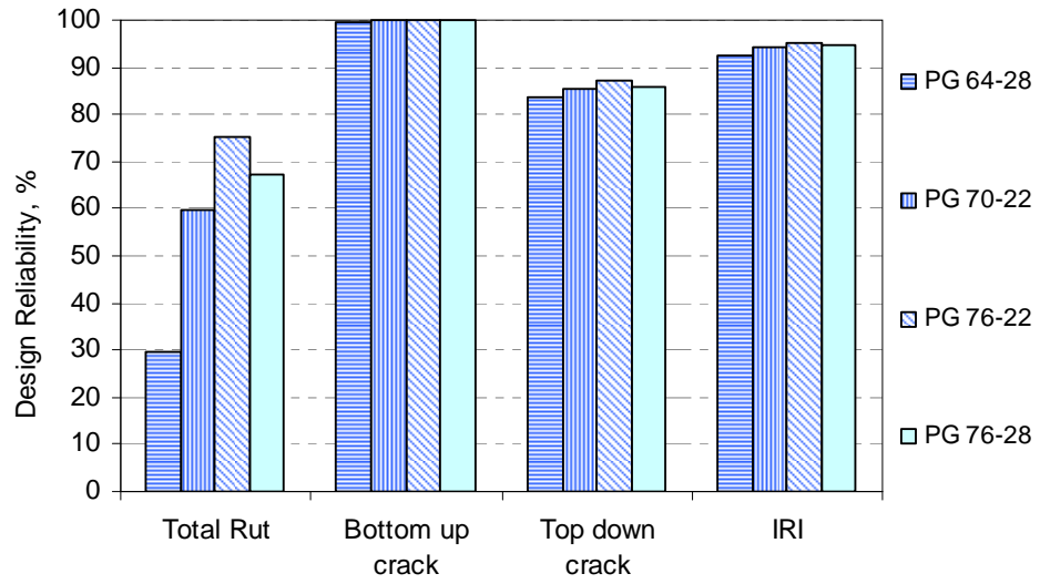
Figure 5.10 Effect of variable binder performance grade on reliability (US 54)
