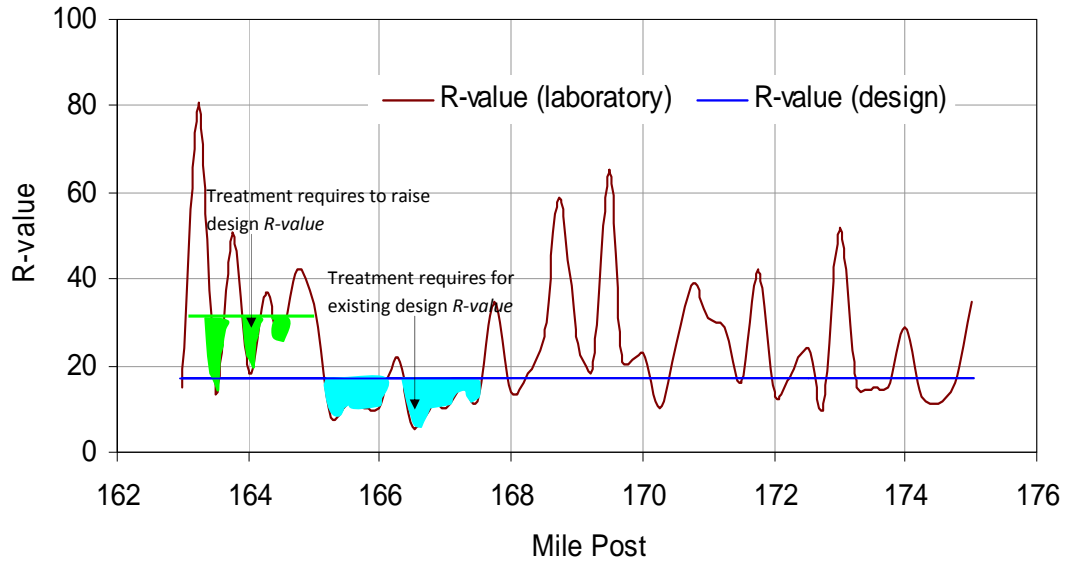
Figure 4.1 Variation of R-value along longitudinal section (US 54)
