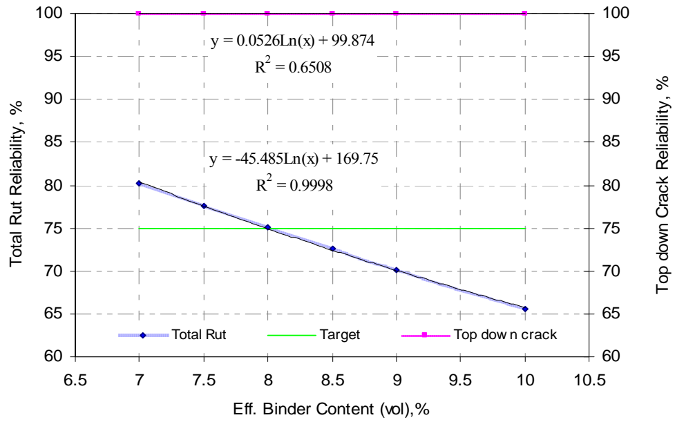
Figure 5.6 Effect of volumetric effective binder content on total rutting and top-down cracking reliability (NM 3)
