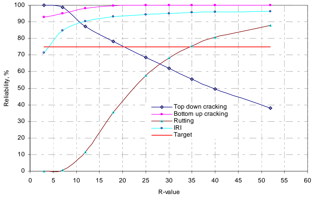
Figure 4.8 Evaluation of minimum R -value with MEPDG reliability output for US 64
