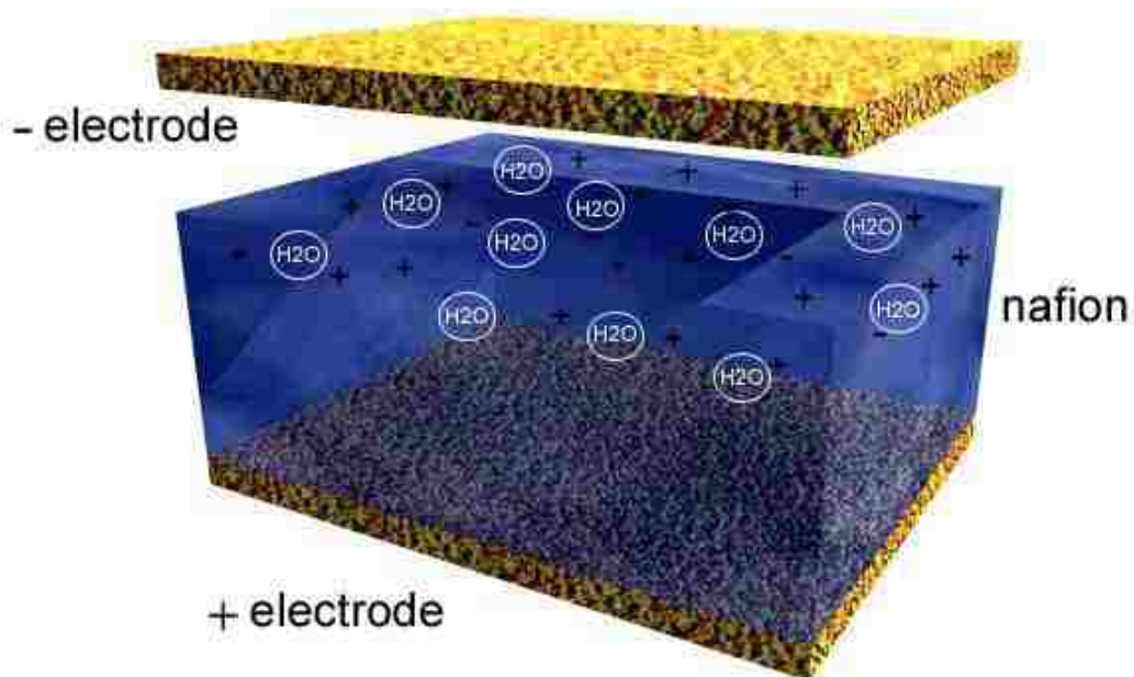
Figure 21. Cation redistribution
