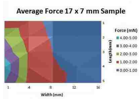
Figure 19. Average force rectangular IPMC
