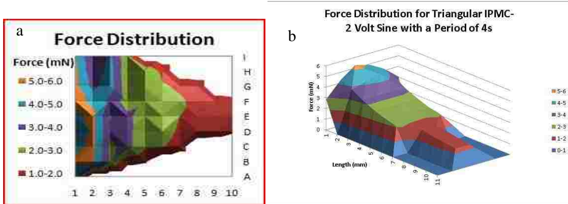
Figure 59. Force distributions for a triangular IPMC. From left to right, a) experimental and b) force simulation
