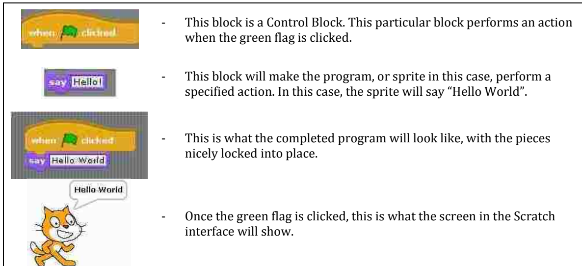
Figure 3: Scratch Syntax [8]
