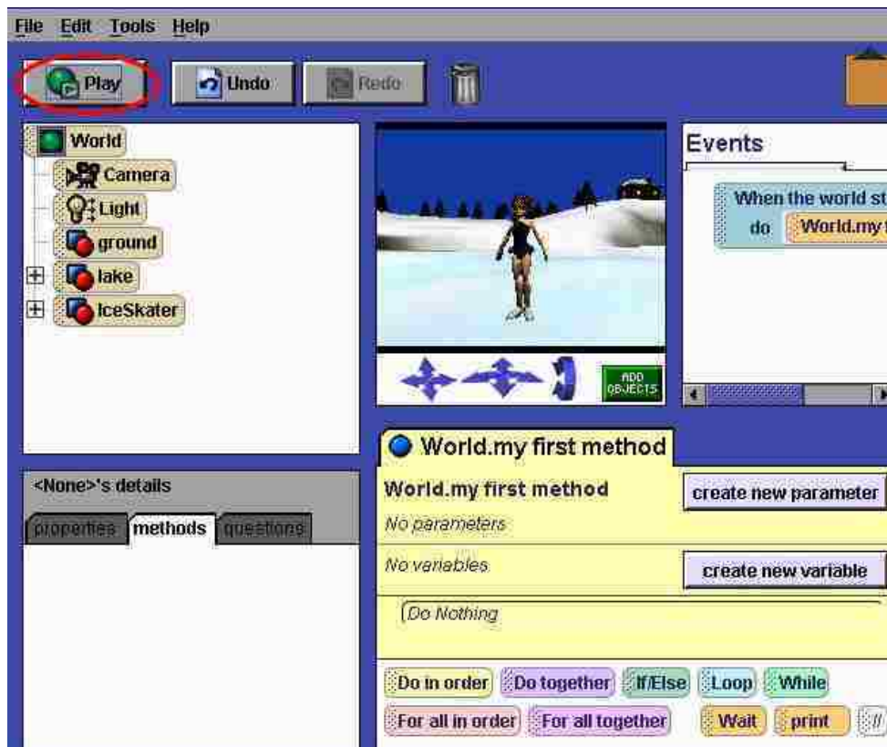
Figure 2: Example Program using Alice [5]
