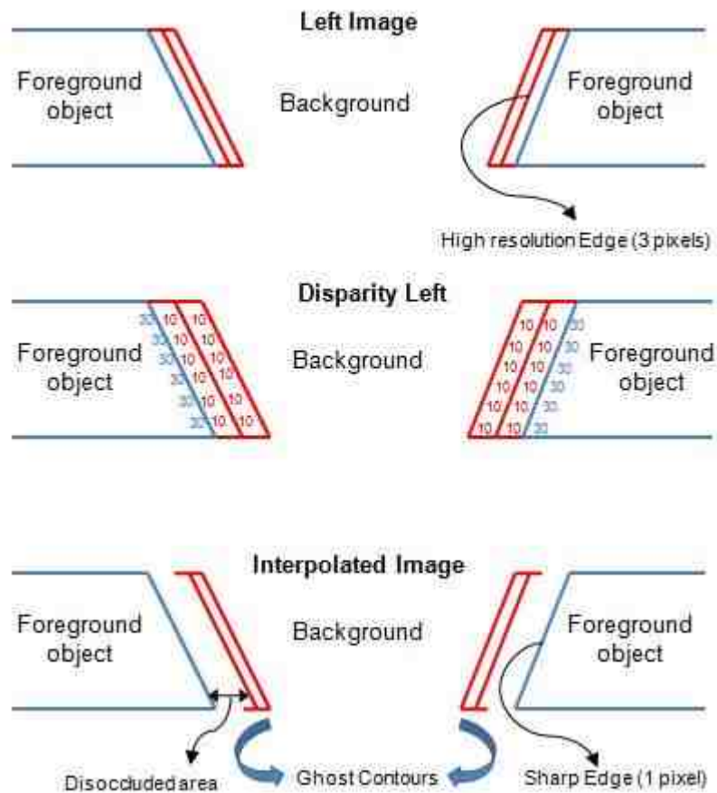
Figure 6.1: Demonstrating ghost contours problem
