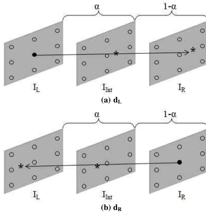
Figure 3.2: Shows forward disparity estimation: (a) disparity compensation from left-to-right; (b) disparity compensation from right-to-left.
