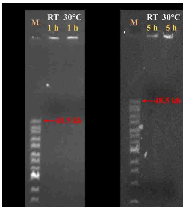
Fig. 3.5 Agarose gel (0.5%) electrophoresis of 1 kb extended marker (M) and RCPs of RCA reaction at RT and 30°C for 1 h (A) or 5 h (B).
