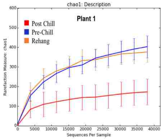
Figure 5. Chao 1 rarefaction curve.
