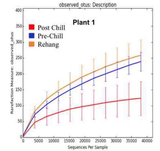
Figure 6. OTU rarefaction curves.
