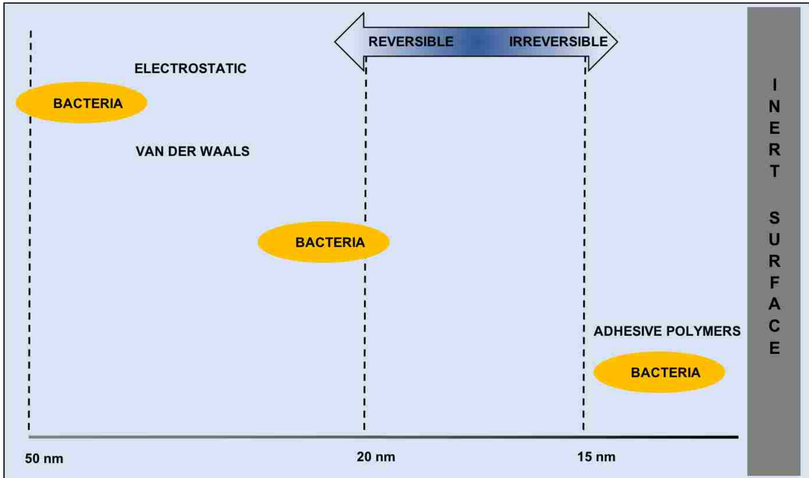
Figure 3C. Three-stage process of bacterial attachment. Adapted from Busscher and Weerkamp, (1987)
