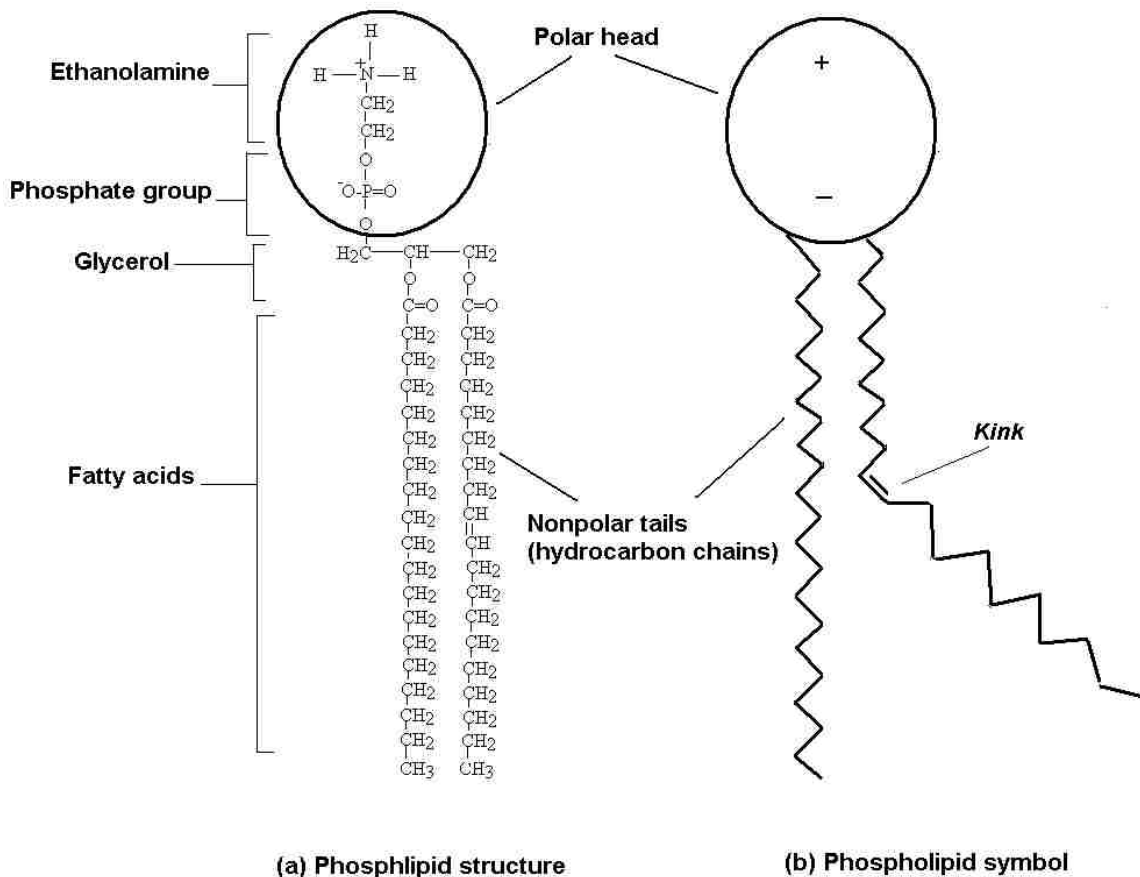
Figure 2.3: The membrane phospholipids and its amphipathic nature. (a) A phospholipid molecule consists of a polar head and two fatty acids (nonpolar tails) attached by a glycerol backbone. PE is an example of the membrane phospholipids, where the polarity of the head results from a positively charged amino group connected to a negatively charged phosphate one. Note that if the 3 hydrogen atoms bonded to the N atom were replaced by 3 methyl groups ( \text{CH}_3 ) then we would have Phosphatidylcholine (PC or lecithin). (b) A schematic drawing of this phospholipid molecule (PE or cephalin). Such a molecule is called zwitterion (hybrid ion) because it has both positively and negatively charged groups in its structure [12].
