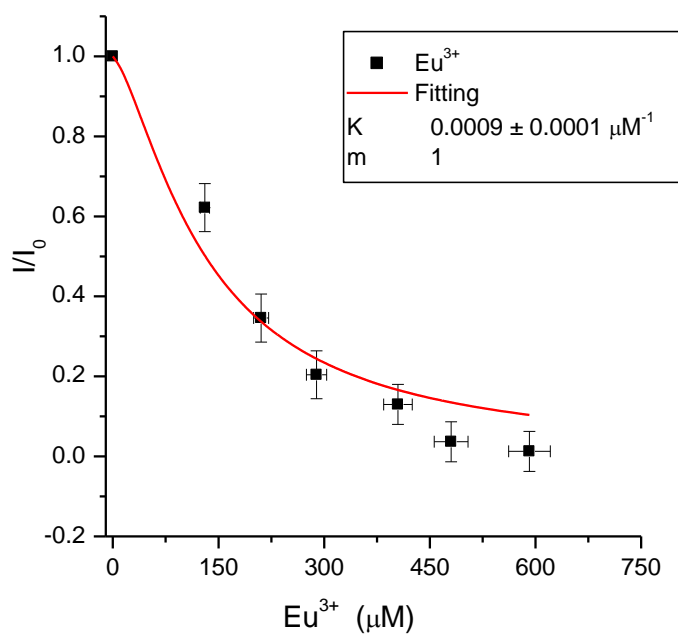
Figure 6.12: Fitting the experimental data of Eu^{3+} .
