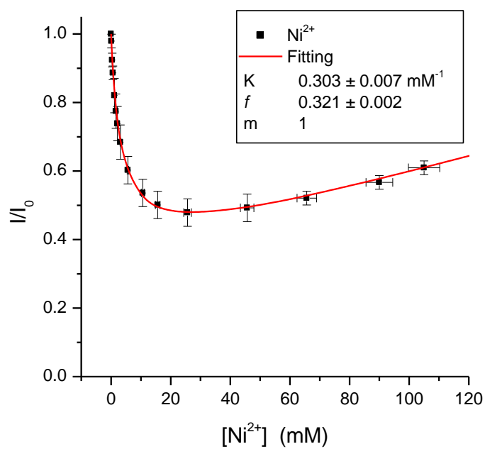
Figure 6.4: Fitting the experimental data of Ni^{2+} .
