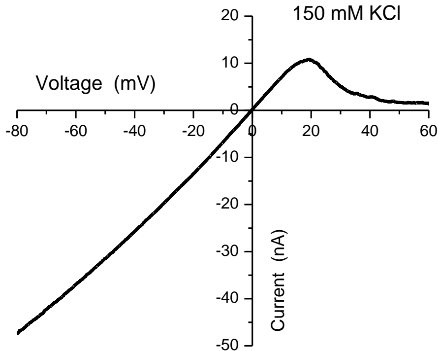
Figure 4.5: Current voltage graph shows the behavior of a population of Lysenin channels in the BLM surrounded by a supporting electrolyte solution of 150 mM KCl, 20 mM HEPES/KOH pH 7. The linearity in the negative voltage shows no rectification, while it can clearly be seen in the positive voltage region due to the voltage-induced gating of Lysenin.
