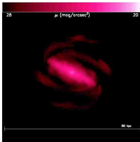
(c) c1 - 2.650 Gyr
