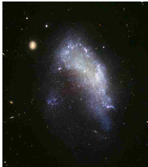
Figure 2.4: An example of an irregular galaxy (NGC 1427A). Image from Wikipedia (2015e), credit AURA, STScI, HST & ESA, NASA.
