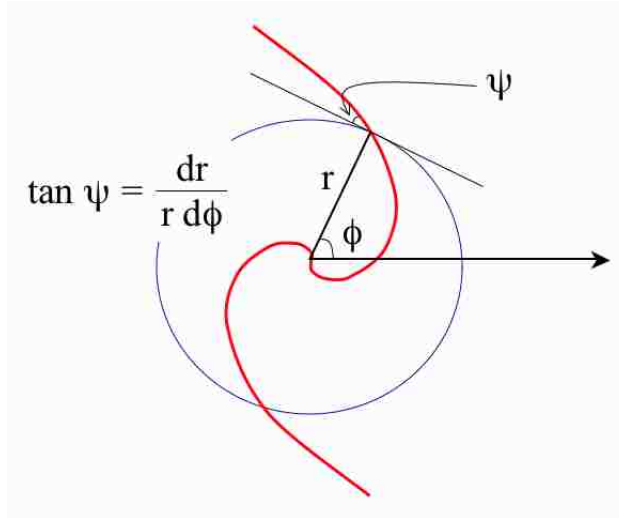
Figure 2.10: The definition of pitch angle, indicated by \psi . Image from Whittle.
