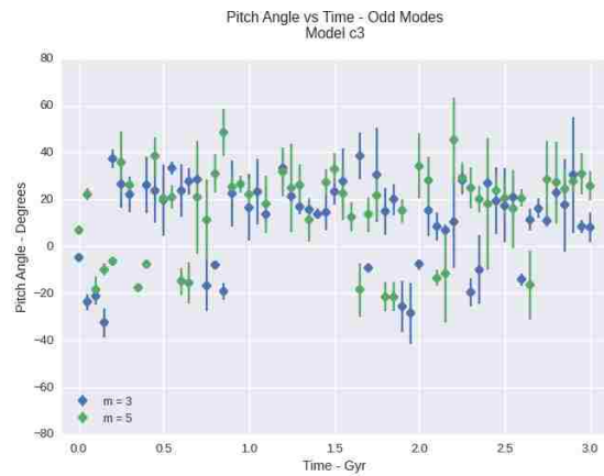
(f) Odd Modes - c3
