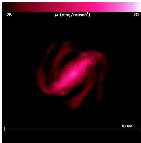
(a) b1 - 2.350 Gyr
