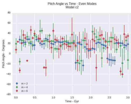
(c) Even Modes - c2
