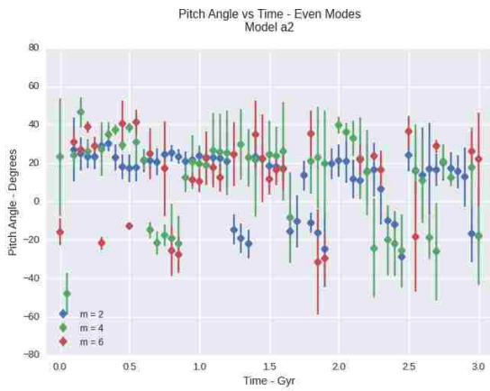
(c) Even Modes - a2
