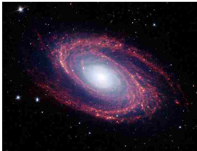
Figure 2.1: An example of a grand design spiral galaxy (M81) with a bulge in the center. Image from Wikipedia (2014b), credit NASA and the Spitzer Space Telescope (SSC & Caltech).
