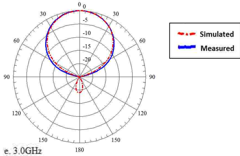
Figure 9.4 Normalized measured and simulated patterns (a) 2.2GHz, (b) 2.4GHz, (c) 2.6GHz, (d) 2.8GHz, and (e) 3GHz
