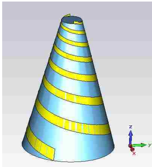
Figure 4.2 Initial spiral arms constructed in CST.
