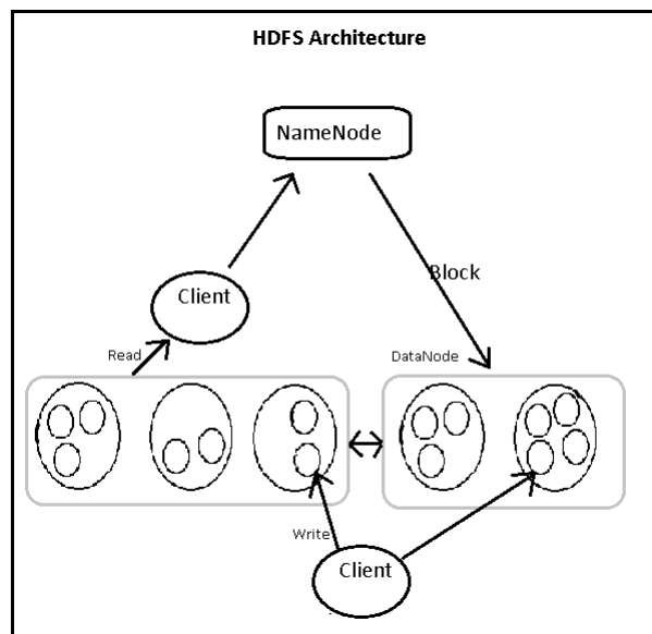
Figure 5.3: HDFS architecture
