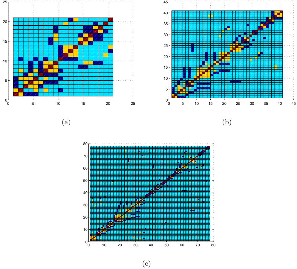
Figure 6.4: \mathbf{D}\mathbf{D}^T for three test systems: (a) IEEE 14-bus (b) IEEE 30-bus and (c) IEEE 57-bus.
