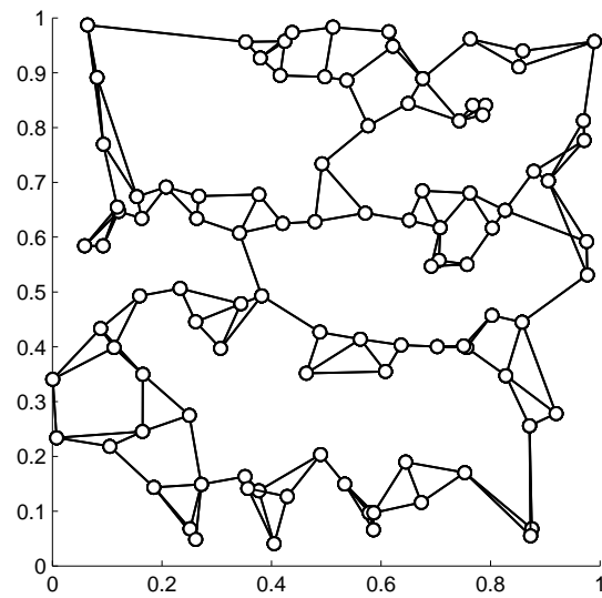
Figure 5.3: Topology of the 100-node GGM.
