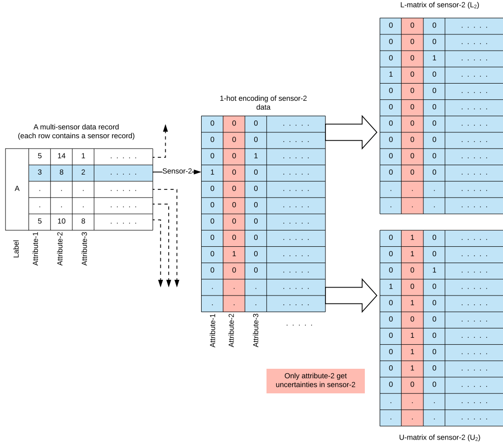
Figure 6.4: Sensor-Specific Uncertainties in Sensor S_2 . Note. Sensor S_2 corresponds to k = 2 . Sensor-specific uncertainty is introduced into the second attribute, i.e., j = k = 2 (pink column in the illustration showing 1-hot encoding of sensor data). This attribute’s true state is a_2 = 8 and its state-space has 16 states, i.e., \Theta_2 = \{0, 1, \dots, 15\} . The size of the focal element B_2 of the SFE uncertainty is randomly picked from the integers lying in [2, |\Theta_2|] = [2, 16] as |B_2| = 6 . The elements of B_2 are chosen s. t. it contains the true value a_2 = 8 while the remaining |B_2| - 1 = 5 states are randomly selected from \Theta_2 \setminus \{a_2\} = \{0, \dots, 7, 9, \dots, 15\} . In this figure, the focal element randomly selected in this manner is B_2 = \{0, 1, 4, 6, 7, 8\} . The PrBound pair [0,1] is introduced into each of the corresponding entry (pink columns in the L- and U-matrices).
