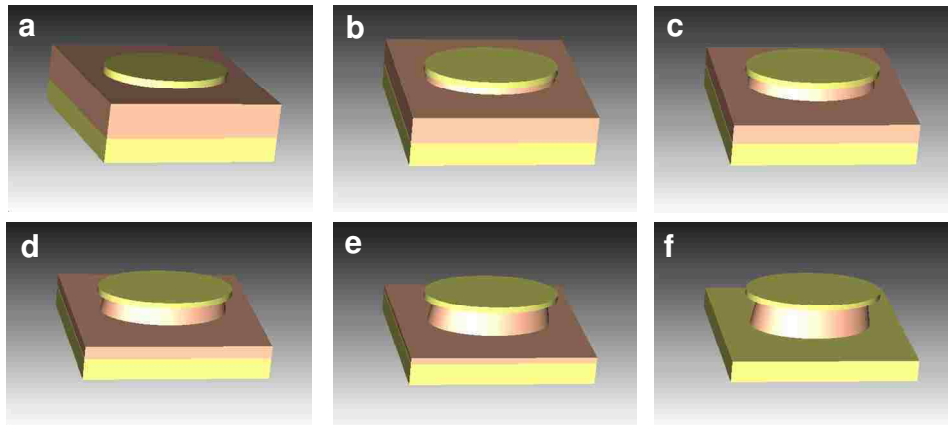
Fig. 6.11 Sequence of schematic views of changing shape and thickness of MAA depending on RIE processing. For example, (a) shows no etched MMA and (f) shows fully RIE etched MAA. The variety results in change of effective refractive index between metal plates.
