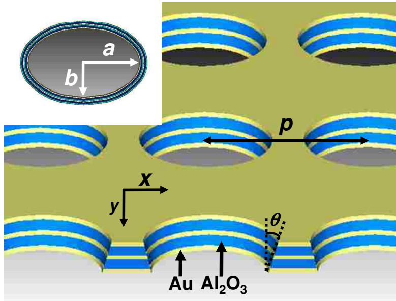
Fig. 4.9 Schematic view of structure and dimensions for two FLMs elliptical NIM: p = 830 nm, 2a = 584 nm, 2b = 361 nm, and \theta (SWA) = 13^\circ . Inset shows magnified elliptical hole with dimension ( a , b ) in major/minor axis.
