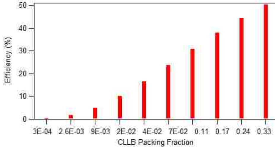
Fig. 19. Efficiency of CLLB component based on {}^6\text{Li}(n,\alpha) reaction rate for different packing fractions.
