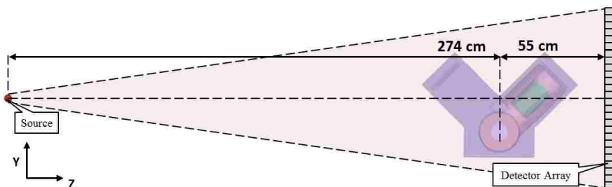
Fig. 51. 2D MCNP model of the imaging scenario
