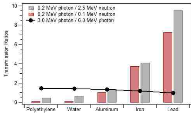
Fig. 1. Transmission ratio comparison for different dual-radiation imaging
