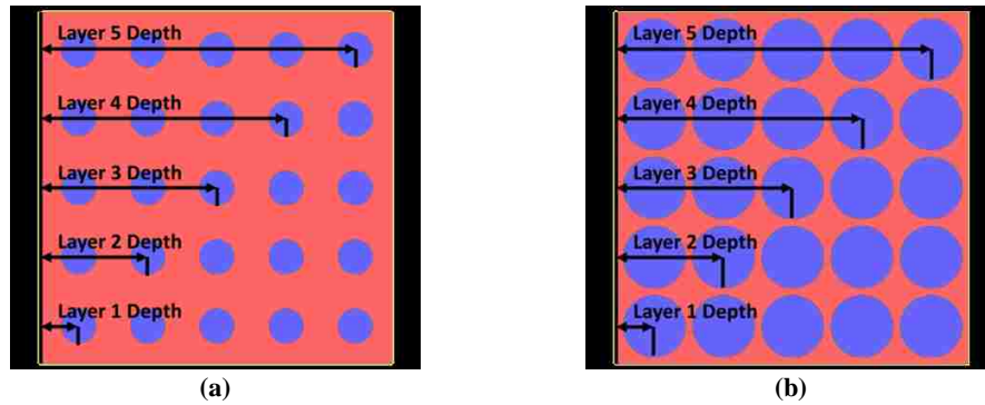
Fig. 17. CLLB layer placement in EJ-299-33A matrix for crystal diameters of (a) 5-mm, (b) 9-mm
