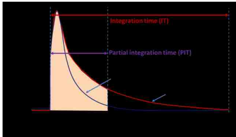
Figure 38 - Pulse Shape Discrimination Scheme Showing Differences in Photon and Neutron Trace Signals [12]
