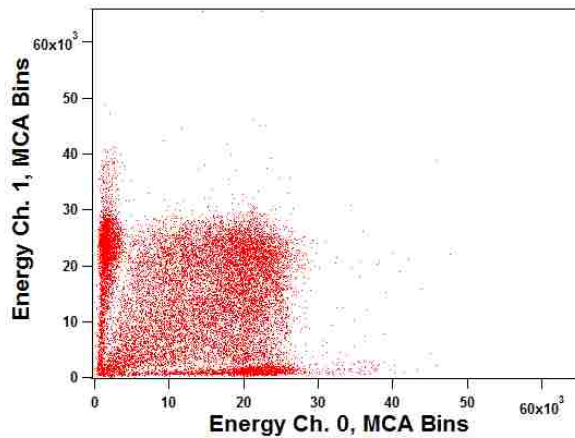
Figure 58 - Energy Coincidence Between Two Channels of qMorpho with Coincidence Window at 1 ADC Clock Cycles
