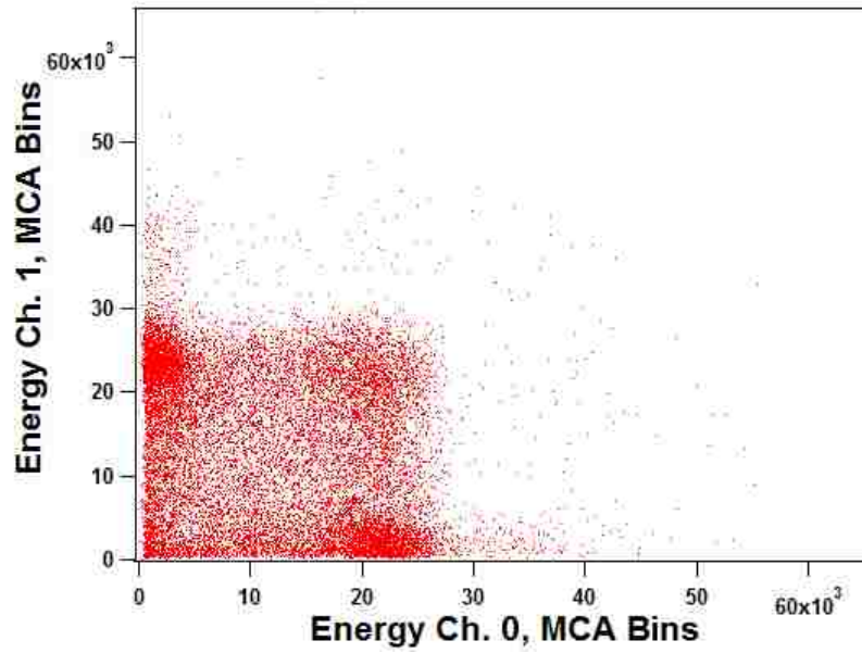
Figure 52 – Energy Coincidence Between Two Channels of qMorpho
