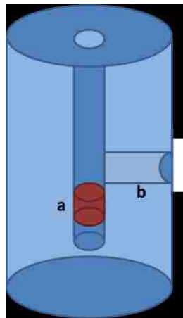
Figure 28 - Pu-Be Source Schematic Showing the (A) Pu-Be Source in the "Closed" Position, and the (B) Neutron Beam Port
