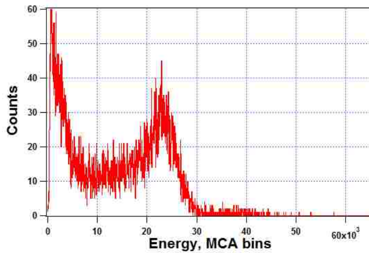
Figure 53 – Energy Spectra of ^{60}\text{Co} on Channel 0
