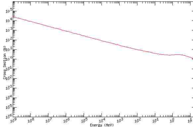
Figure 15 - 3 He Total Absorption Cross-Section Data [22]
