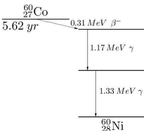
Figure 30 - Decay Scheme of ^{60}\text{Co} [60]
