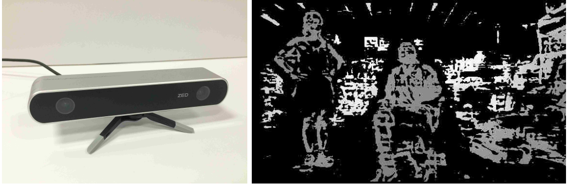
Figure 2.1: (Left) The Stereo Labs Zed stereo camera. (Right) A representative depth image captured by the Zed camera. Distance is colored on a grey to white scale where grey is nearer to the camera. Black pixels indicate that a point correspondence could not be found between the two camera images.
