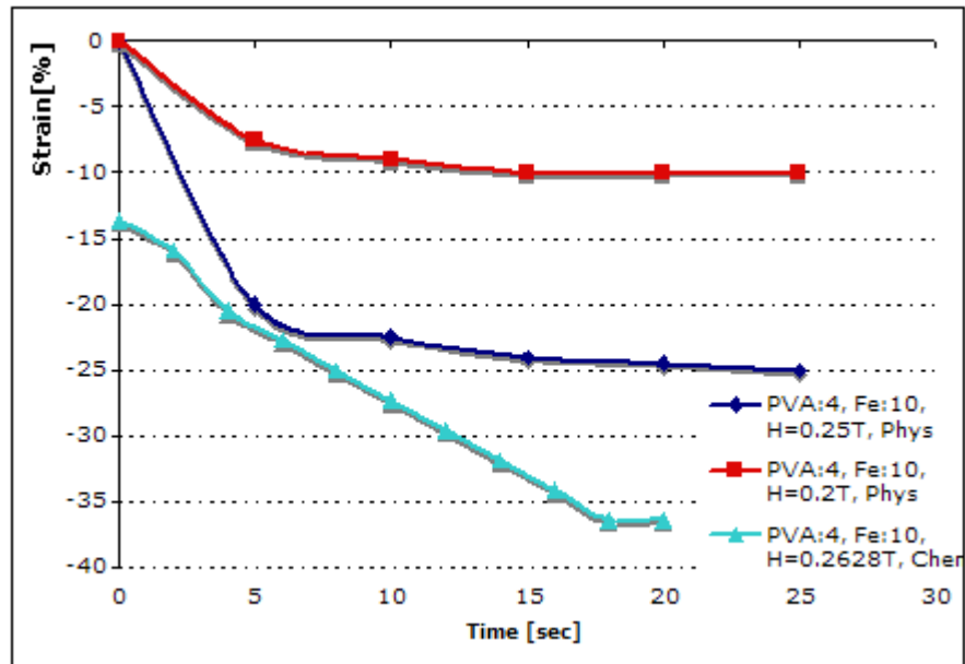
Figure 35: Strain over time for physically and chemically crosslinked samples.
