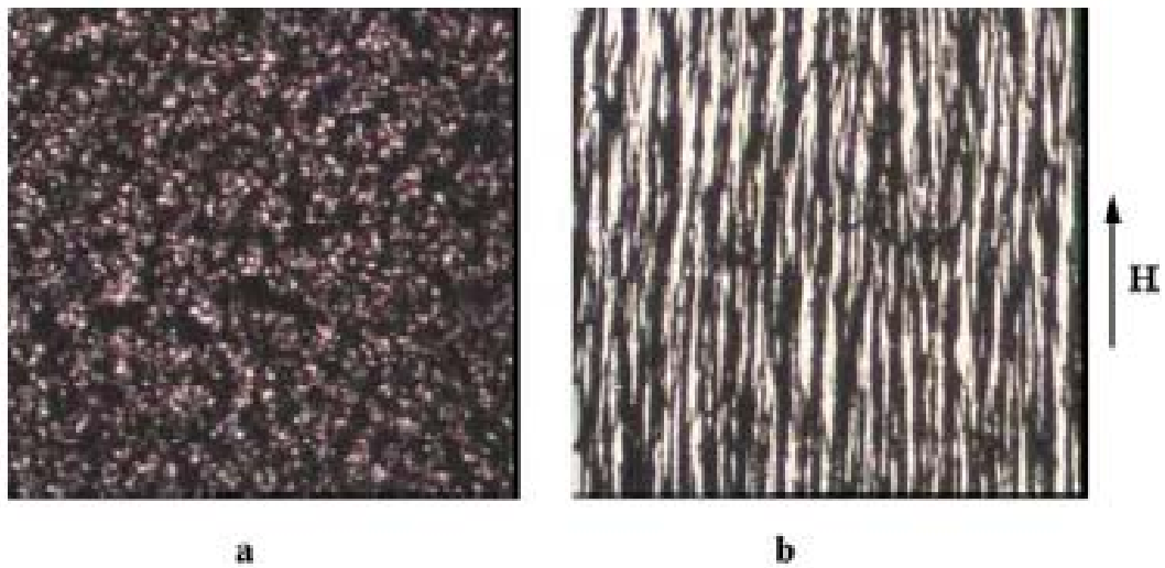
Figure 25. Formation of magnetic particles in silicon oil (5 wt%) [15]. (a) No external magnetic field. (b) The magnetic induction 50 mT.
