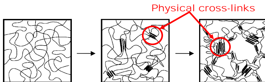
Figure 22. Schematic of physical crosslinking.
