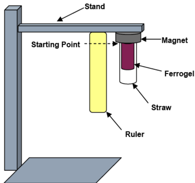
Figure 27. Testing apparatus for free strain.
