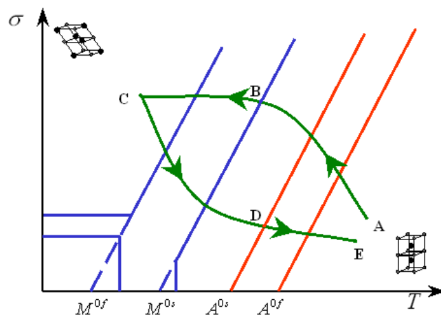
Figure 8. Schematic of a thermo-mechanical loading path demonstrating pseudoelastic behavior of SMAs [8].
