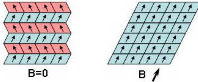
Figure 14. Principle of the Ferromagnetic Shape Memory Effect [5].
