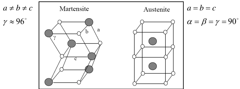
Figure 7. Schematic of Unit cells of NiTi in the martensite and austenite phases [12].
