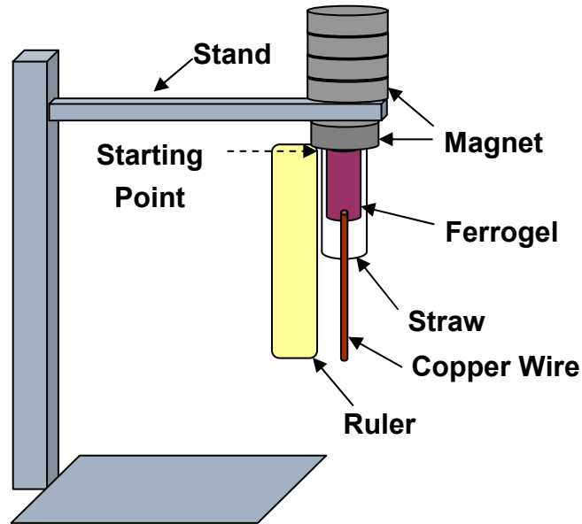
Figure 28. Testing apparatus for loaded tests.
