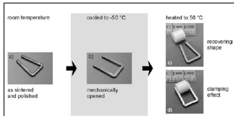
Figure 10. The behavior of the staple during a cooling-heating cycle [16].
