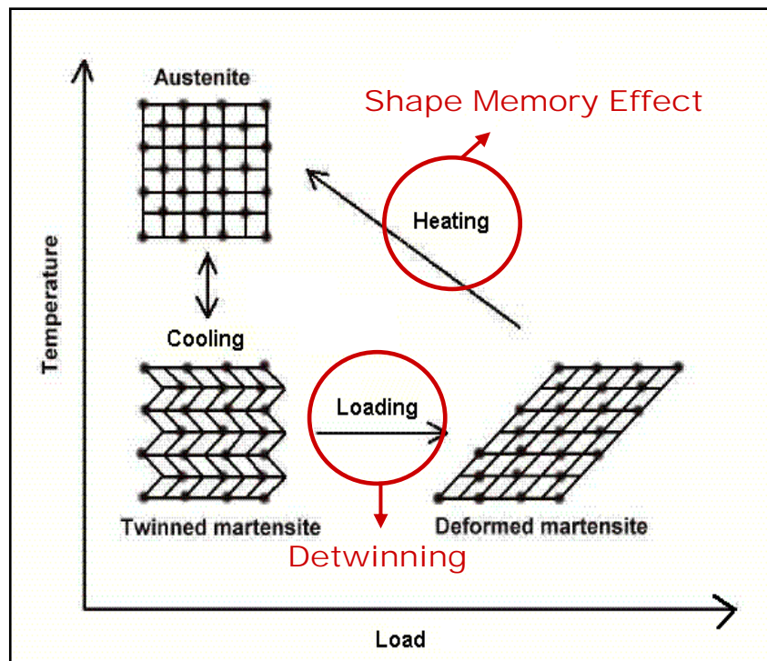
Figure 9. Transformation from the austenite to the martensite phase and shape memory effect [17].
