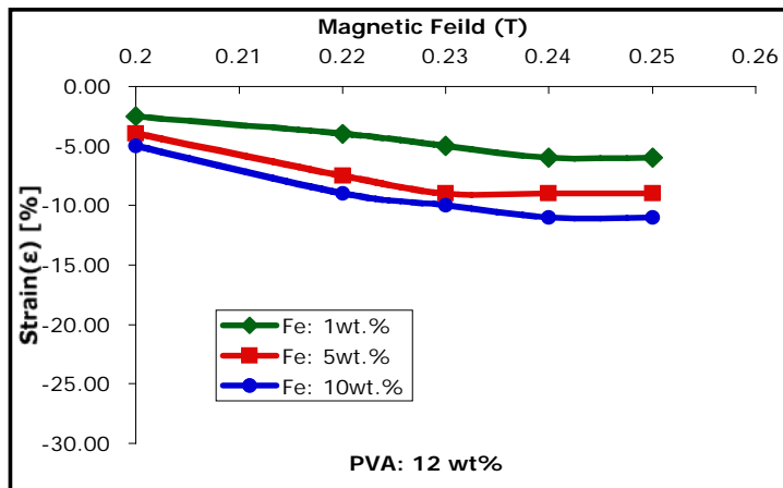
Figure 31. Free strain under field for selected PVA and CIP weight percents.
