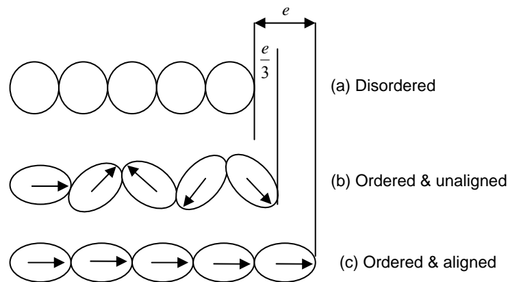
Figure 13. Schematic Diagram of the Magnetostrictive Materials [1].
