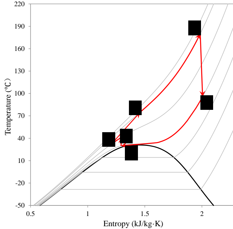
Figure 3–24 T - s diagram of s\text{CO}_2 Brayton cycle with pre-compression and inter-cooling.
