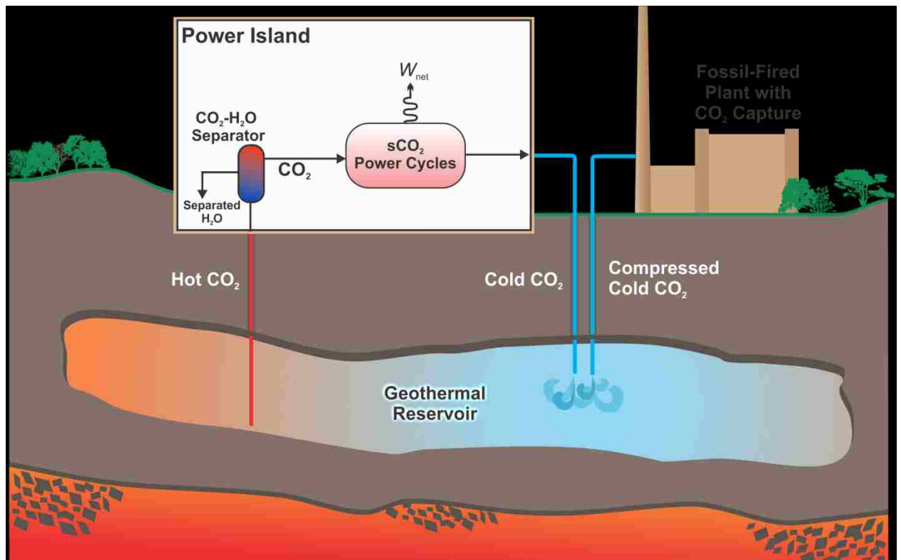
Figure 3–1 Sketch of CO 2 direct expansion approach using hot produced CO 2 from geothermal reservoir.
