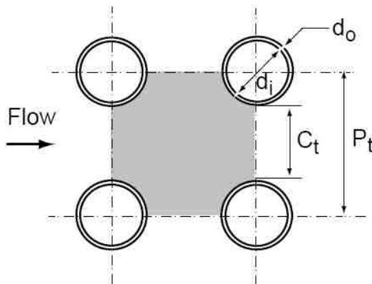
Figure A-4 Square-pitch layout and the equivalent diameter equation.
