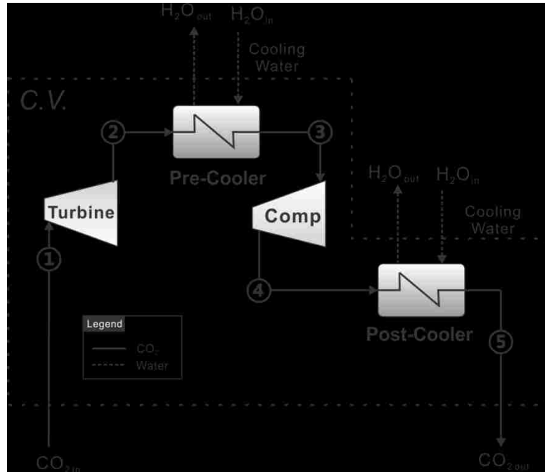
Figure 3–8 Control volume for direct expansion performance evaluation.
