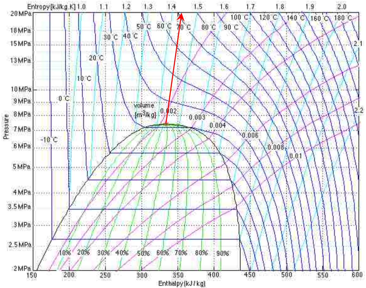
Figure 3–5 P-h diagram of CO 2 .
