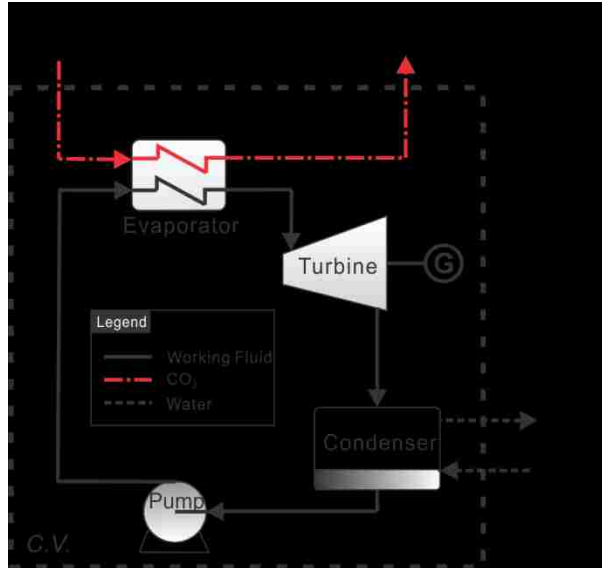
Figure 4–3 Control volume for ORC exergy and thermal efficiency calculation.
