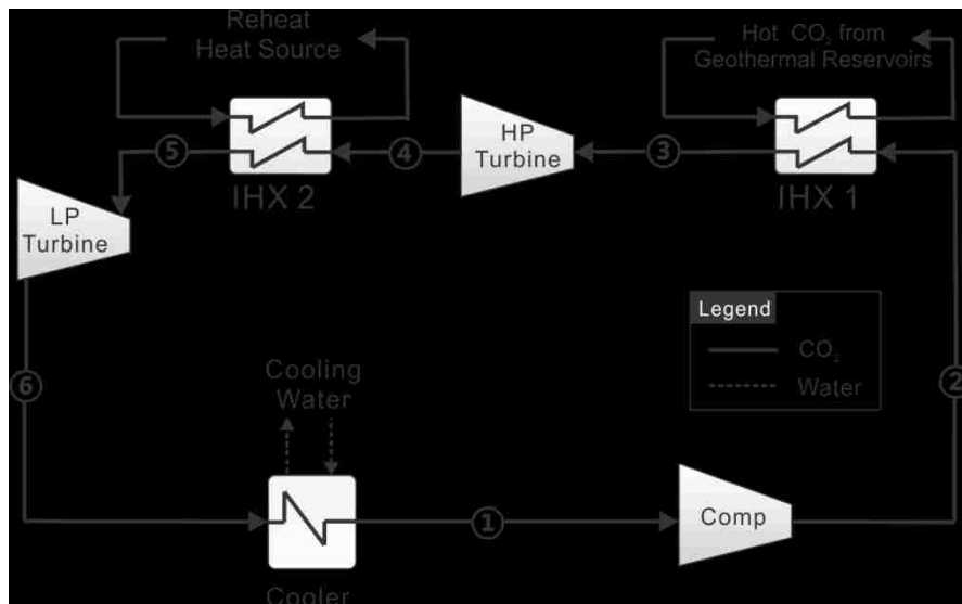
Figure 3–29 Schematic of sCO 2 Brayton cycle with reheat.
