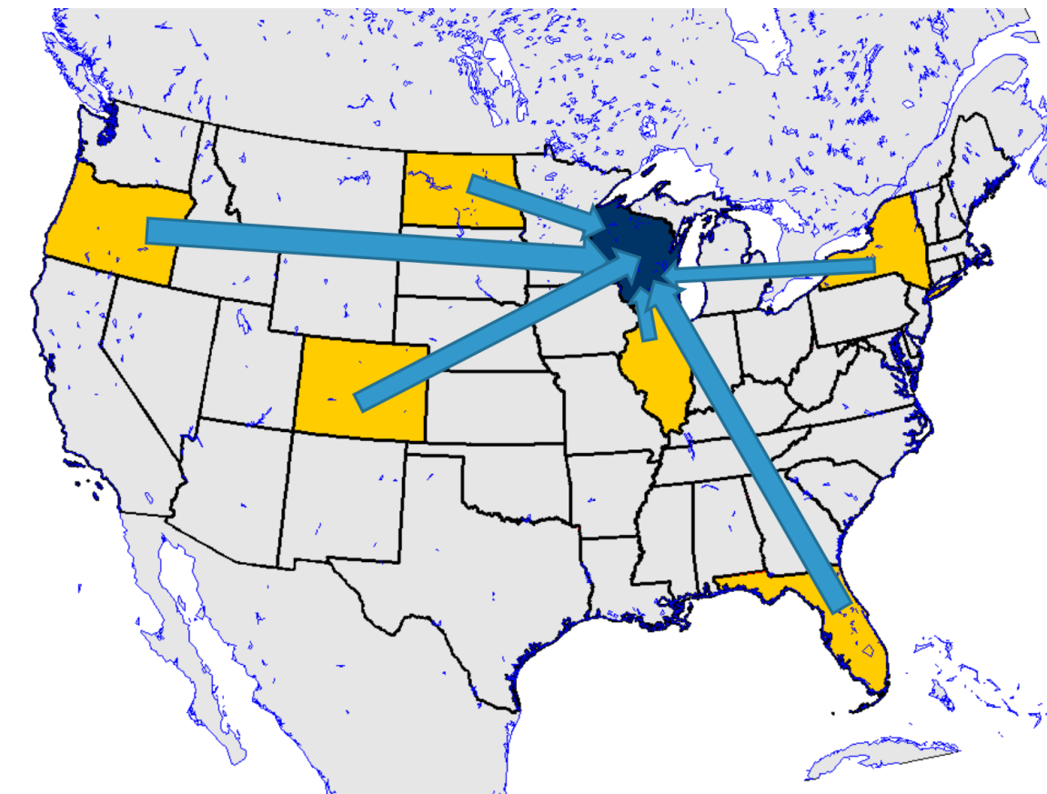
Figure 1.1: Data from different states may be used as surrogate data for the state of Wisconsin.
