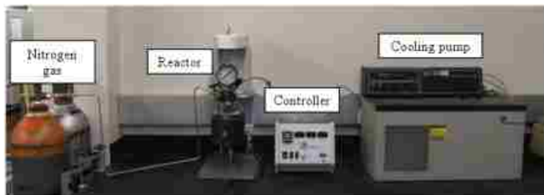
Figure 3.6: Specimen curing set-up to simulate elevated temperature and pressure
