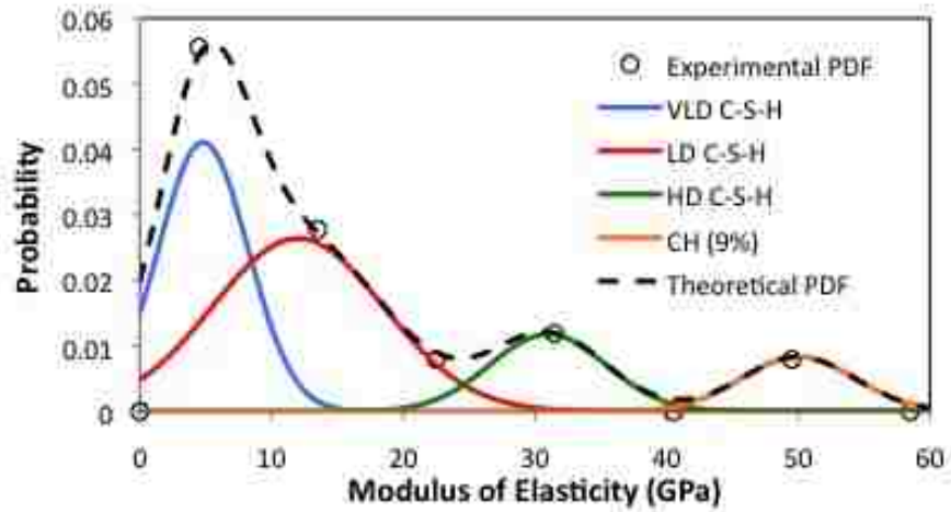
Figure 4.27: Deconvolution of 0.9 C/S C-S-H compacted to 150 MPa
