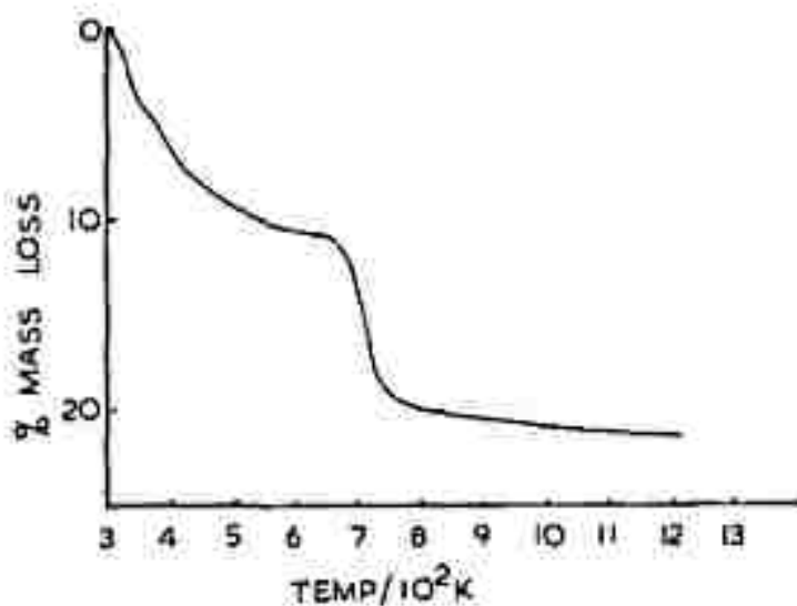
Figure 2.2: Typical TGA curve for Ordinary Portland Cement as published by Earnest [22].
