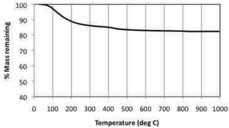
Figure 4.20: Thermogravimetric Analysis of 0.9 C/S C-S-H
