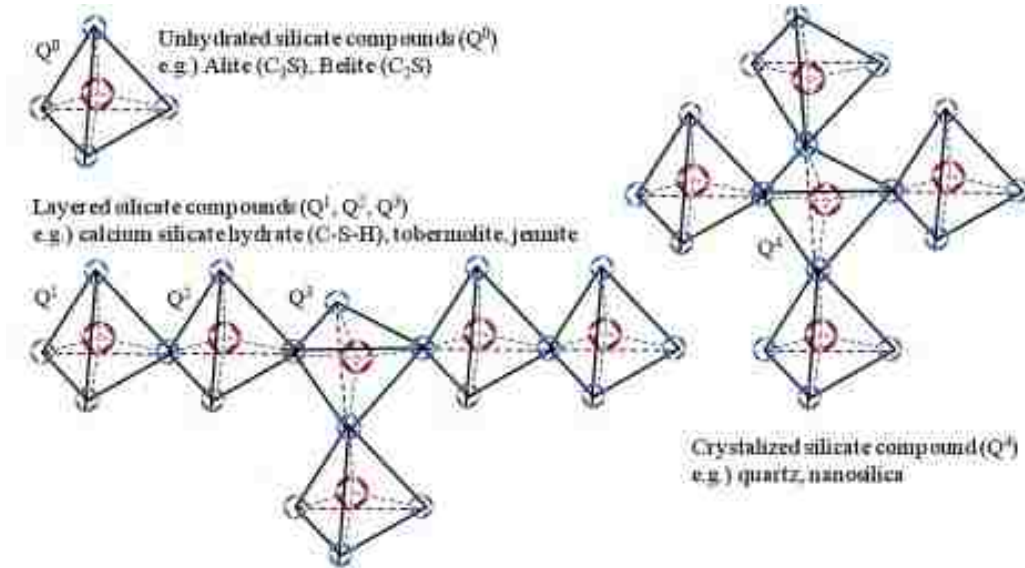
Figure 3.15: Various silicate compounds detectable by 29 Si NMR
