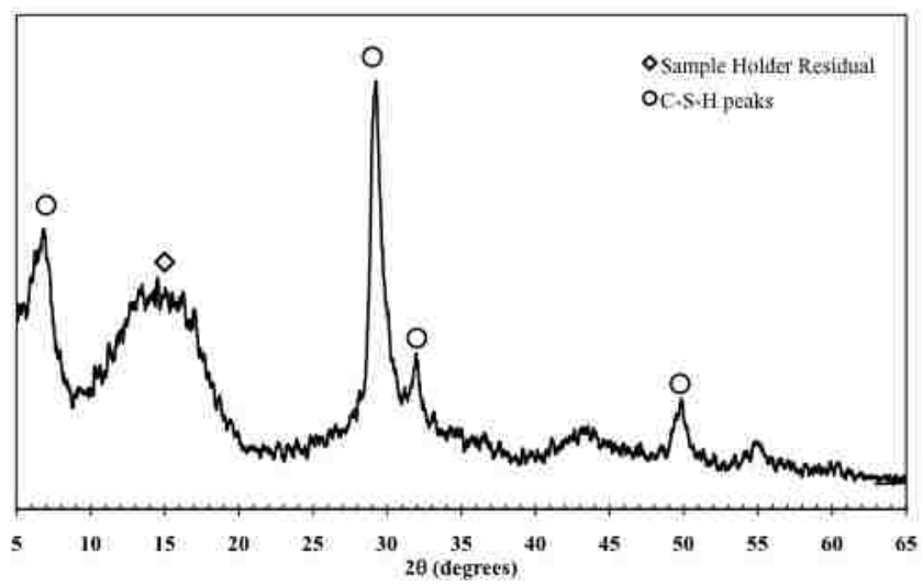
Figure 4.16: XRDA Plot of 0.9 C/S C-S-H.
