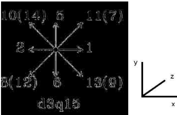
Figure 2 D3Q15 lattice arrangement. The directions in parenthesis are angled out of the paper. The directions on the diagonals not in parenthesis are angled into the paper. Not shown here is direction zero which is the node itself, direction 3 that is normal to the page facing out, and direction 4 that is normal to the page facing in.
