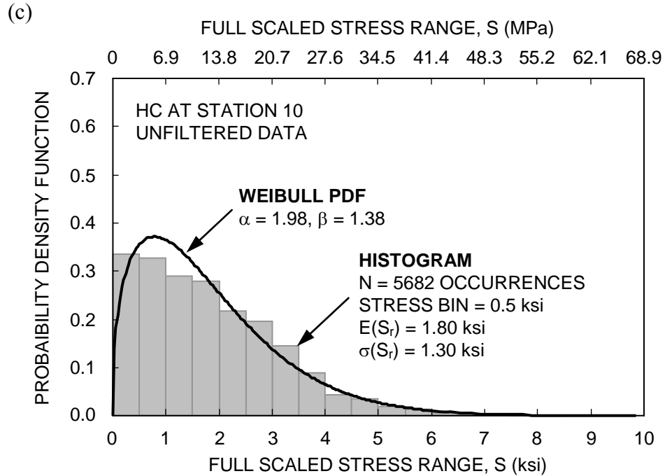
(c) unfiltered data at Station 10, 15 knots, HC and heading of 0°
