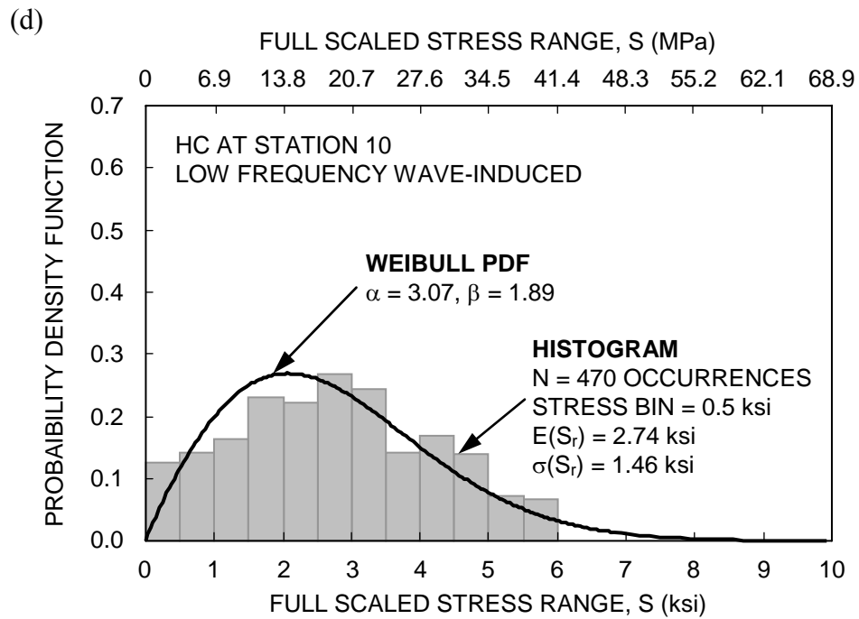
(d) low frequency wave-induced data at Station 10, 15 knots, HC and heading of 0°
