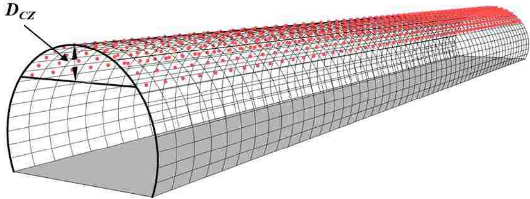
Figure 7 – Depth of convective zone under tunnel ceiling
