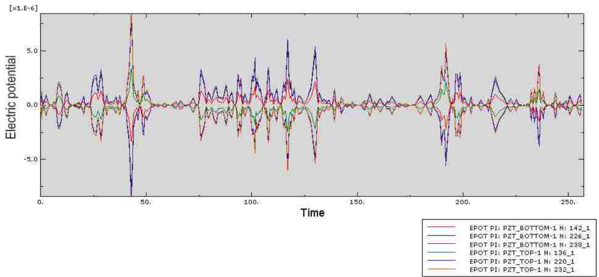
Figure 46: Time-history of electrical potential EPOT for the dynamic load beam model - six nodes
