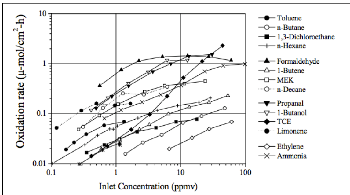
Figure 3.2.2: Measured PCO Reaction Rates for VOCs of Interest in Indoor Air.
