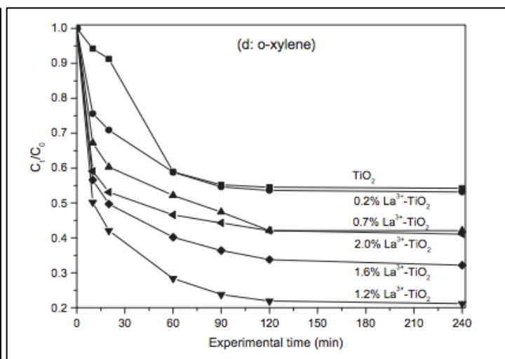
Figure 3.3.2: PCO Degradation of o -xylene
