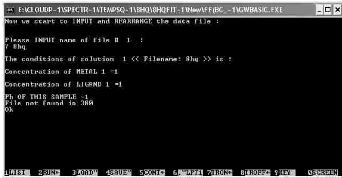
Figure A1.8- Screen shot showing the result of entering an input file name that does not exist in the folder that contains the "SQUAD-IN.BAS" program that is running.
