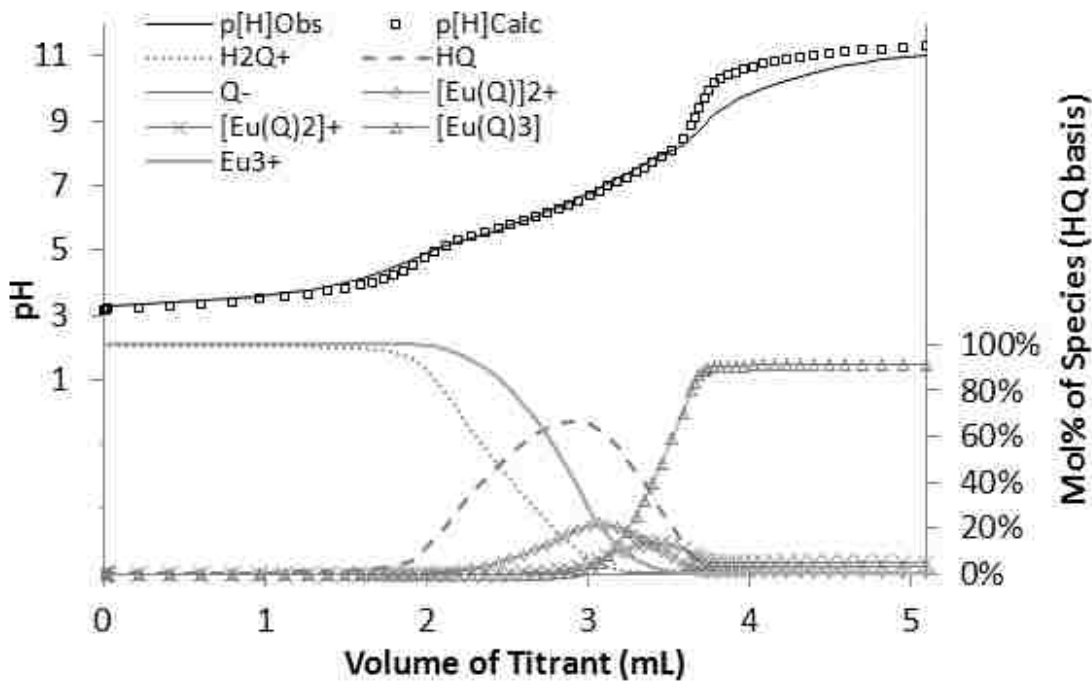
Figure 3.17- Hyperquad fit results for titration of [HQ] = 3 \times 10^{-4} M, [Eu^{3+}] = 1 \times 10^{-4} M, [NaCl] = 0.1 M, [HCl] = 0.001 M by [NaOH] = 0.01024 \pm 0.00002 M and [NaCl] = 0.09 M. T = 2.0 \pm 0.2 °C.
