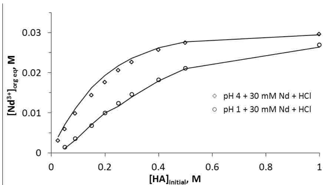
Figure 2.6- Calculated by SXLSQL (line) and observed (symbols) organic \text{Nd}^{3+} concentration as a function of initial HA molarity.
