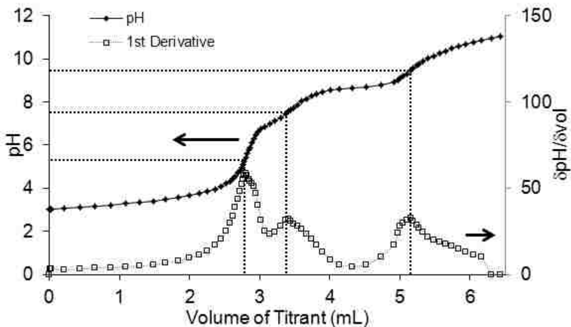
Figure 3.32- Titration of [Eu^{3+}] = 3 \times 10^{-4} M, [NaCl] = 0.1 M, [HCl] = 0.001 M, [Triton\ X-114] = 1 wt% ( \sim 0.02 M), by [NaOH] = 0.01024 \pm 0.00002 M and [NaCl] = 0.09 M. T = 1.8 \pm 0.2 °C.
