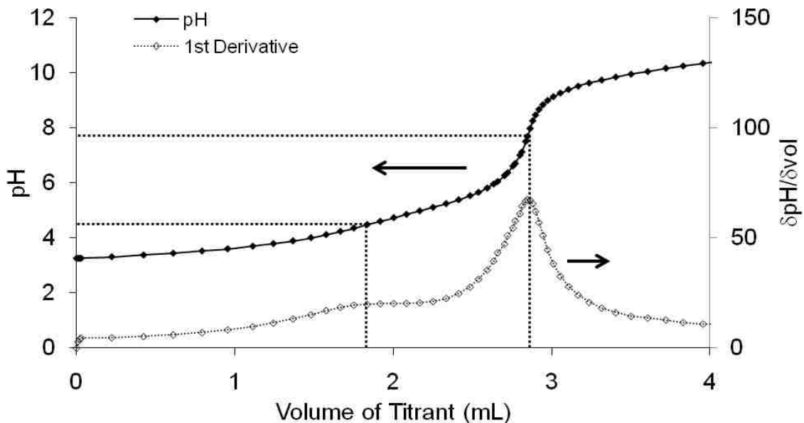
Figure 3.23- Titration of [HQ] = 3 \times 10^{-4} M, [NaCl] = 0.1 M, [HCl] = 0.001 M, [Triton\ X-114] = 1 wt% ( \sim 0.02 M) by [NaOH] = 0.01024 \pm 0.00002 M and [NaCl] = 0.09 M. T = 1.8 \pm 0.2 °C.
