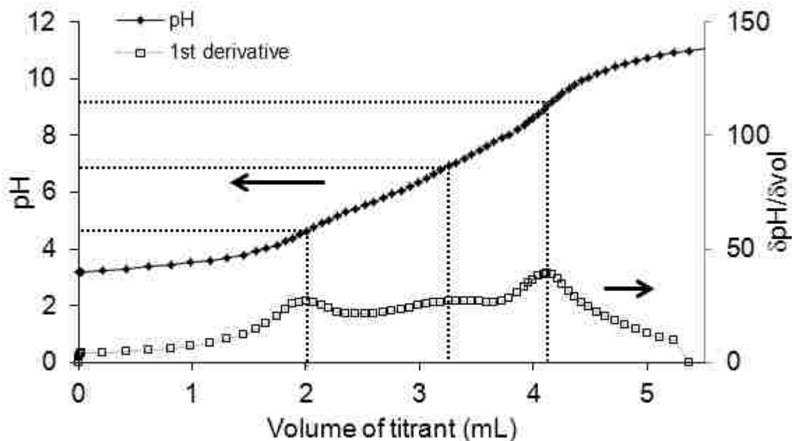
Figure 3.14- Titration of [HQ] = 3 \times 10^{-4} \text{ M} , [Eu^{3+}] = 1.5 \times 10^{-4} \text{ M} , [NaCl] = 0.1 \text{ M} , [HCl] = 0.001 \text{ M} by [NaOH] = 0.01024 \pm 0.00002 \text{ M} and [NaCl] = 0.09 \text{ M} . T = 1.9 \pm 0.2 \text{ } ^\circ\text{C} .
