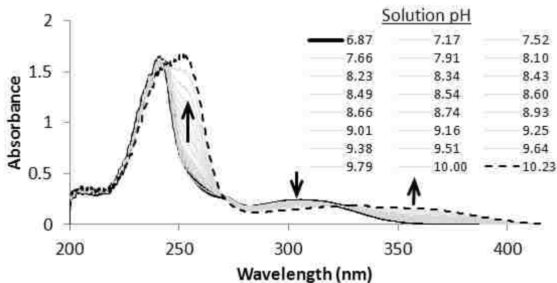
Figure 3.7- Spectral changes for [HQ] = 10^{-5} \text{ M} , [\text{NaCl}] = 0.1 \text{ M} , [\text{HCl}] = 0.001 \text{ M} titrated by NaOH of varying concentration and volume at 1.8 \pm 0.2 \text{ }^\circ\text{C} . The solution pH for each spectrum is listed in the figure legend. Arrows indicate the direction of the spectral change as pH increases. These spectral changes represent the transition from 8-hydroxyquinoline protonation state B to C in Figure 3.2.
