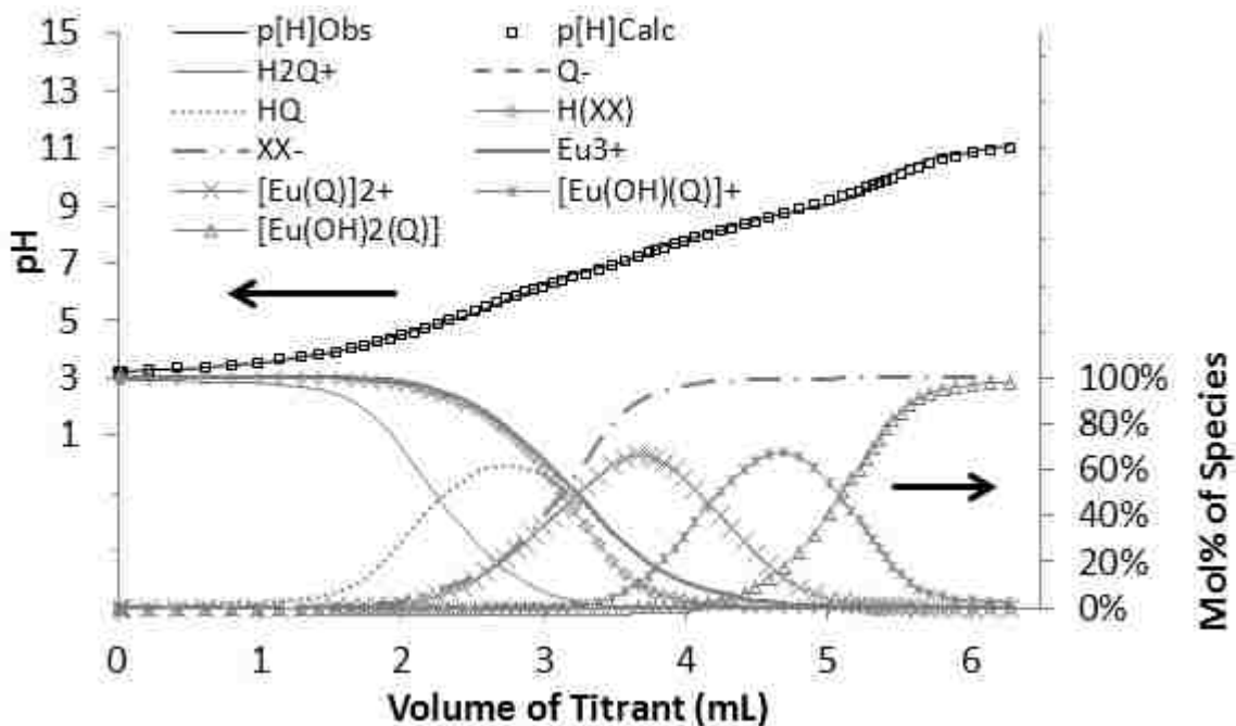
Figure 3.35- Hyperquad fit for the titration of [HQ] = 3 \times 10^{-4} \text{ M} , [Eu^{3+}] = 3 \times 10^{-4} \text{ M} , [NaCl] = 0.1 \text{ M} , [HCl] = 0.001 \text{ M} , [Triton \text{ X-114}] = 1 \text{ wt\% } (\sim 0.02 \text{ M}) , by [NaOH] = 0.01024 \pm 0.00002 \text{ M} and [NaCl] = 0.09 \text{ M} . T = 1.8 \pm 0.2 \text{ } ^\circ\text{C} .
