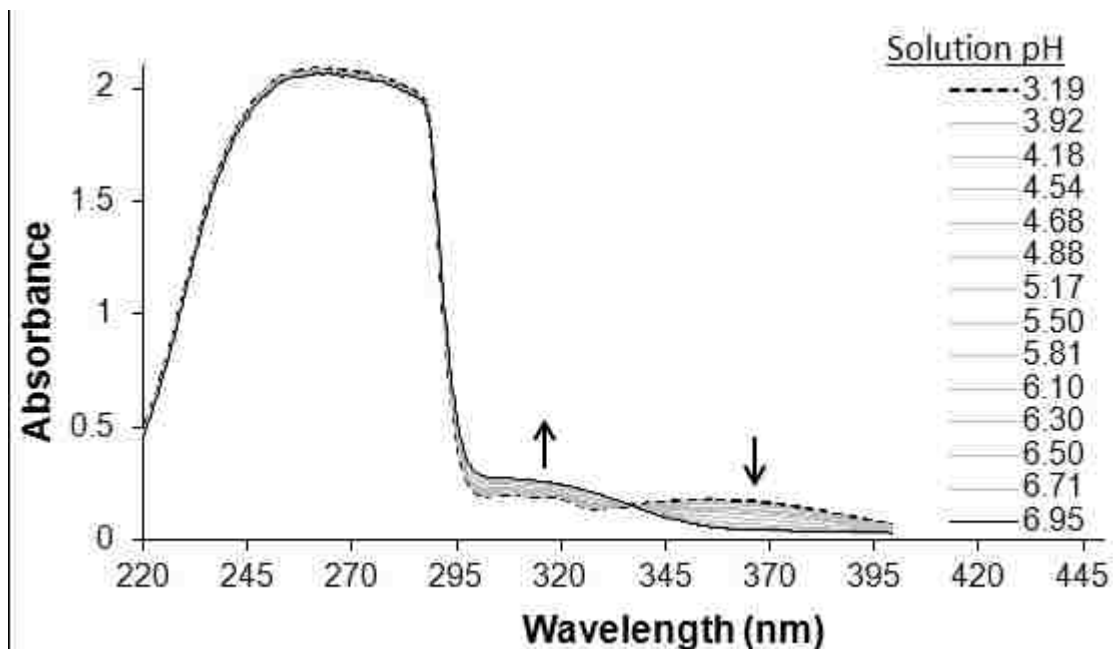
Figure 3.26-Spectra obtained while titrating a solution containing: [HQ] = 0.0001\text{ M} , [NaCl] = 0.1\text{ M} , [Triton\ X-114] = 1\text{ wt\%} . Spectra shown are of pH 3.19–6.95. The arrows indicate the spectral change as pH increases.
