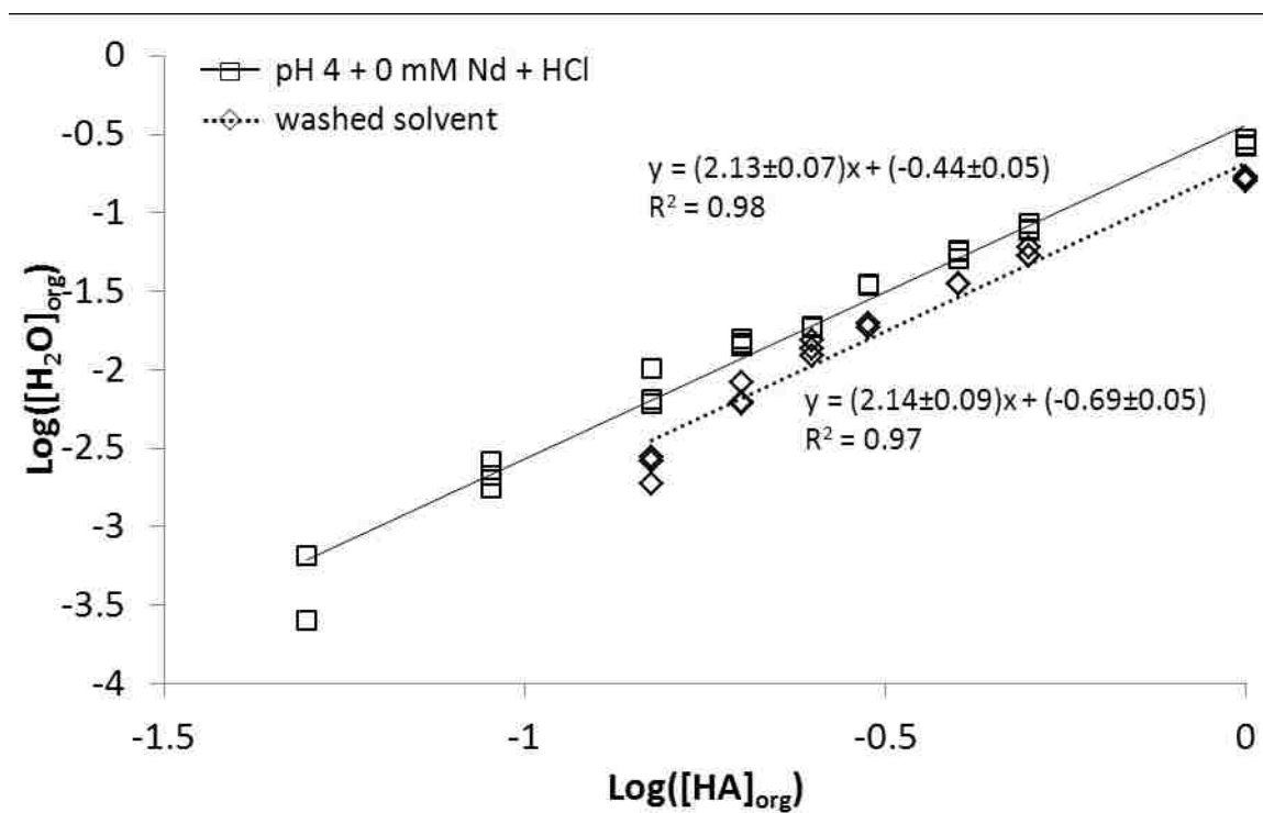
Figure 2.8- Log-slope analysis of water in the washed solvent and the pH 4 + 0 mM Nd + HCl system. The matching slopes indicate that no water was co-extracted with \text{Na}^+ in the pH 4 + 0 mM Nd + HCl system.
