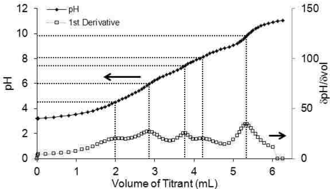
Figure 3.34- Titration of [HQ] = 3 \times 10^{-4} \text{ M} , [Eu^{3+}] = 3 \times 10^{-4} \text{ M} , [NaCl] = 0.1 \text{ M} , [HCl] = 0.001 \text{ M} , [Triton \text{ X-114}] = 1 \text{ wt\% } (\sim 0.02 \text{ M}) , by [NaOH] = 0.01024 \pm 0.00002 \text{ M} and [NaCl] = 0.09 \text{ M} . T = 1.8 \pm 0.2 \text{ } ^\circ\text{C} .
