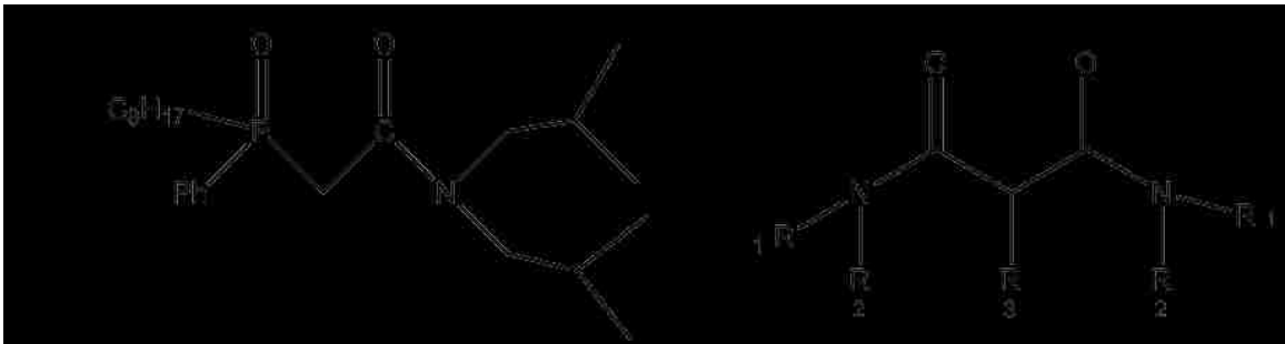
Figure 1.5- Examples of extractants developed for the trivalent actinide/trivalent lanthanide co-extraction: A) octyl (phenyl)-N,N-diisobutylcarbamoyl-methylphosphine oxide; B) generic form of the diamide extractant.
