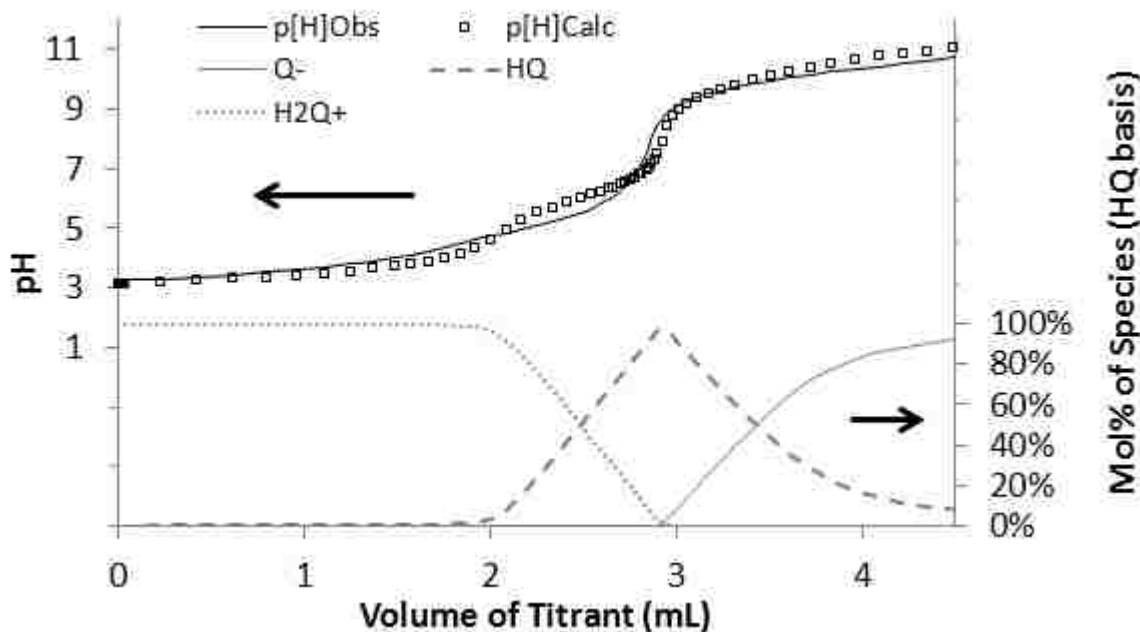
Figure 3.24- Hyperquad fit for the titration of [HQ] = 3 \times 10^{-4} \text{ M} , [NaCl] = 0.1 \text{ M} , [HCl] = 0.001 \text{ M} , [Triton \text{ X-114}] = 1 \text{ wt\%} (\sim 0.02 \text{ M}) by [NaOH] = 0.01024 \pm 0.00002 \text{ M} and [NaCl] = 0.09 \text{ M} . T = 1.8 \pm 0.2 \text{ } ^\circ\text{C} .
