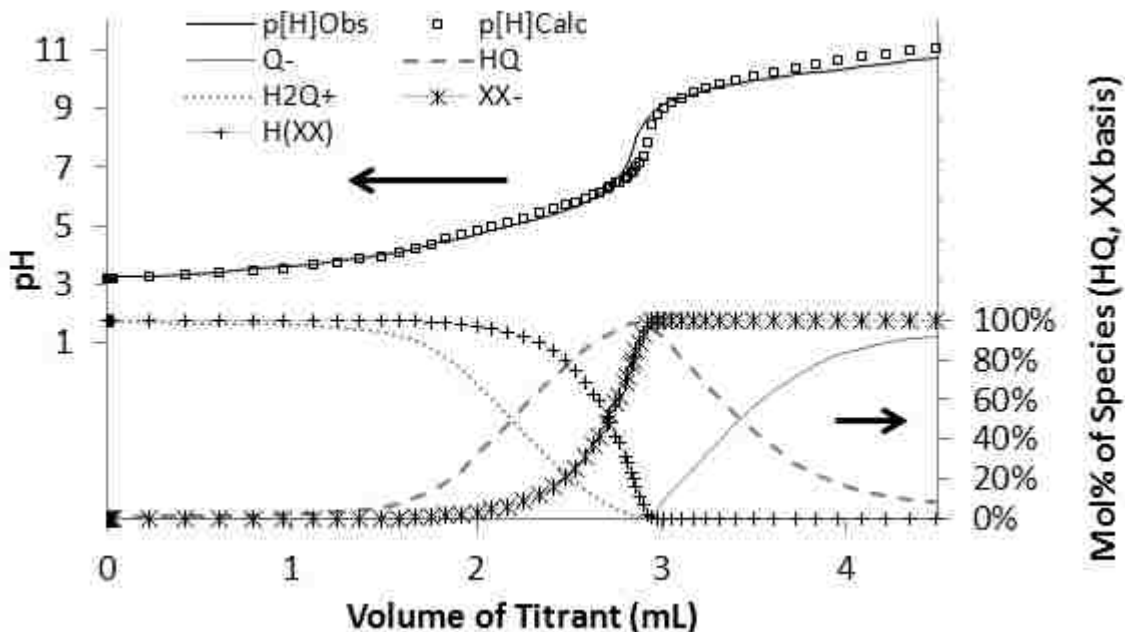
Figure 3.25- Hyperquad fit for the titration of [HQ] = 3x10 -4 M, [NaCl] = 0.1 M, [HCl] = 0.001 M, [Triton X-114] = 1 wt% (~0.02 M), by [NaOH] = 0.01024 ± 0.00002 M and [NaCl] = 0.09 M. T = 1.8±0.2 °C.
