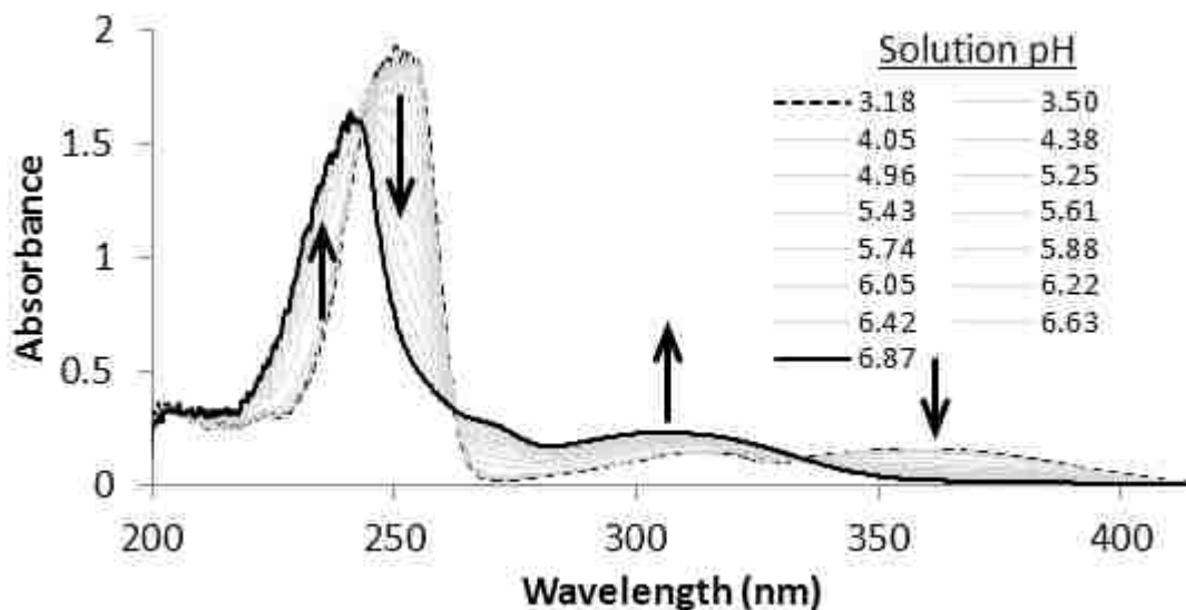
Figure 3.6-Spectral changes for [HQ] = 10^{-5} M , [NaCl] = 0.1 M , [HCl] = 0.001 M titrated by NaOH of varying concentration and volume at 1.8 \pm 0.2 ^\circ C . The solution pH for each spectrum is listed in the figure legend. Arrows indicate the direction of the spectral change as pH increases. These spectral changes represent the transition from 8-hydroxyquinoline protonation state A to B in Figure 3.2.
