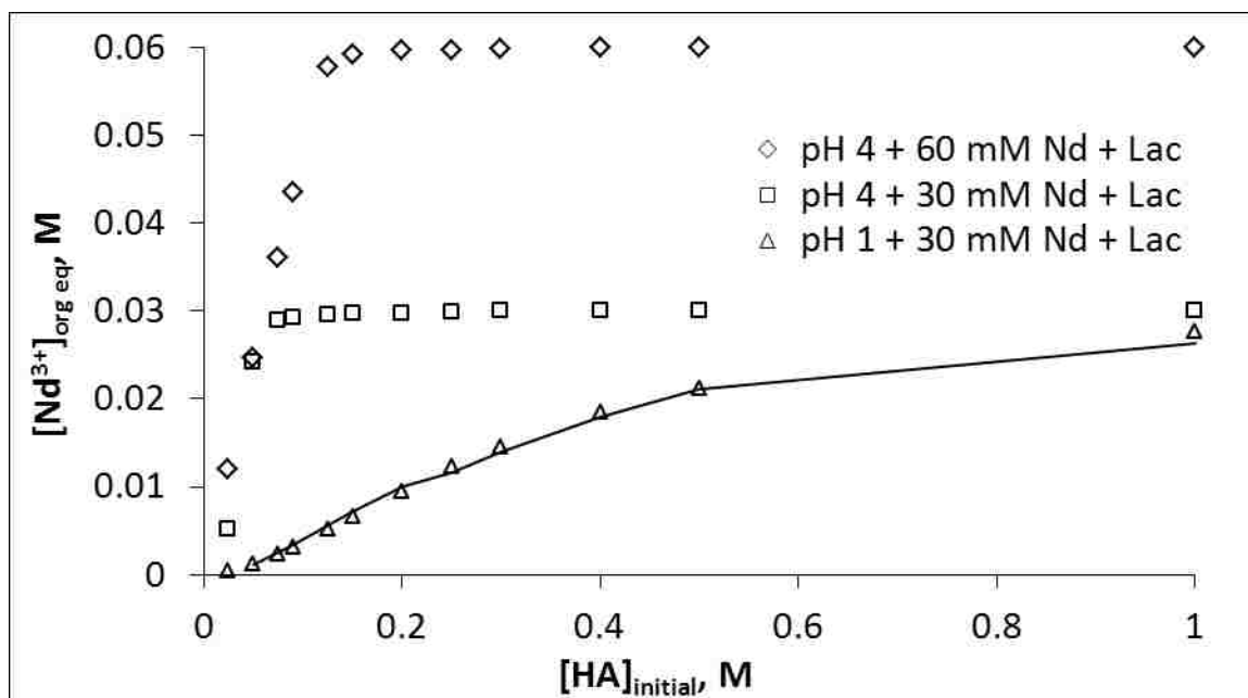
Figure 2.15- \text{Nd}^{3+} extraction results. Observed data are depicted as points, SXLSQL modeling results are depicted as the solid curve.
