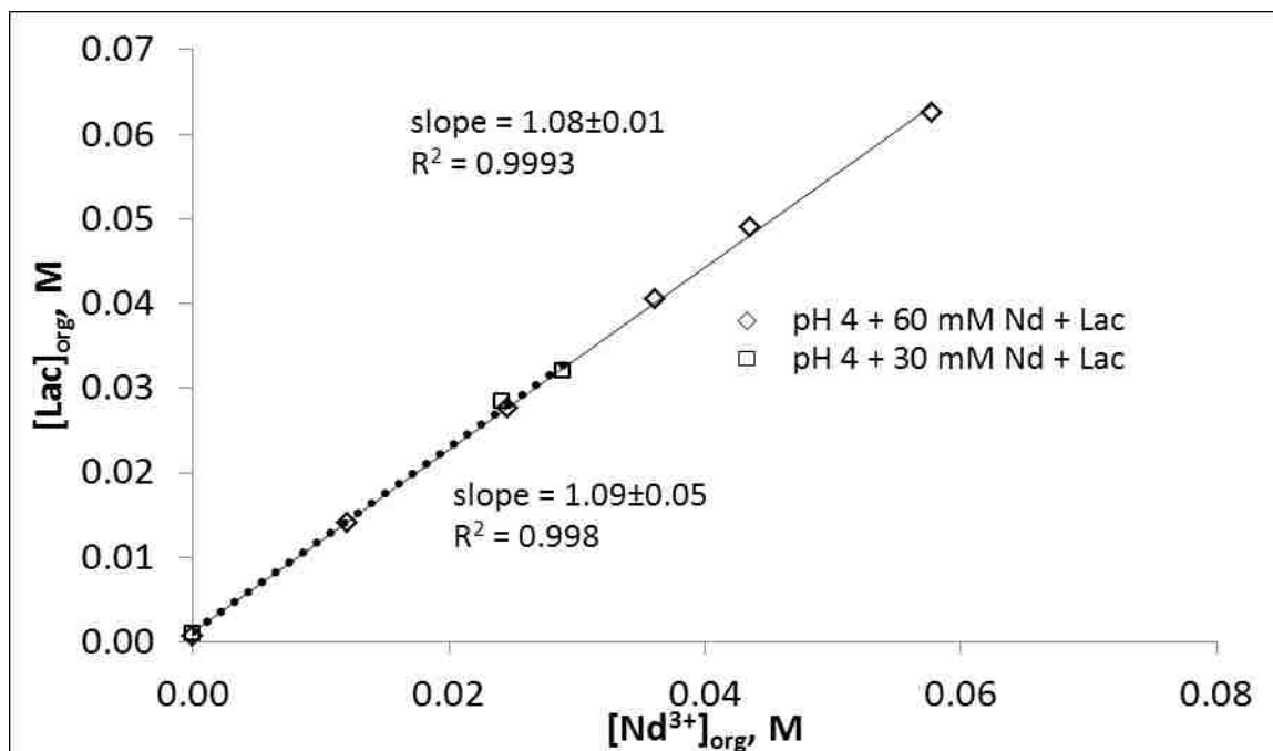
Figure 2.21- Linear scale dependence of the extraction of Lac and \text{Nd}^{3+} in the pH 4 + (30, 60) mM Nd + Lac systems. This data is limited to the data points where the \text{Nd}(\text{Lac})(\text{HA})_2 species was shown to be present.
