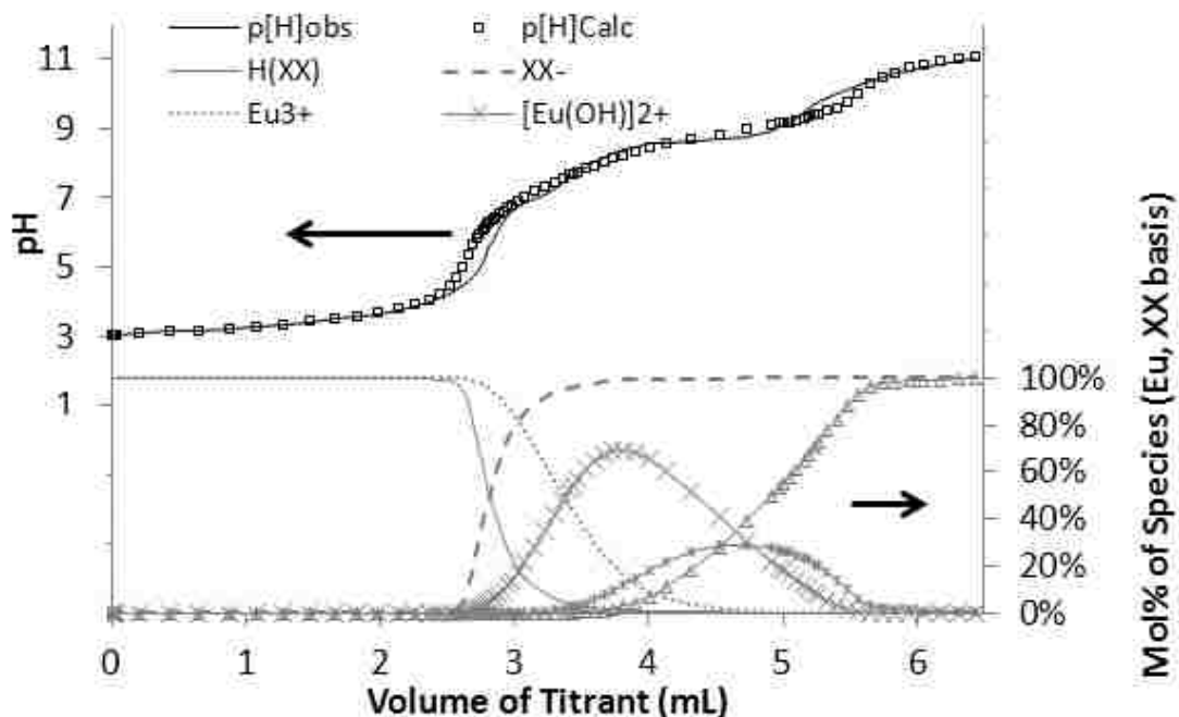
Figure 3.33- Hyperquad fit for the titration of [Eu^{3+}] = 3 \times 10^{-4} M, [NaCl] = 0.1 M, [HCl] = 0.001 M, [Triton\ X-114] = 1 wt% ( \sim 0.02 M), by [NaOH] = 0.01024 \pm 0.00002 M and [NaCl] = 0.09 M. T = 1.8 \pm 0.2 °C.
