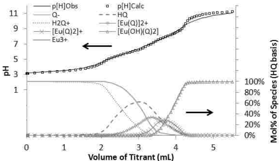
Figure 3.15- Hyperquad fit results for titration of [HQ] = 3 \times 10^{-4} \text{ M} , [Eu^{3+}] = 1.5 \times 10^{-4} \text{ M} , [NaCl] = 0.1 \text{ M} , [HCl] = 0.001 \text{ M} by [NaOH] = 0.01024 \pm 0.00002 \text{ M} and [NaCl] = 0.09 \text{ M} . T = 1.7 \pm 0.2 \text{ } ^\circ\text{C} .
