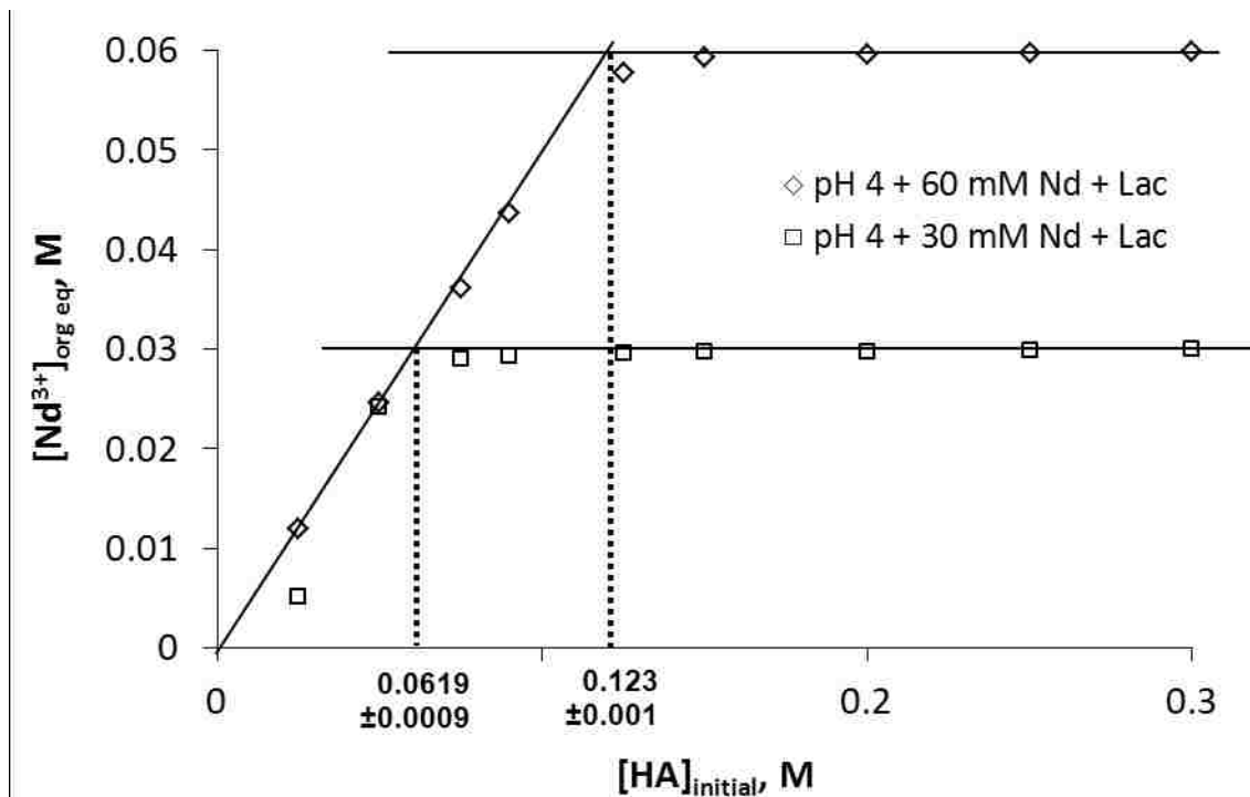
Figure 2.16- The transition between saturation and quantitative extraction supports the 1:2 \text{Nd}^{3+} : HA stoichiometry of the \text{NdLacA}_2 complex.
