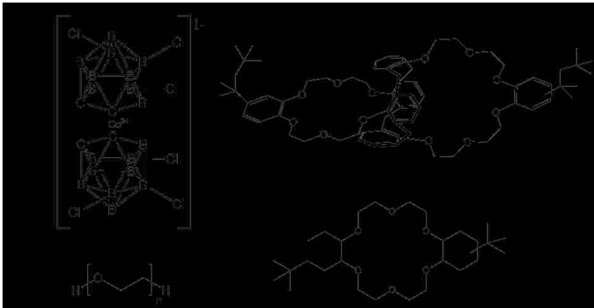
Figure 1.3- Extractants used in cesium and strontium extraction: A) Chlorinated Cobalt Dicarbollide; B) Polyethylene Glycol; C) Calix[4]arene-bis(4-tert-octylbenzo-crown-6); D) bis [4,4'(5')-(tert-butyl)cyclohexano]-18-crown-6.
