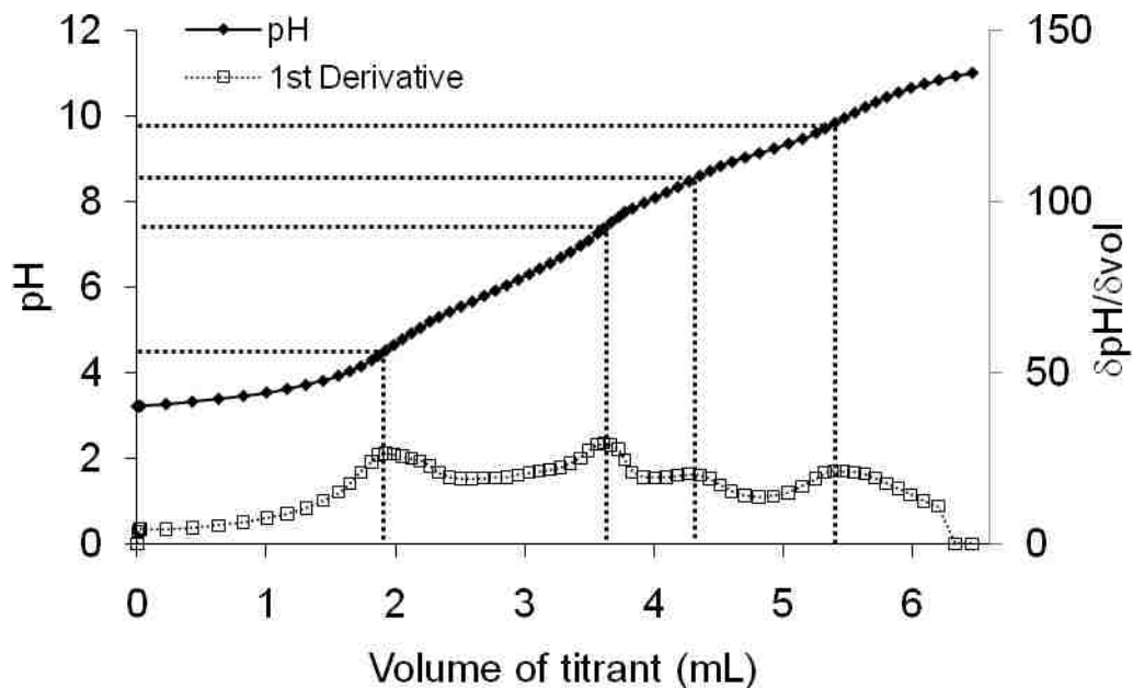
Figure 3.12- Titration of [HQ] = 3 \times 10^{-4} \text{ M} , [Eu^{3+}] = 3 \times 10^{-4} \text{ M} , [NaCl] = 0.1 \text{ M} , [HCl] = 0.001 \text{ M} by [NaOH] = 0.01024 \pm 0.00002 \text{ M} and [NaCl] = 0.09 \text{ M} . T = 1.7 \pm 0.2 \text{ } ^\circ\text{C} .
