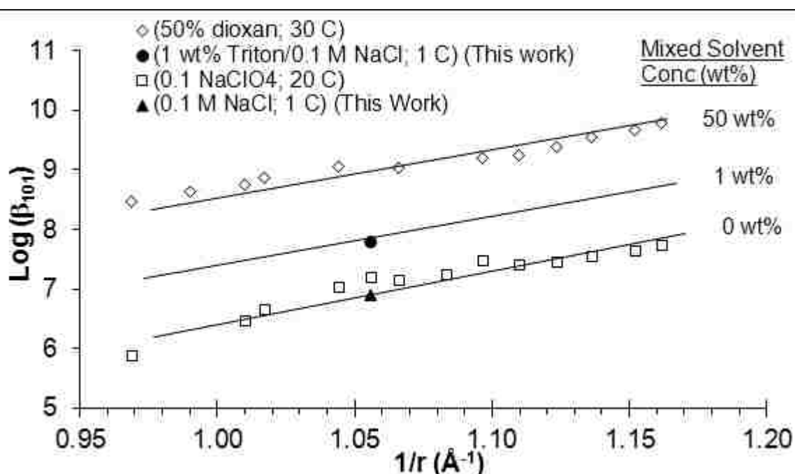
Figure 3.46- Comparison of Literature data for the formation of [\text{Eu}(\text{Q})]^{2+} in 50% dioxane (at T=30^\circ\text{C} ), and 0% dioxane (at T=20^\circ\text{C} ) with the observed values at 1 wt% Triton X-114 (at 1^\circ\text{C} ) and 0 wt% Triton X-114 (at 1^\circ\text{C} ).
