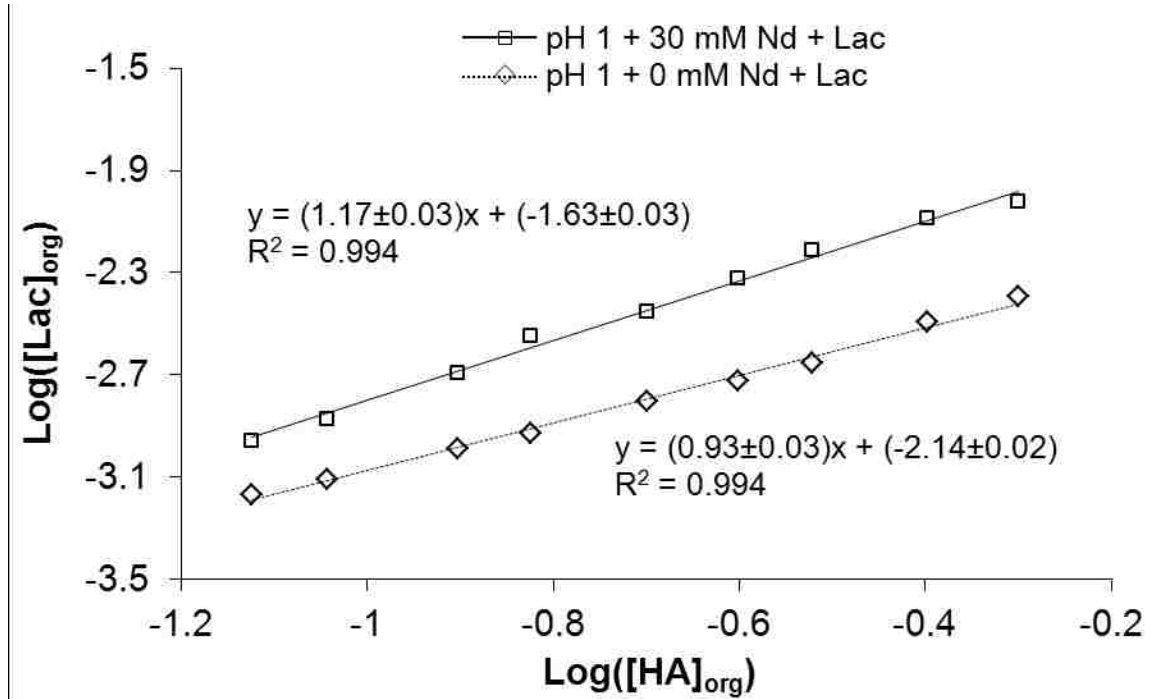
Figure 2.17- Log-slope analysis of Lac extraction vs. [\text{HA}]_{\text{org}} for the pH 1 + (0, 30) mM Nd + Lac systems.
