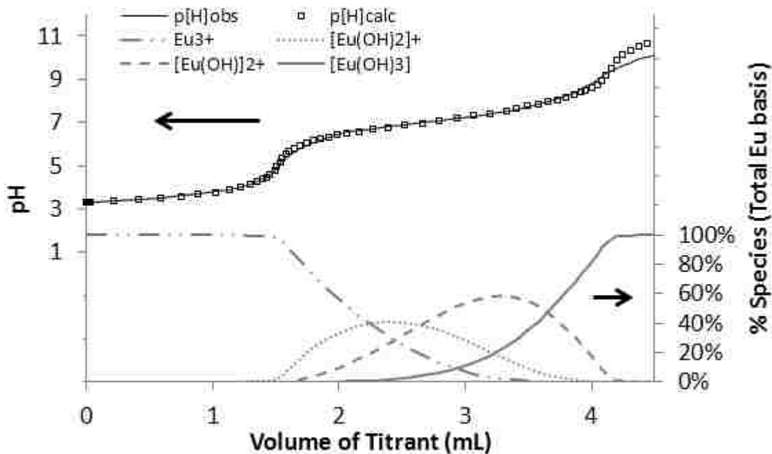
Figure 3.11- Hyperquad modeling results for the titration of [Eu^{3+}] = 3 \times 10^{-4} M, [NaCl] = 0.1 M, [HCl] = 0.001 M by [NaOH] 0.01024 \pm 0.00002 M and [NaCl] = 0.09 M. T = 1.7 \pm 0.2 °C.
