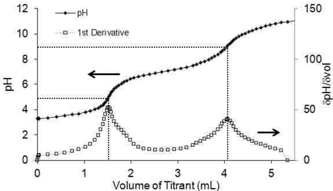
Figure 3.10- Titration of [Eu^{3+}] = 3 \times 10^{-4} M, [NaCl] = 0.1 M, [HCl] = 0.001 M by [NaOH] 0.01024 \pm 0.00002 M and [NaCl] = 0.09 M. T = 1.7 \pm 0.2 °C.
