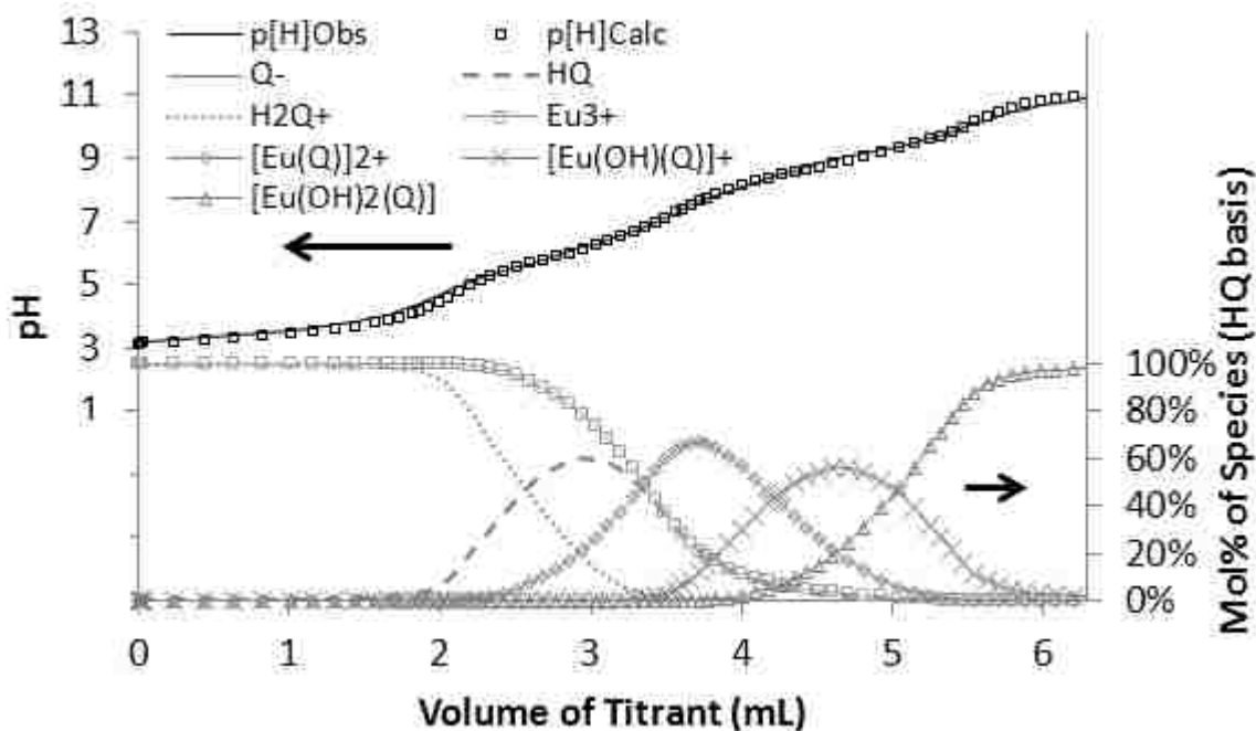
Figure 3.13- Hyperquad fit results for titration of [HQ] = 3 \times 10^{-4} \text{ M} , [Eu^{3+}] = 3 \times 10^{-4} \text{ M} , [NaCl] = 0.1 \text{ M} , [HCl] = 0.001 \text{ M} by [NaOH] = 0.01024 \pm 0.00002 \text{ M} and [NaCl] = 0.09 \text{ M} . T = 1.7 \pm 0.2 \text{ } ^\circ\text{C} .
