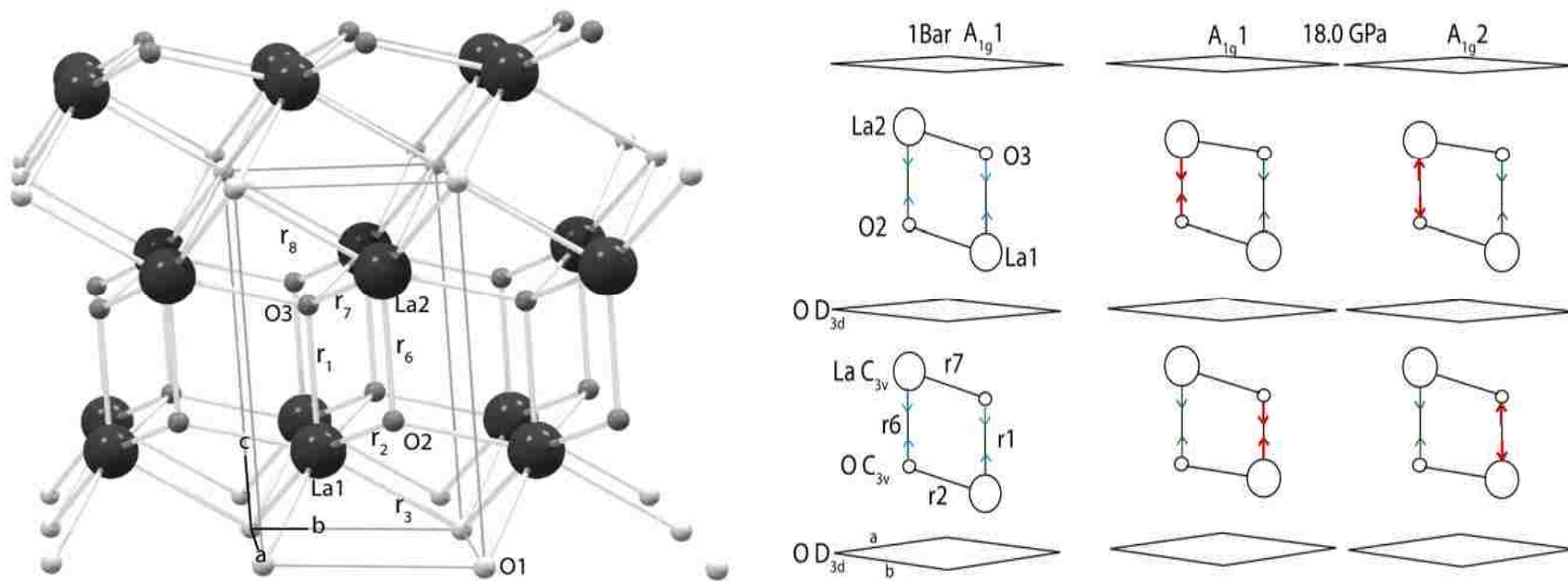
Figure 5.9 (a) The crystal structure of the A-type RES. Edges of the primitive cell are drawn, and the atoms included in the Bravais cell are labeled. Lanthanum atoms (dark gray), La1 and La2, are situated on one of the two C_{3v} sites. Oxygen atoms (medium gray), O2 and O3, are situated on the second C_{3v} site. Oxygen atoms (light gray), O1, occupy the only D_{3d} site. Bond lengths r_4 - r_5 , not labeled, are the O3-O1 and O3-O2 repulsion terms. (b) Super lattice structure shown at ambient pressure and at 18 GPa with the differences in r_6 and r_1 depicted qualitatively.
