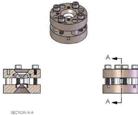
Figure 2.1 Cross-sectional and multi-angle view of the symmetric diamond anvil cell used in this study. There a total of four guide pins and four counter rotating hex head compression screws. The cell body is machined from hardened steel and the backing plates from either tungsten carbide or stainless steel.
