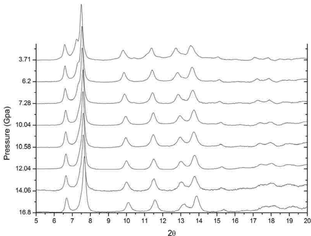
Figure 4.17 Diffraction patterns from Gd_2O_3 Experimental Run #3. Helium is used a pressure transmitting medium. Only the A-Type sesquioxide phase is observed throughout the entire experiment.
