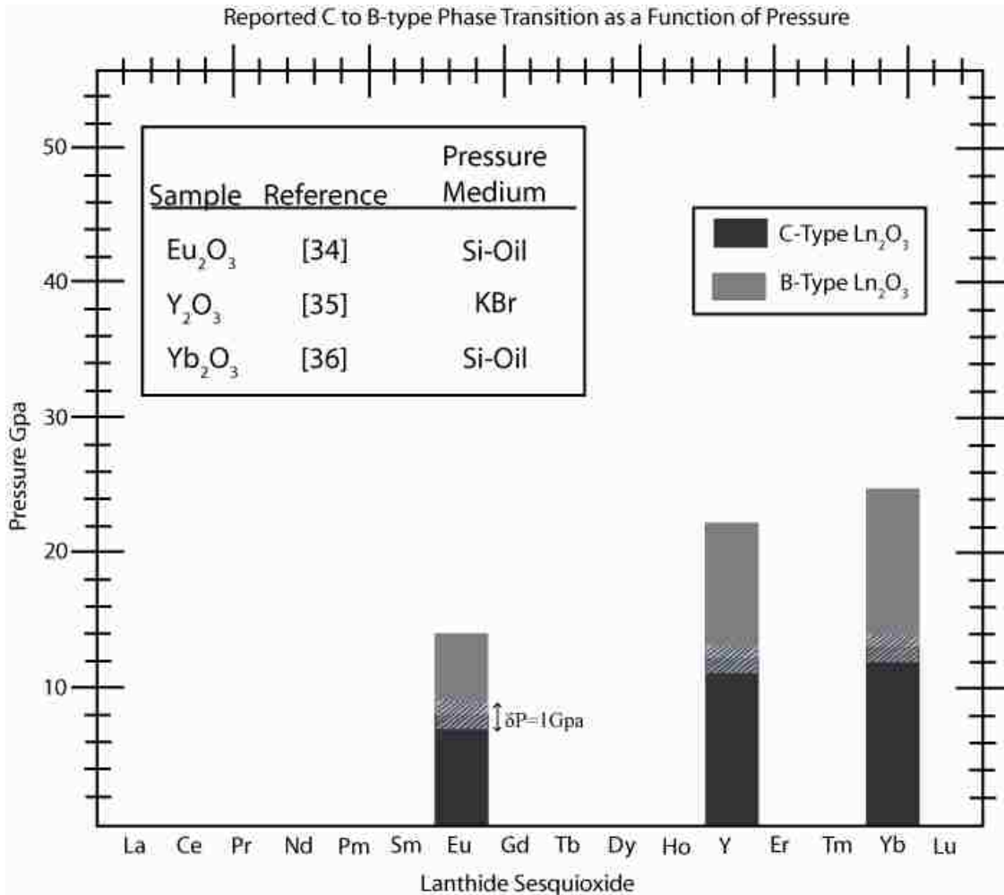
Figure 1.7 C to B-Type pressure induced structural phase transitions reported in the literature. Shown in the caption in the upper left are specific samples studied, the respective reference, and the pressure medium used in the experiment. The darker and lighter shaded portions of the bar graphs are representative of the C and B phases respectively.
