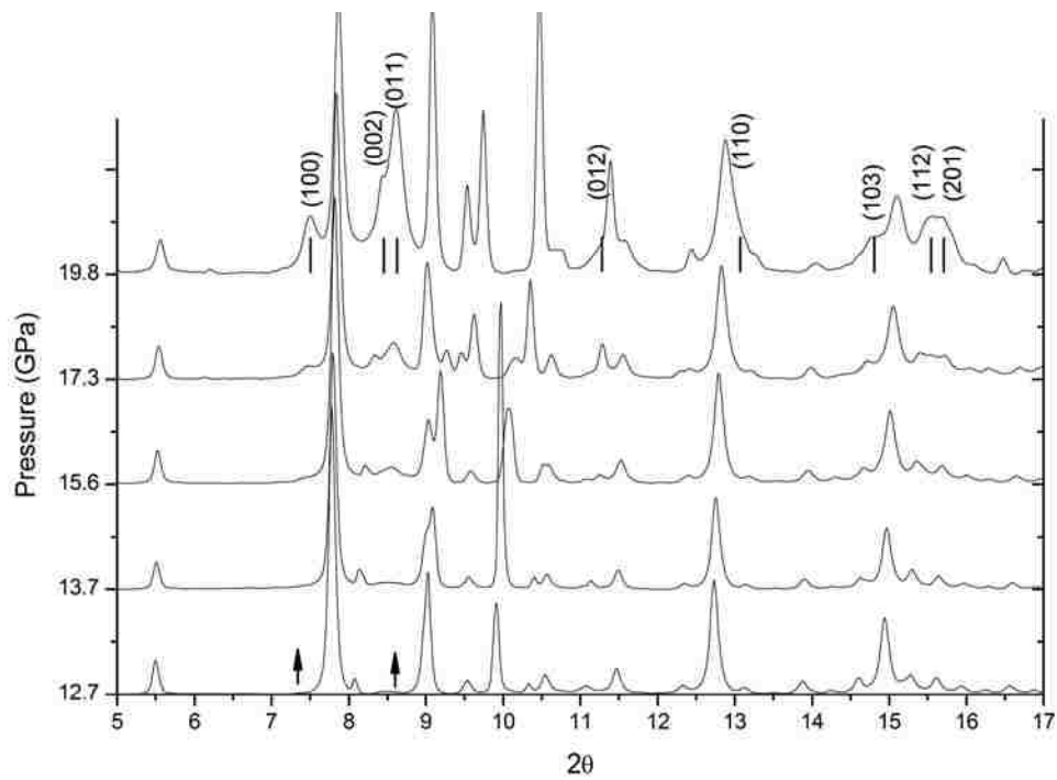
Figure 4.30 Enlargement of diffraction patterns of Y_2O_3 Experimental Run #1 from 12.7 to 19.8 GPa.
