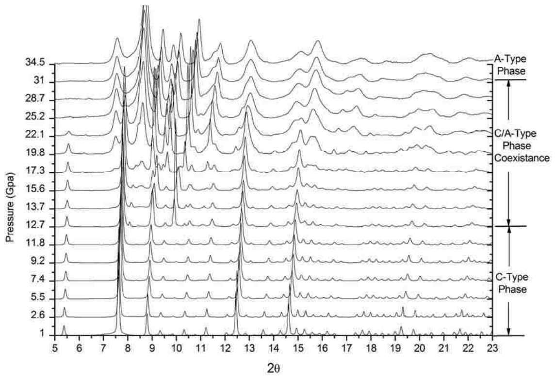
Figure 4.29 Diffraction patterns of Y_2O_3 Experimental Run #1.
