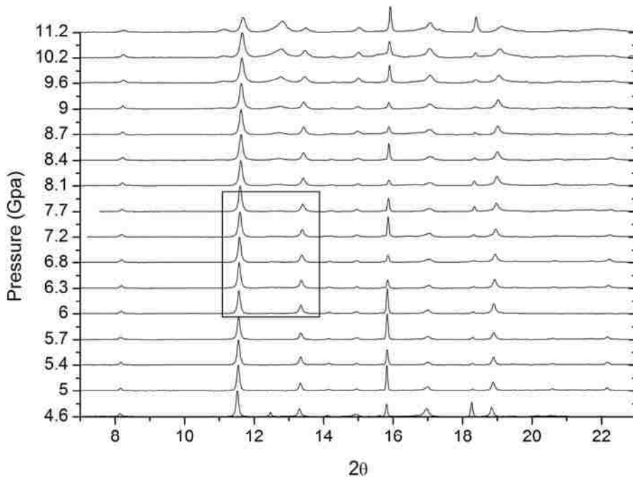
Figure 4.12 Diffraction patterns of \text{Gd}_2\text{O}_3 Experimental Run #5. A nitrogen pressure transmitting medium is used and the material compressed up to 11 GPa.
