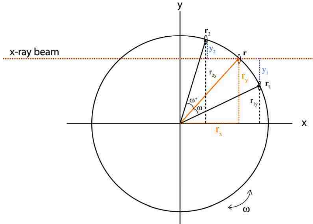
Figure 2.11 Sample centering diagram.
