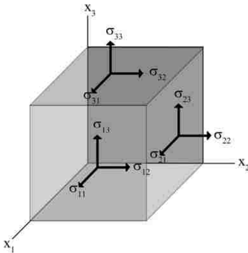
Figure 2.2 The stress tensor represented in Cartesian coordinates.
