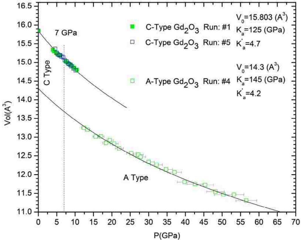
Figure 4.19 Volume versus pressure equation of state for \text{Gd}_2\text{O}_3 .
