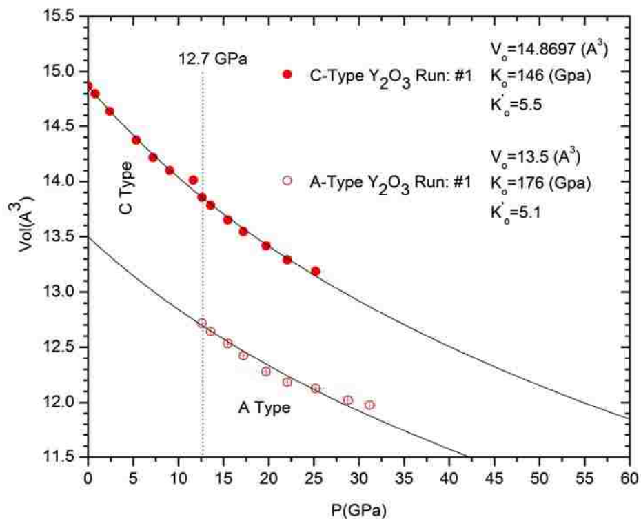
Figure 4.31 Volume versus pressure equation of state for Y 2 O 3
