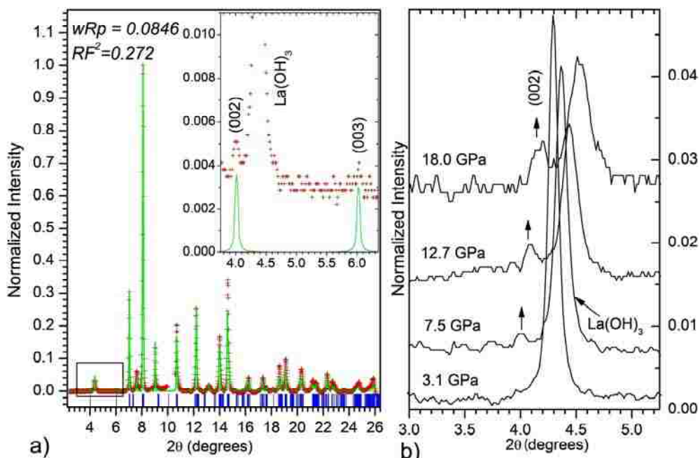
Figure 5.2. (a) Diffraction pattern of \text{La}_2\text{O}_3 at 7.5 GPa. Red pluses indicate the measured pattern and the solid green line represents the calculated super lattice diffraction pattern. The inset corresponds to the inscribed box at the bottom left. (b) Enlarged region of the diffraction patterns from \text{La}_2\text{O}_3 at various pressures. Upward arrows indicate a super lattice reflection indexed to the (002) plane. A peak from \text{La}(\text{OH})_3 is present in the data and labeled.
