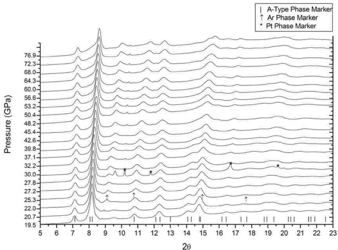
Figure 4.16 Diffraction patterns for Gd_2O_3 Experimental Run #4. Diffraction peaks from the A-Type phase, Ar, and Pt are marked with vertical lines, arrows and asterisks above the respective plot.
