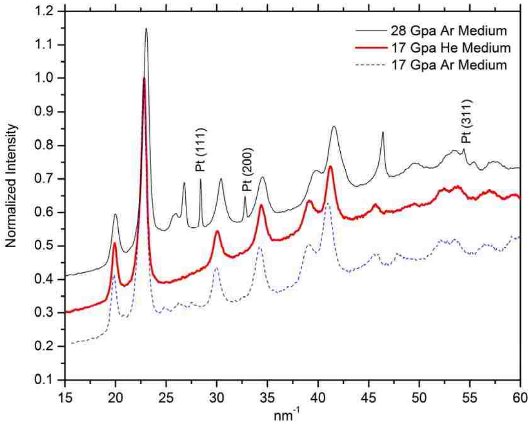
Figure 4.18 Diffraction patterns of A-Type \text{Gd}_2\text{O}_3 compressed using helium and argon pressure media in separate experiments. The thick and thin dashed curves are from experiments where He and Ar are used as pressure media respectively at approximately 17 GPa. The thin curve is diffraction of \text{Gd}_2\text{O}_3 in the A-Type phase at 28 GPa and Pt peaks are labeled.
