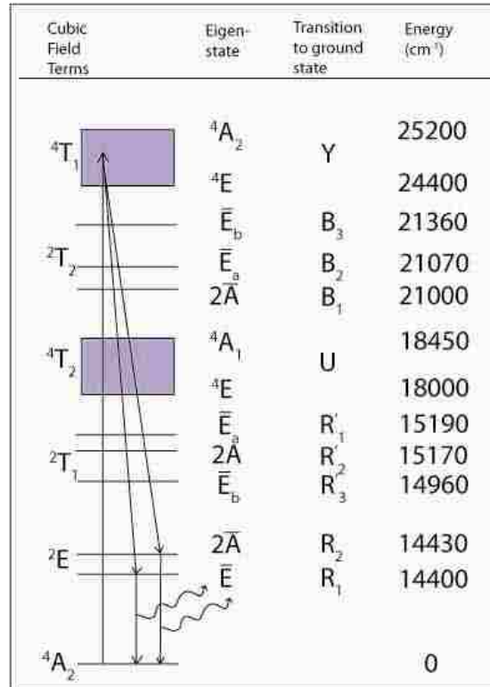
Figure 2.4. Electronic energy diagram for Al_2O_3:Cr^{3+} . The arrows outline the pumping scheme used in all ‘in-house’ pressure measurements. The cubic crystal field terms are subsequently split by smaller trigonal field and spin-orbit perturbations to the free ion energy levels. 46
