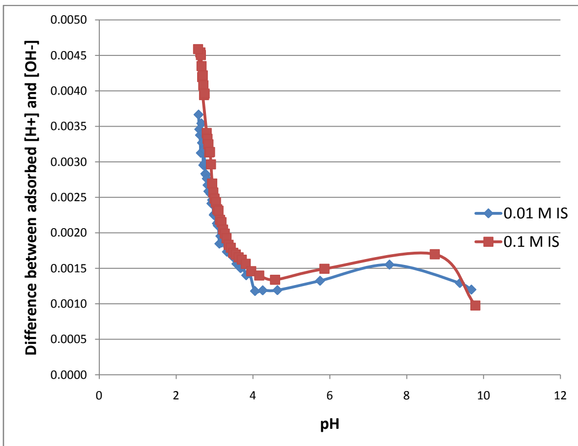
Figure 3.4: Titrations of graphite under different ionic strength
