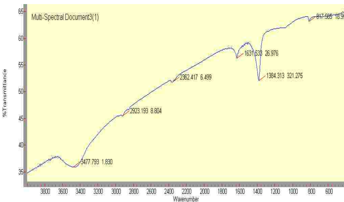
Figure 3.2: Infrared Spectra of Experimental Graphite
