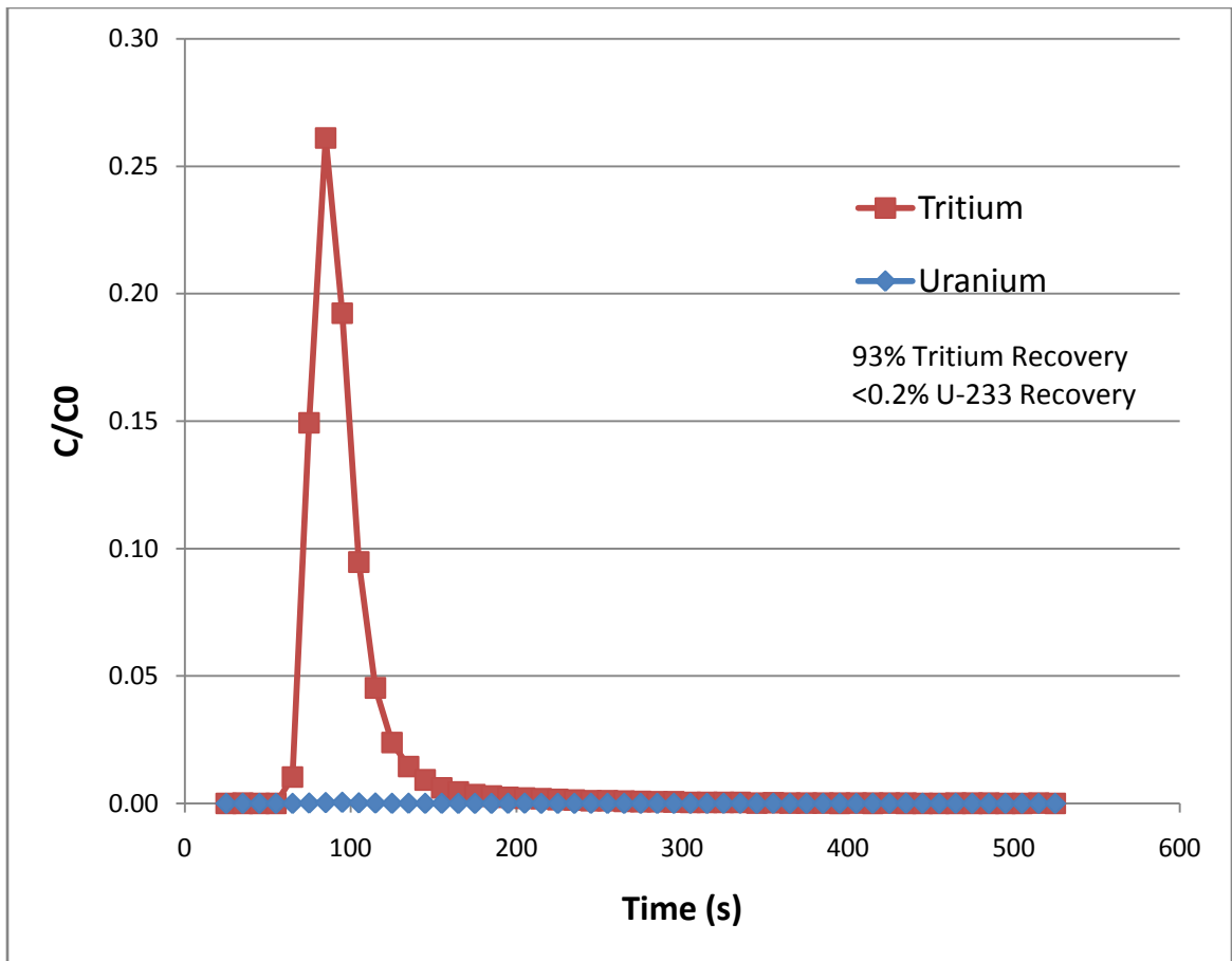
Figure 3.14: Initial Fast Flow Column Experiment ( pH = 6.5 ) 2 \mu g U-233
