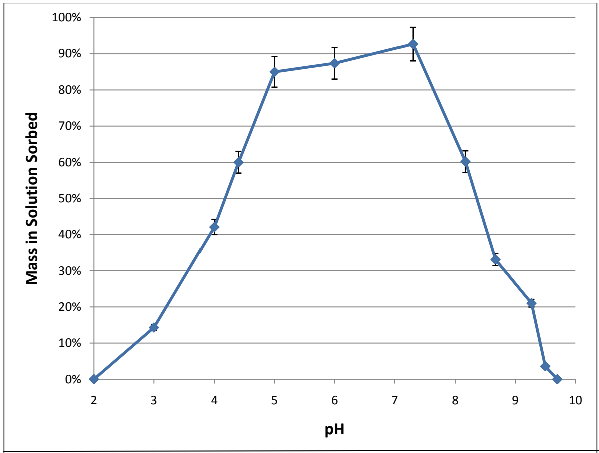
Figure 3.5: Uranium sorption (Initial [U] = 500 ppb) to graphite as a function of pH Ionic Strength = 0.01 M, p\text{CO}_2 = 390 ppm
