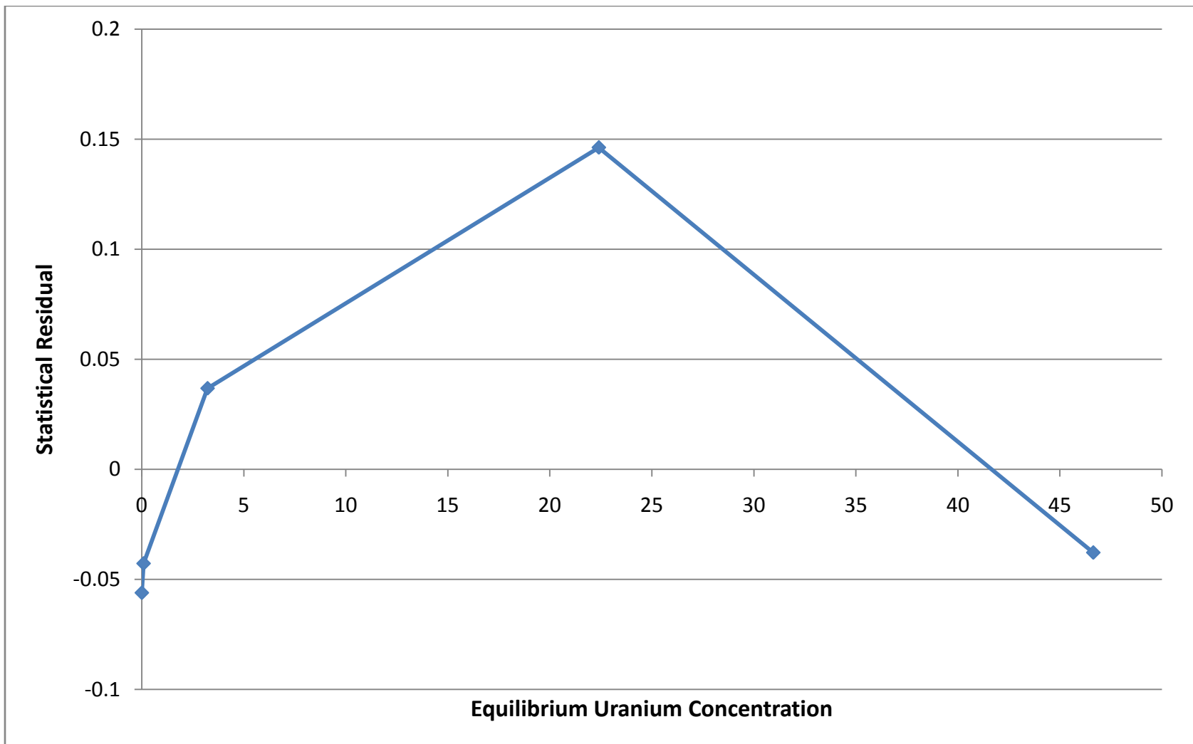
Figure 3.10: Residuals for Langmuir fit of Sorption data at pH = 5
