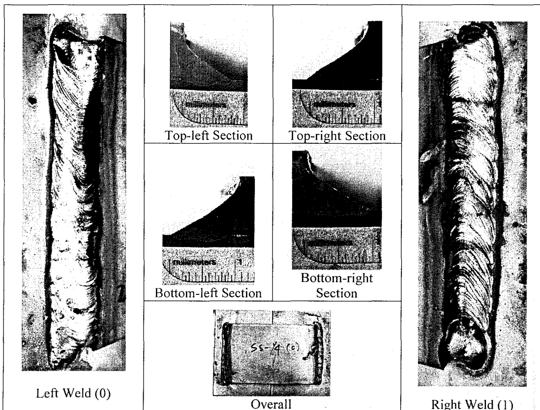
Figure 6.33: Specimen SS-(1/4)0
