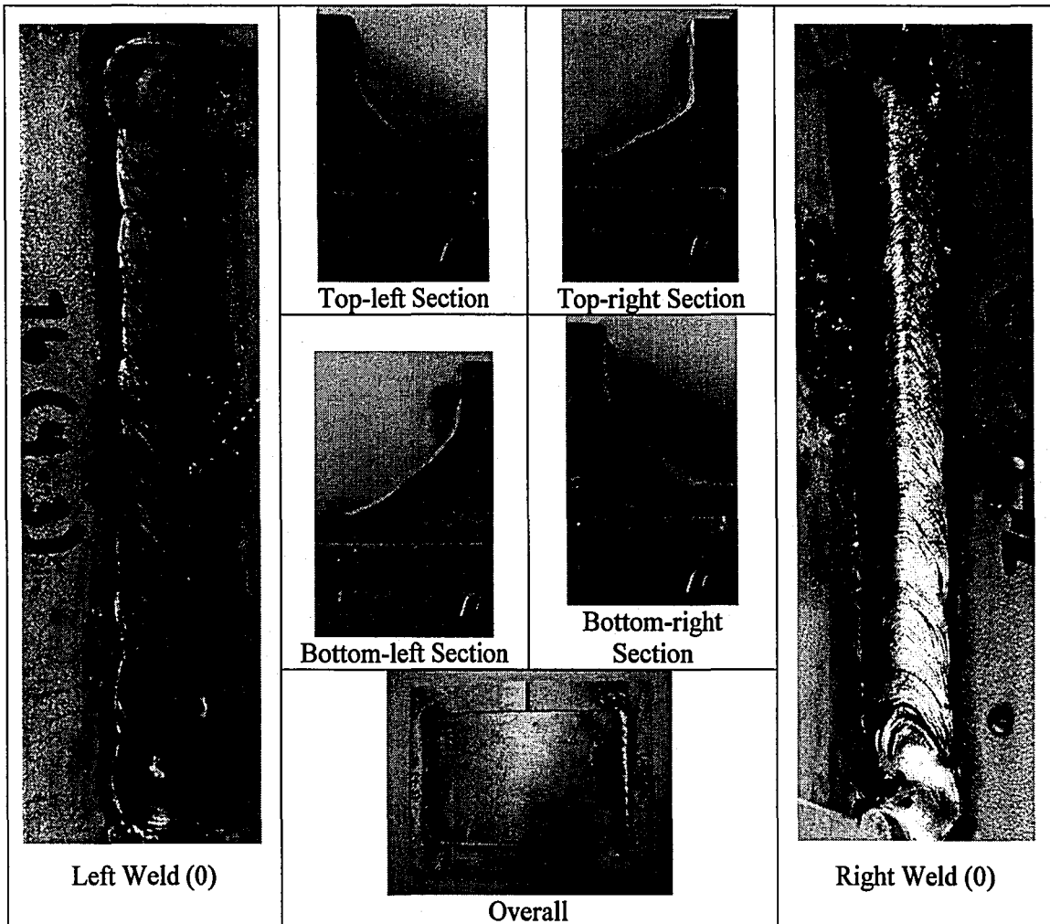
Figure 6.7: Specimen SS-76
