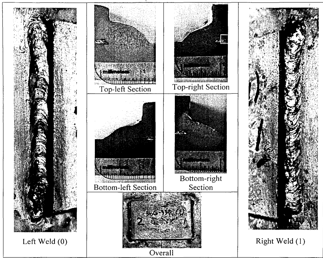
Figure 5.3: Specimen 36G-33(1)
