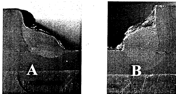
Figure 8.30: Polished Sections from Specimen T-5
