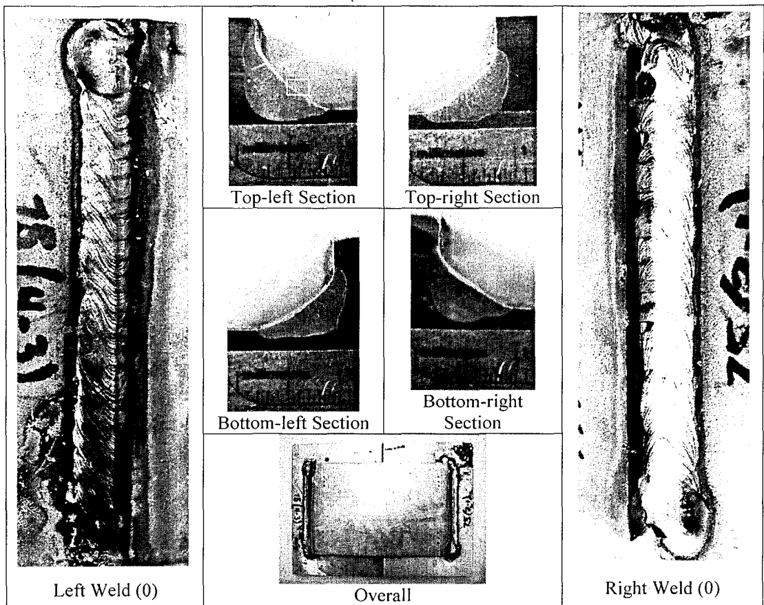
Figure 6.5: Specimen SS-75
