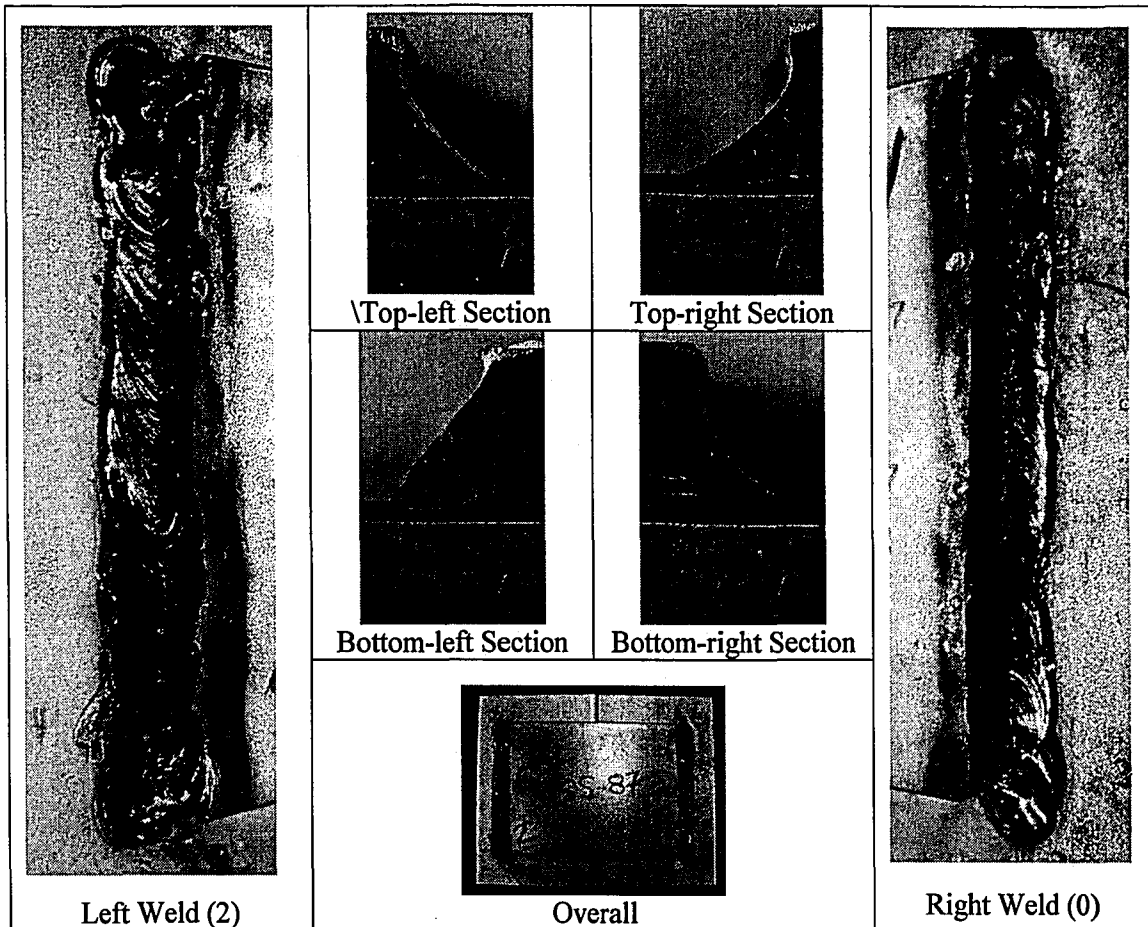
Figure 6.16: Specimen SS-87
