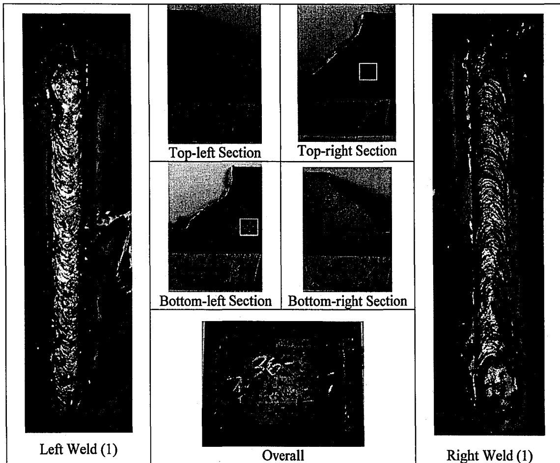
Figure 4.6: Specimen 36-6
