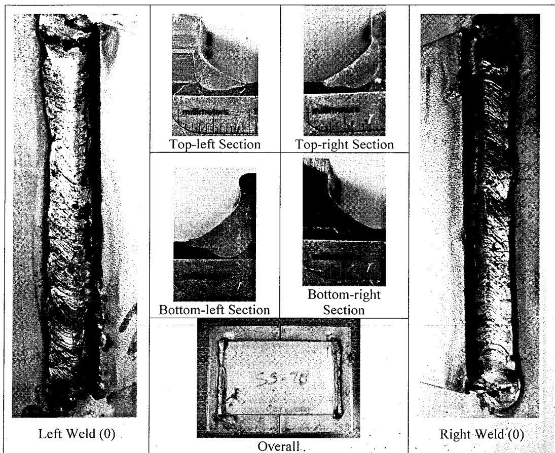
Figure 6.9: Specimen SS-78
