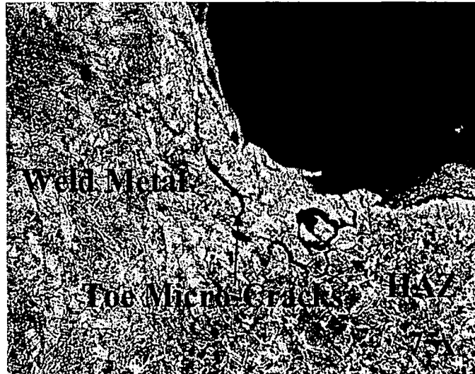
Figure 5.7: Toe Micro-Cracking in Specimen 36G-33(2)-Top-left Section
