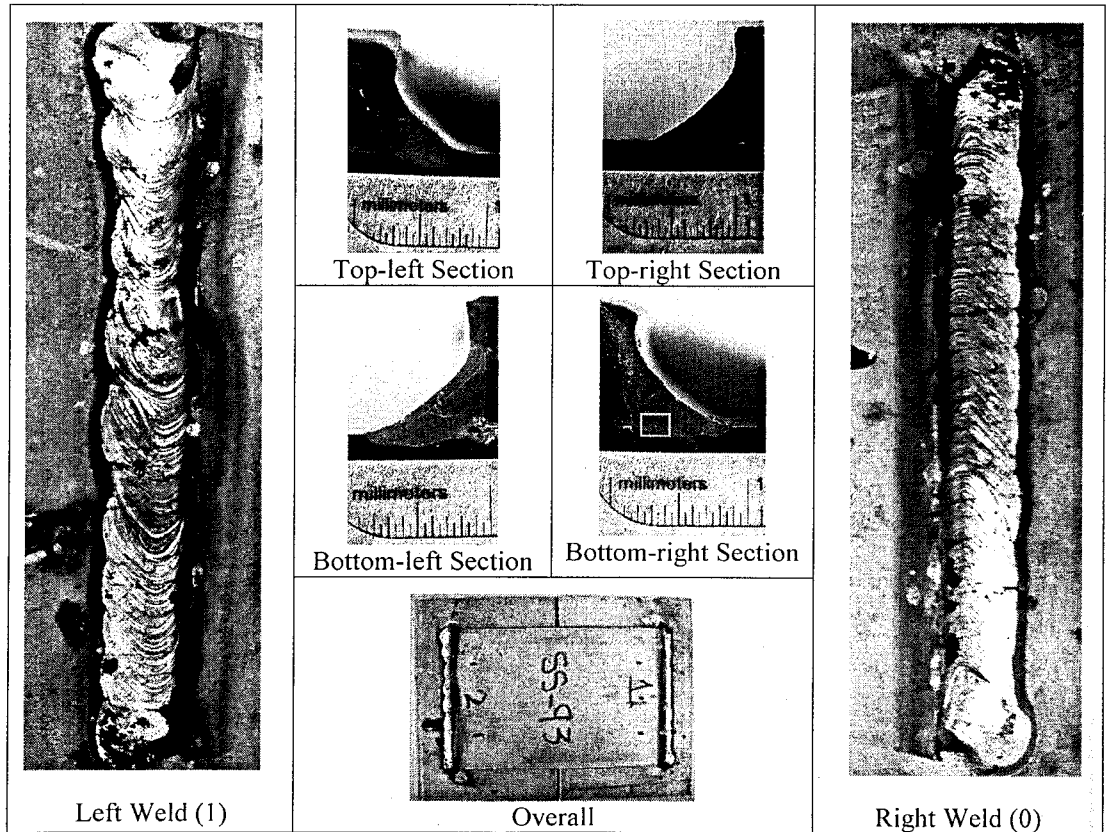
Figure 6.25: Specimen SS-93
