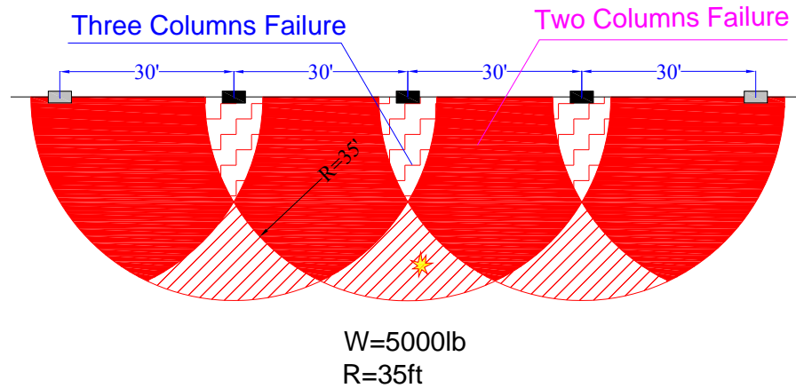
Figure 3-17: Blast load effects due to Direct Shear Failure at W=5000lb
