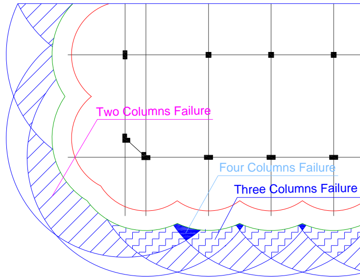
Figure 3-20: Flexural failure condition at W=5000\text{lb}
