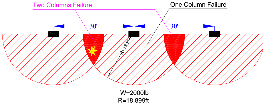
Figure 3-6: Blats load effects due to Brisance Failure at W=2000lb
