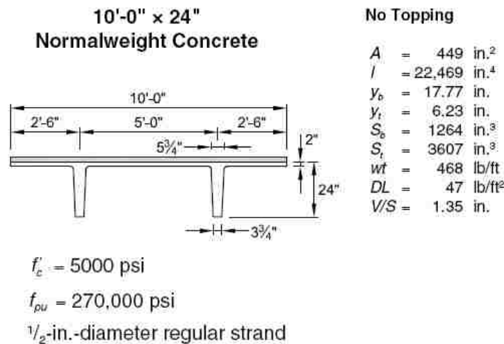
Figure 5-7: Properties of double tee slab(PCI, 2010)
