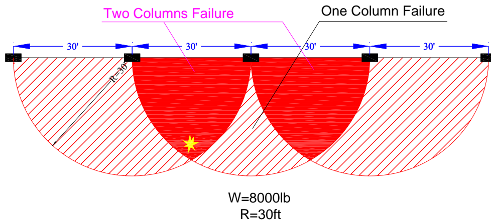
Figure 3-7: Blast load effects due to Brisance Failure at W=8000lb
