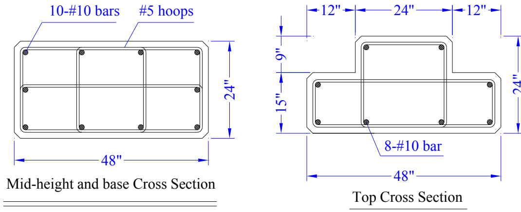
Figure 3-1: Column cross-sections
