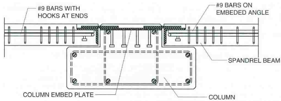
Figure 5-23: Spandrel-to-column connection (PCI, 2007)
