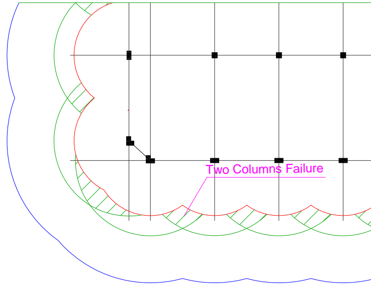
Figure 3-21: Direct shear failure condition at W=5000\text{lb}
