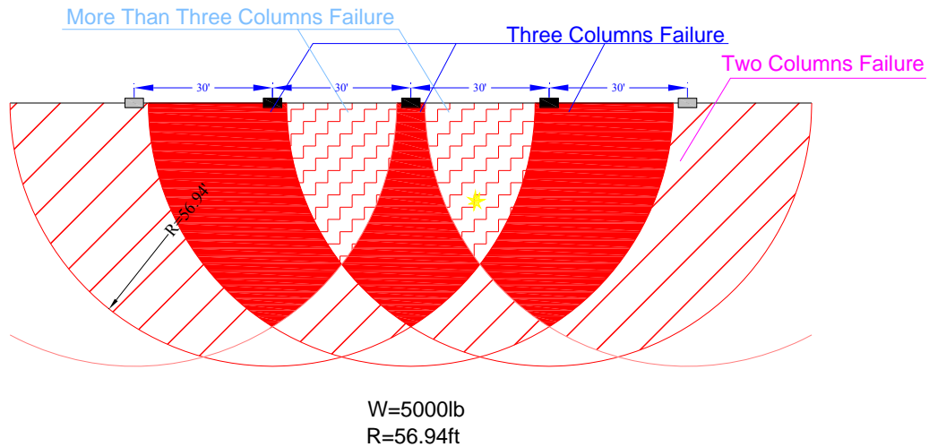
Figure 3-13: Blast load effects due to Flexural Failure at W=5000lb
