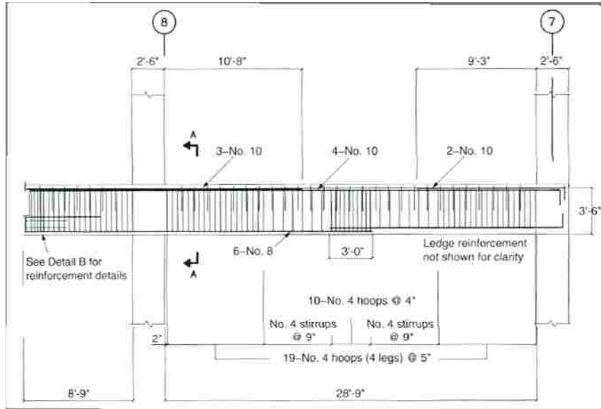
Figure 2-8: Reinforcement details about overhung frames (PCI, 2007)
