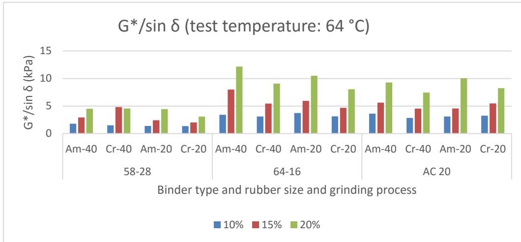
Figure A1. G*/sin δ (test temperature: 64 °C)
