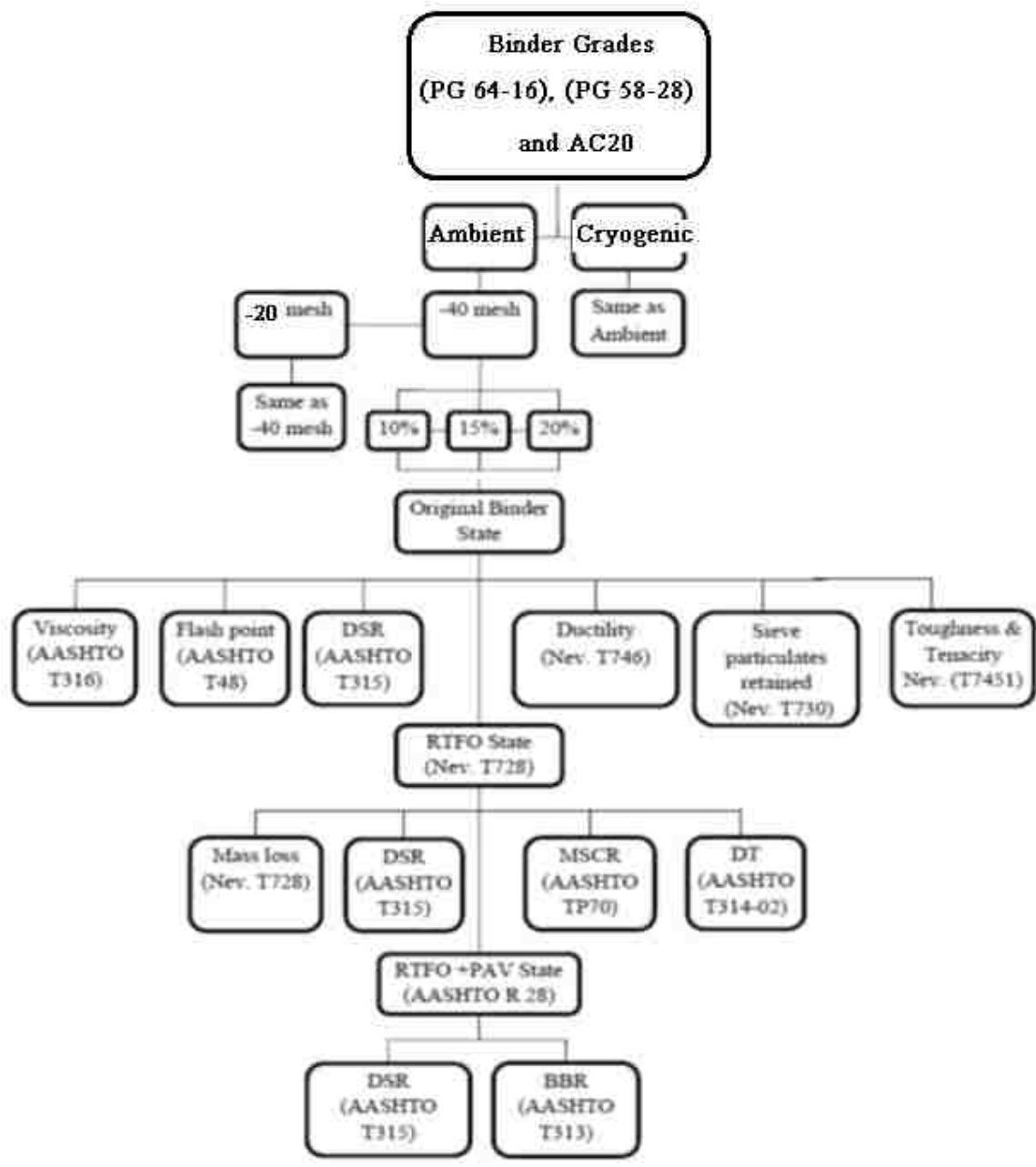
Figure 32. Methodology of evaluating properties of rubber modified binder
