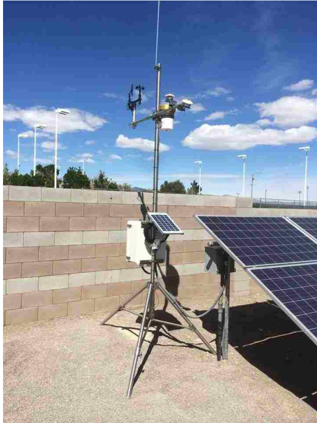
Figure 4. Weather Station installed at the City of Las Vegas West Maintenance Yard to assist in the data collection for the solar plant
