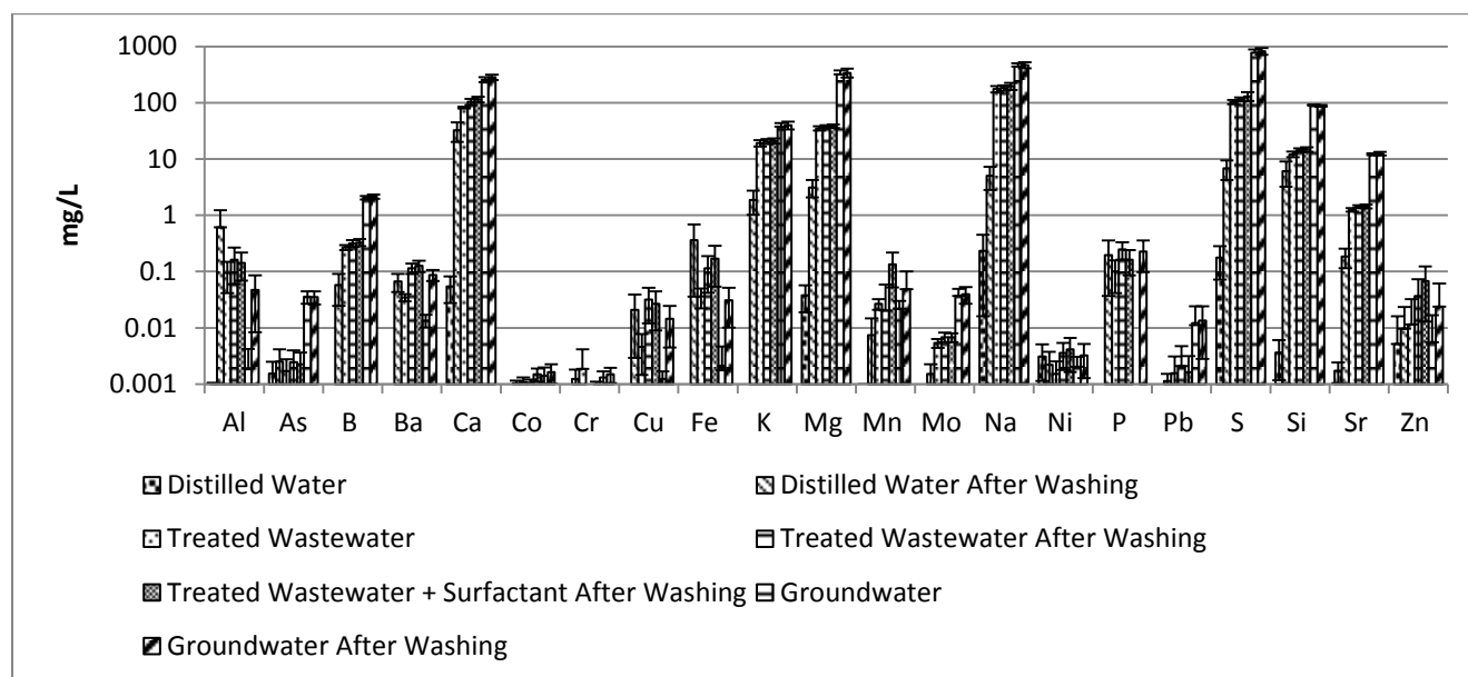
Figure 34. Mean trace concentration of 21 metals from the second to the eighth panel washes
