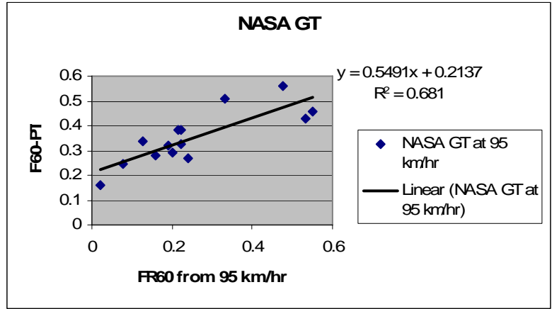
Figure 6 NASA GT May 2007 Calibration Constants from F60 and FR60 at 95 km/hr with DFT-PTI
