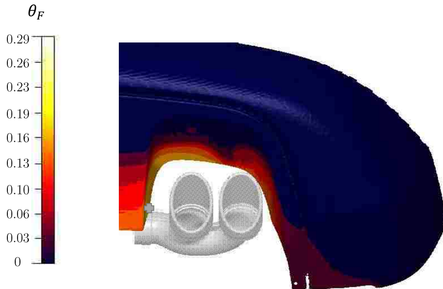
Figure 4-45: \theta_F contours for predicted highest \theta_{FM} case, optimized geometry.
