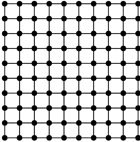
Figure 2-1: A 2 input, 10 level full factorial sample.
