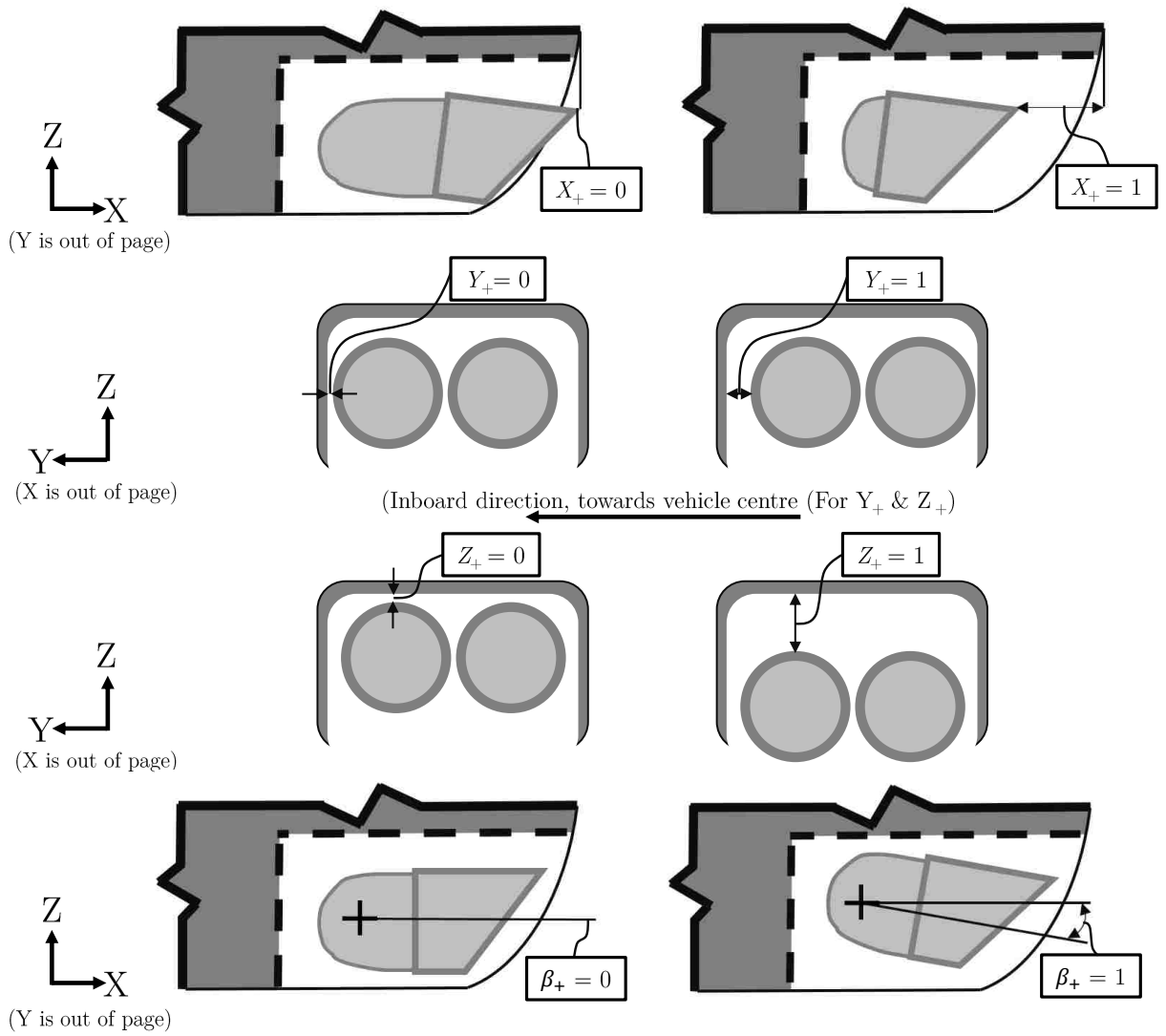
Figure 3-12: Geometric parameters (driver's side view for X_+ and \beta_+ and rear view for Y_+ and Z_+ ).
