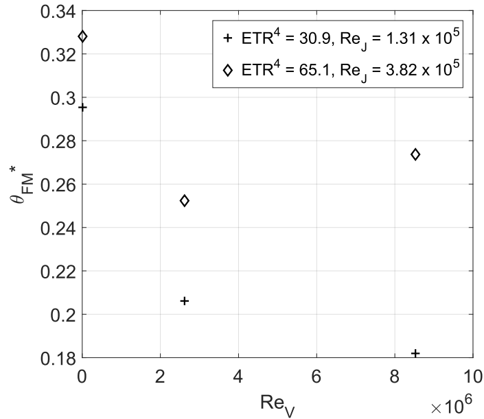
Figure 3-14: \theta_{FM}^* values of cases simulated with CFD to determine non-geometric parameters.
