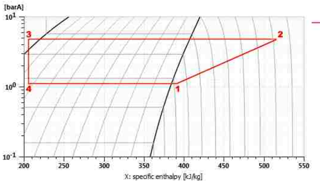
Fig. 3. 7: Pressure-enthalpy diagram of the thermodynamic cycle performed by the heat pump (from 1 to 2 the compressor, from 2 to 3 the condenser, from 3 to 4 the expansion valve and from 4 to 1 the evaporator).
