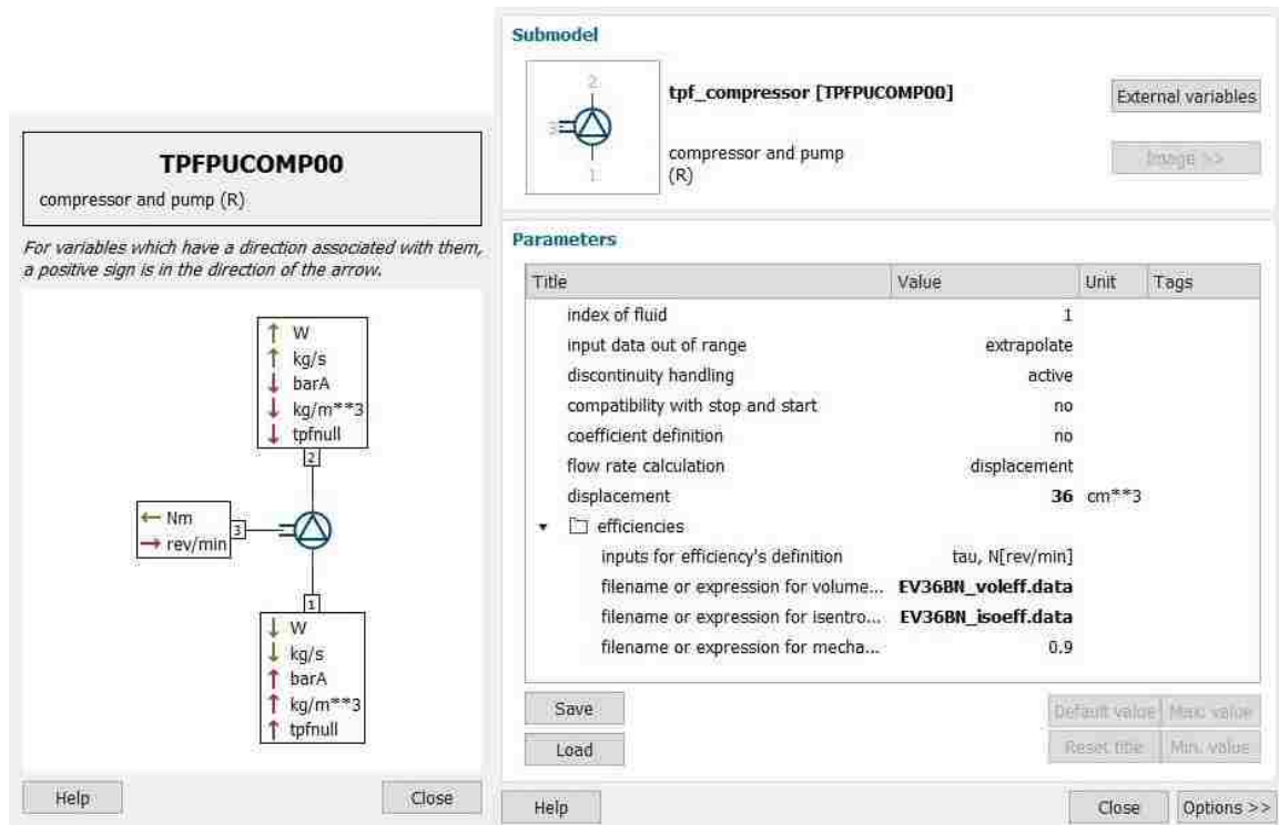
Fig. 2. 4: Element adopted for the modelling of the compressor; list of external variables and parametrization.
