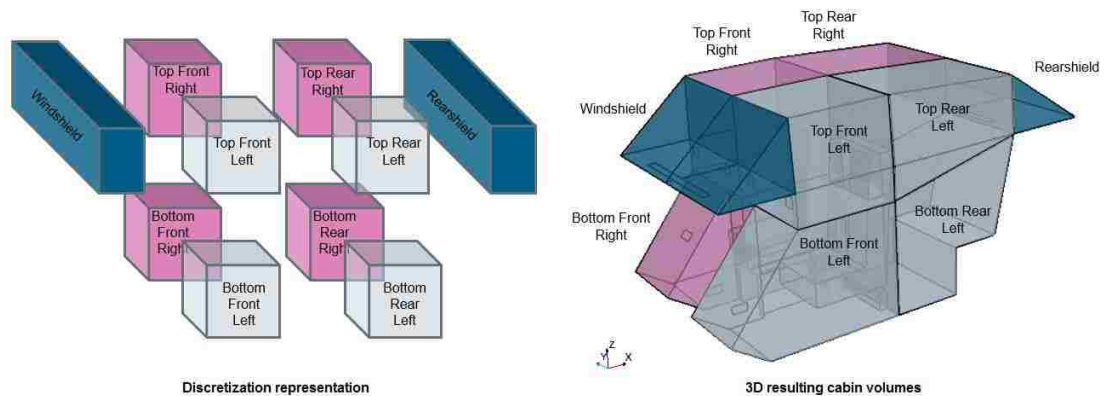
Fig. 4. 1: Representation of the cabin space split in 10 volumes.
