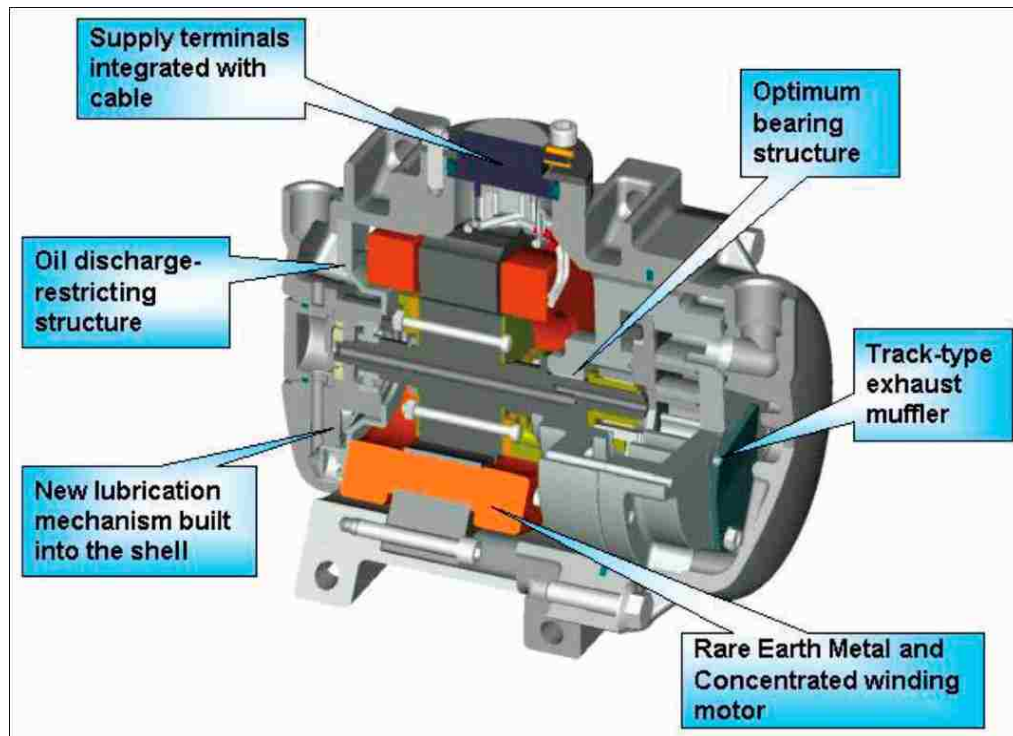
Fig. 1. 5: Main element technologies of the electric compressor [20].
