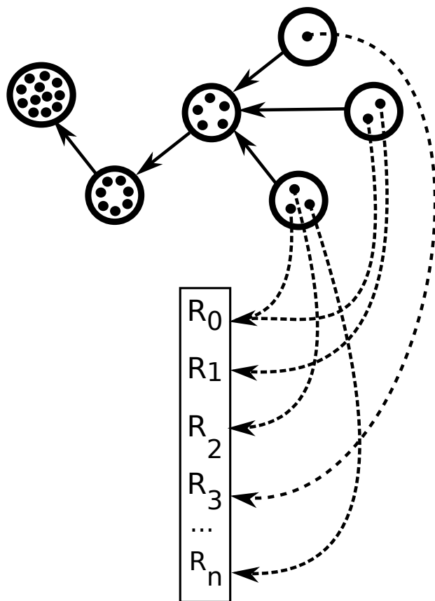
Figure 3.1: An illustrative example of a \mathbf{Facet}_i category shows a basic exemplary structure of the facets within this facet type. The objects are sets of pointers to resources classified as that particular facet type. For convenience, only pointers from leaf nodes have been drawn.
