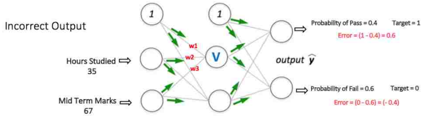
Figure 3.6: Forward propagation step. Source[19]
