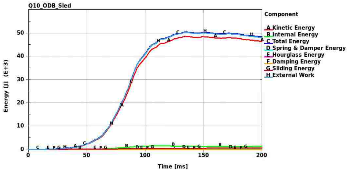
Figure 120 – Energy balance of the sled test simulation
