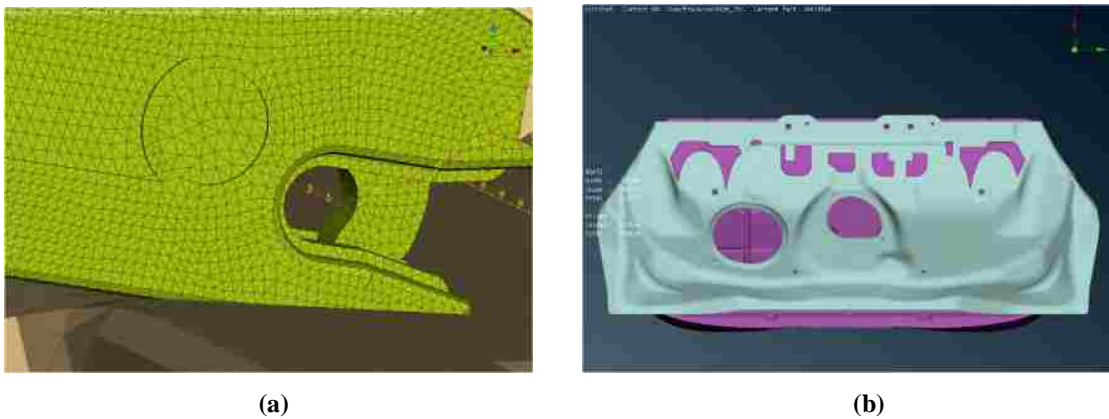
Figure 70 – Detected initial penetration of CRS clamps against the seat foam (a) and of foam the vehicle body (b, bottom view)
