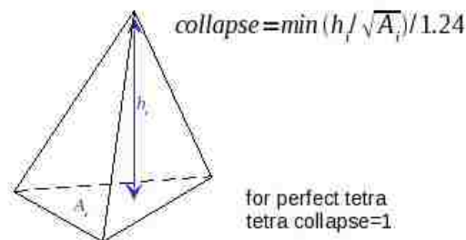
Figure 60 – Representation and definition of tetra collapse
