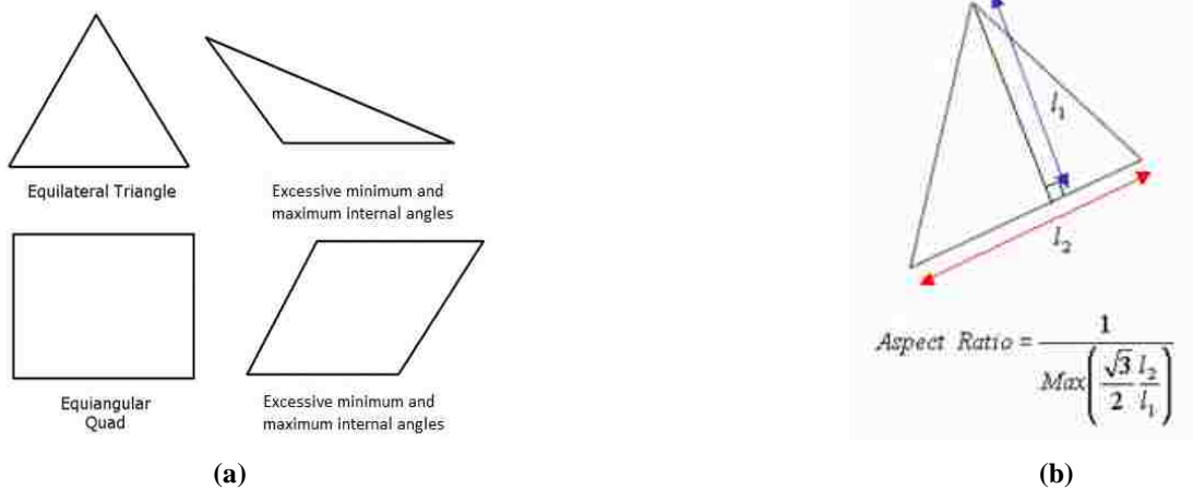
Figure 58 – Representations and definition of minimum and maximum internal angles (a) and aspect ratio (b)
