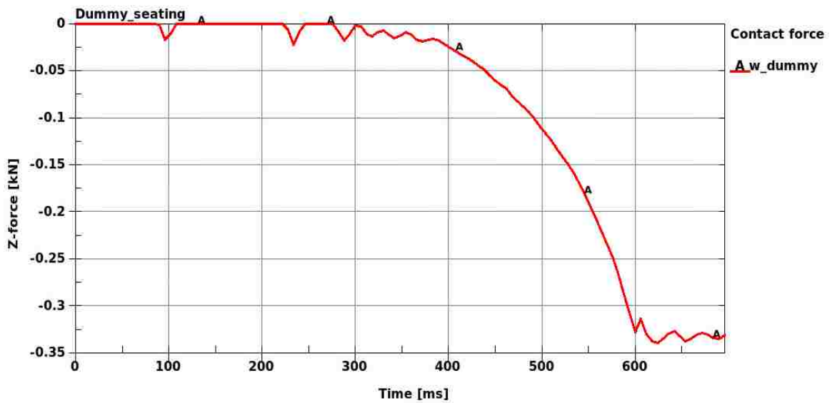
Figure 85 – Vertical contact force imposed by the rigid dummy on the CRS
