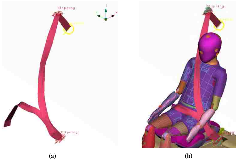
Figure 103 – Finite Element seat belt, slip rings, and retractor
