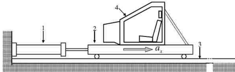
Figure 37 – HYGE Sled scheme. 1) pneumatic hydraulic piston; 2) bogie; 3) rails; 4) element to test [9]
