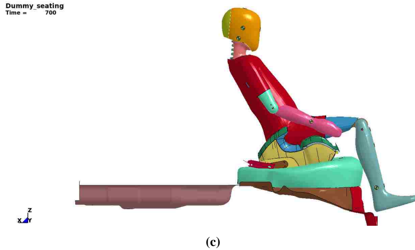
Figure 83 – Dummy seating simulation system at 0 (a), 360 (b) and 700 ms (c)
