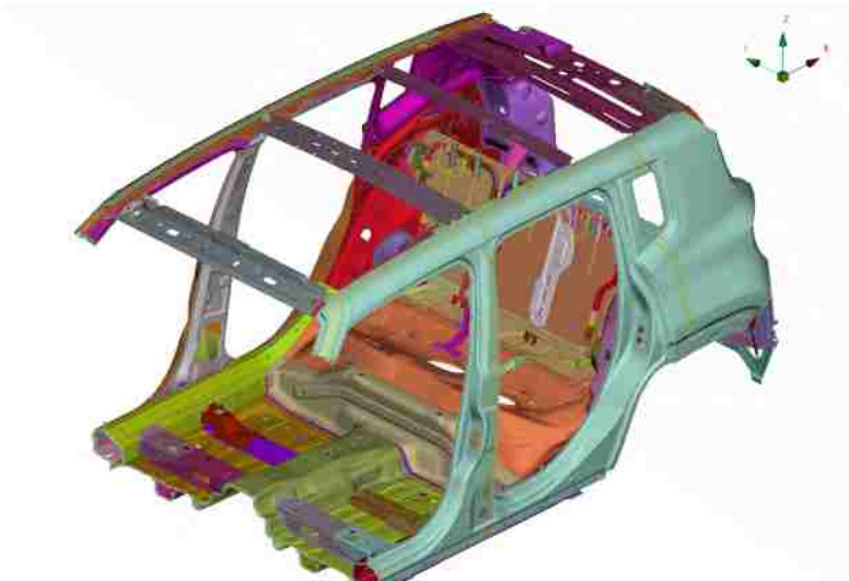
Figure 49 – Isometric view of the vehicle body FE model
