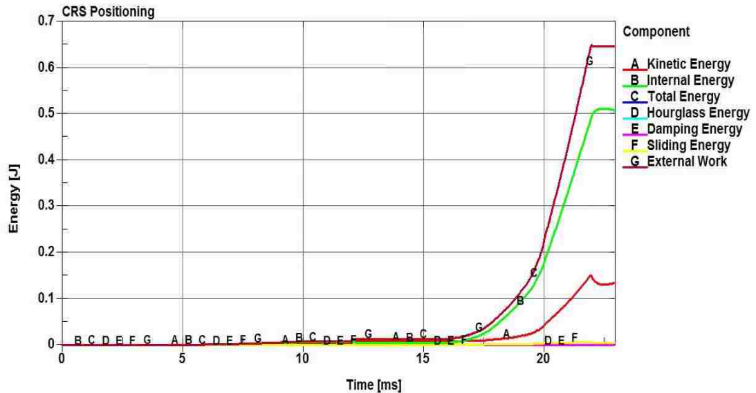
Figure 73 – Energy balance of the depenetration simulation
