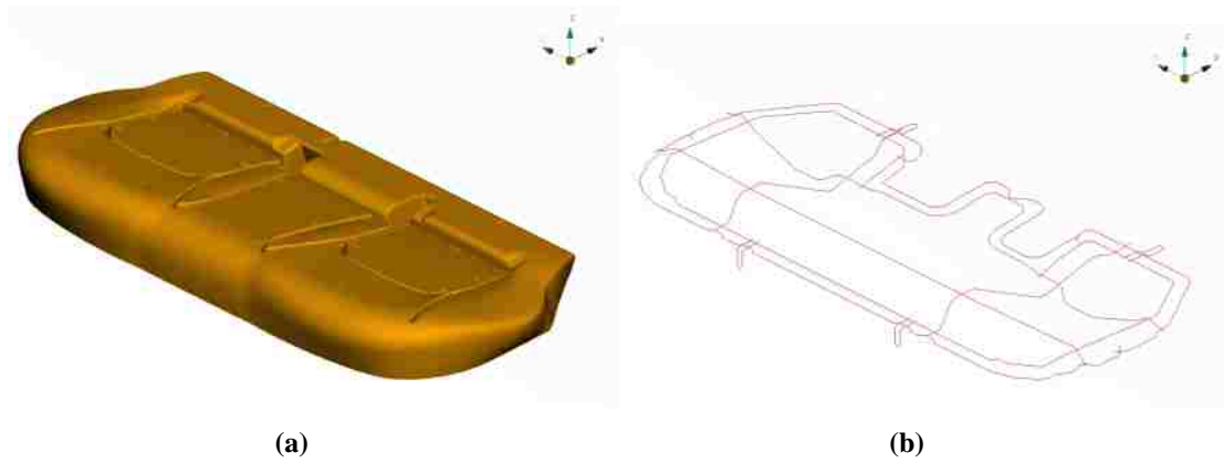
Figure 51 – Isometric view of the 2 nd -row seat foam (a) and its relative suspension frame (b) FE models
