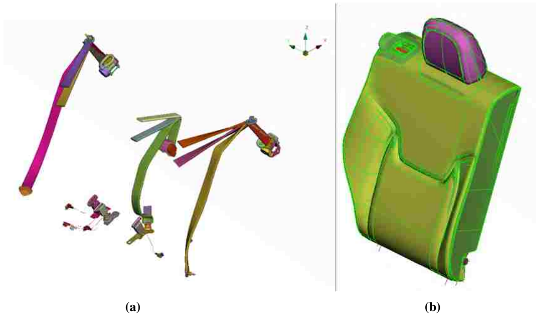
Figure 53 – Isometric view of the restraint system (a) and backseat foam CAD models
