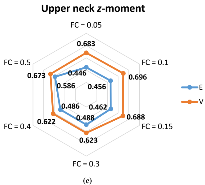
Figure 139 – Sensitivity analysis on the upper neck moment
