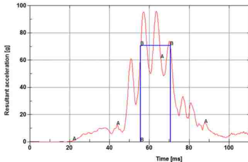
Figure 7 – HIC criterion calculation [11]
