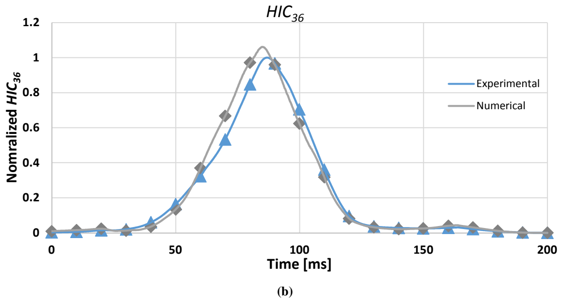
Figure 126 – Experimental and numerical HIC_{36}
