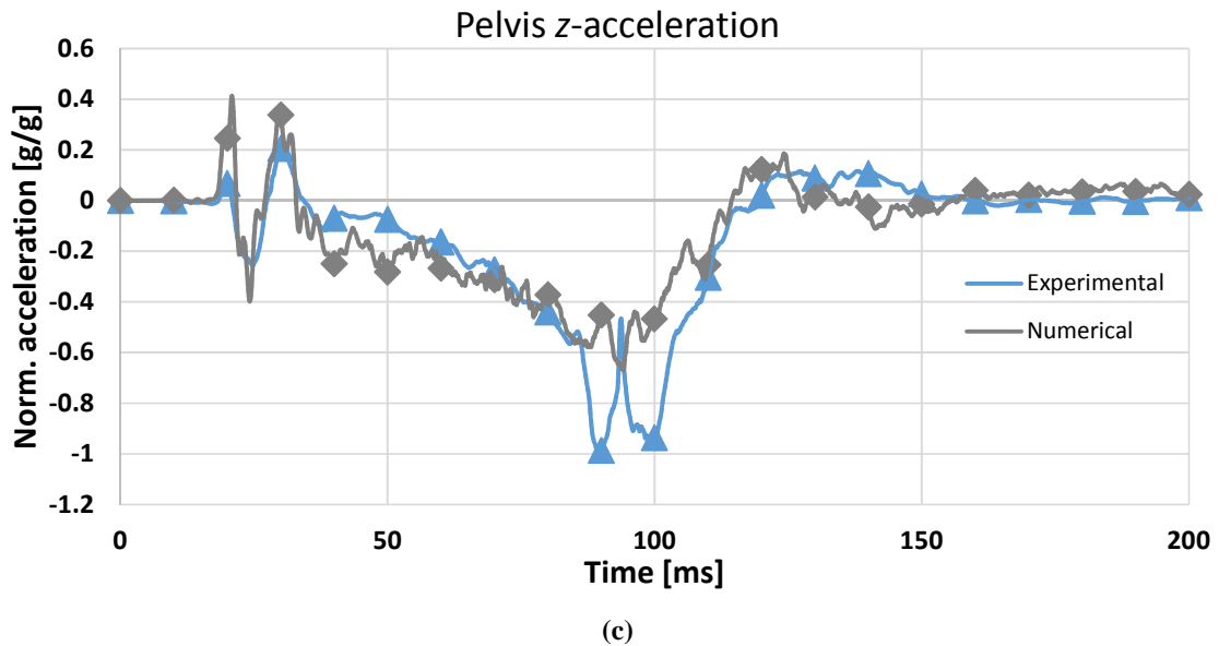
Figure 128 – Experimental and numerical pelvis x (a), y (b) and z (c) accelerations
