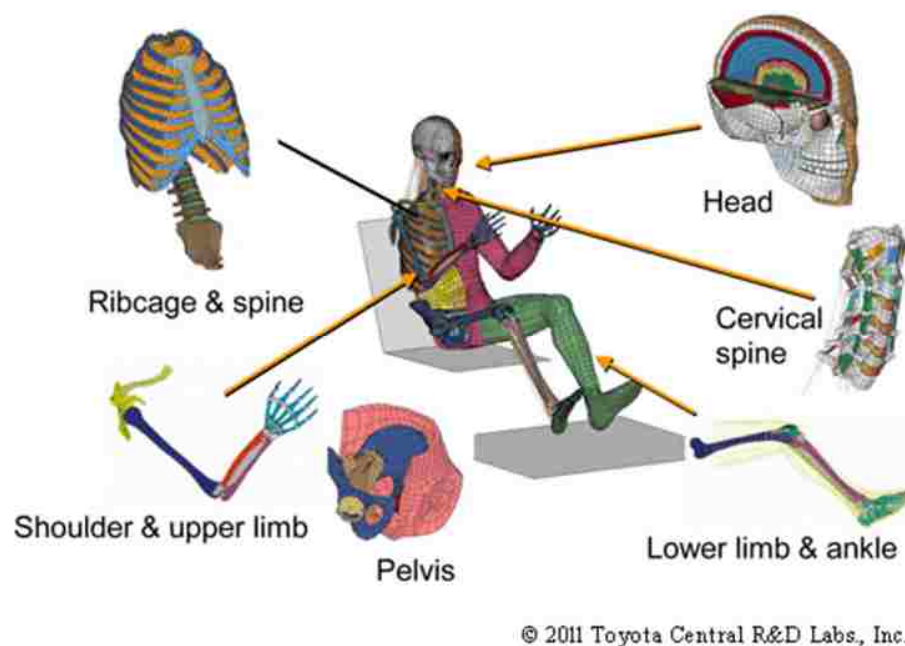
Figure 40 – THUMS Finite Element model [82]
