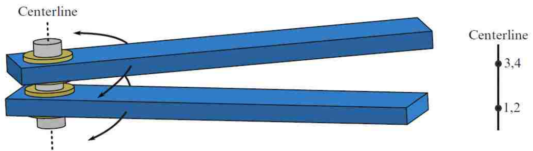
Figure 69 – LS-DYNA revolute joint scheme [94]
