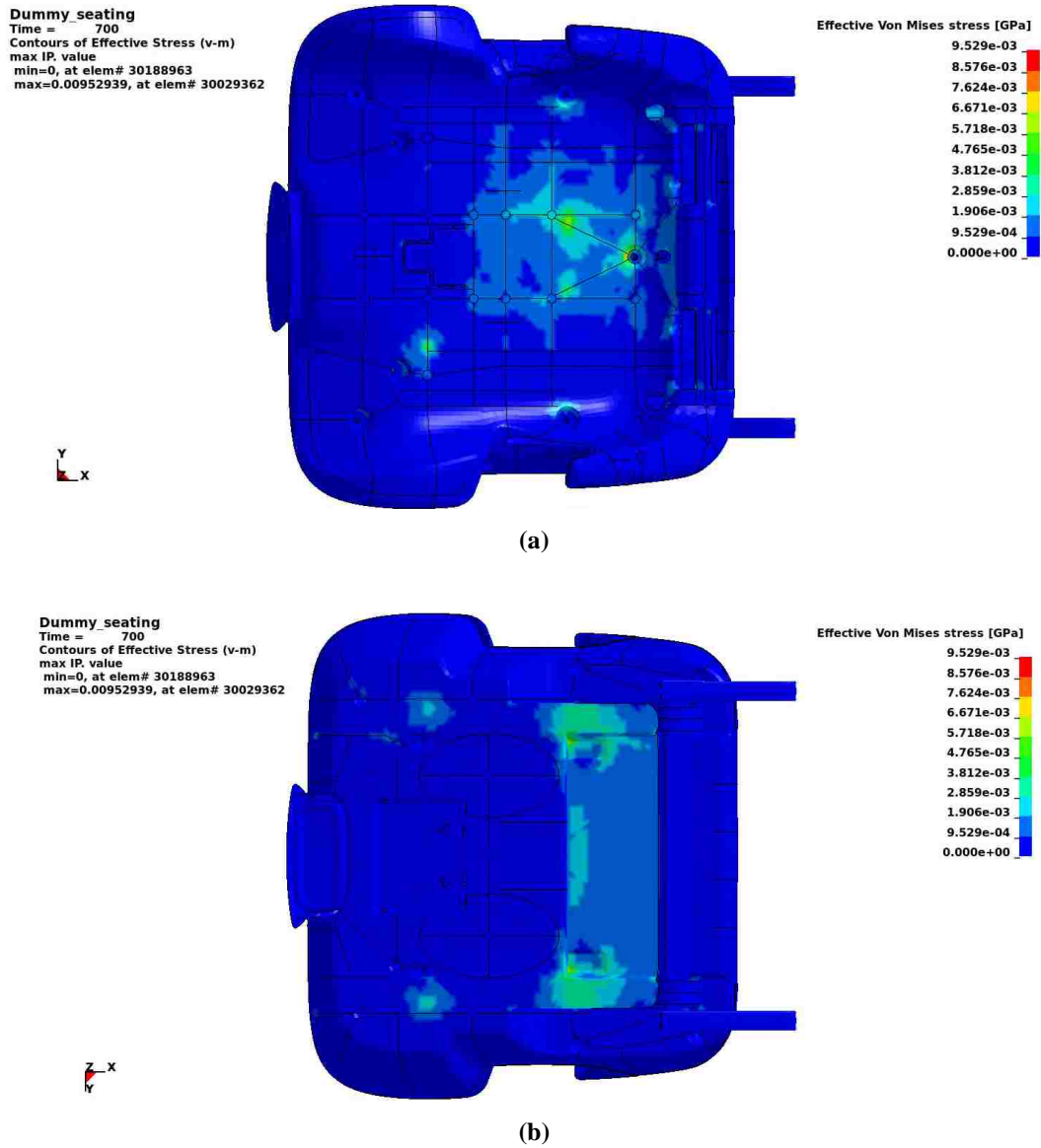
Figure 89 – Top (a) and bottom (b) view of contours of stress on the booster seat at 700 ms of simulation
