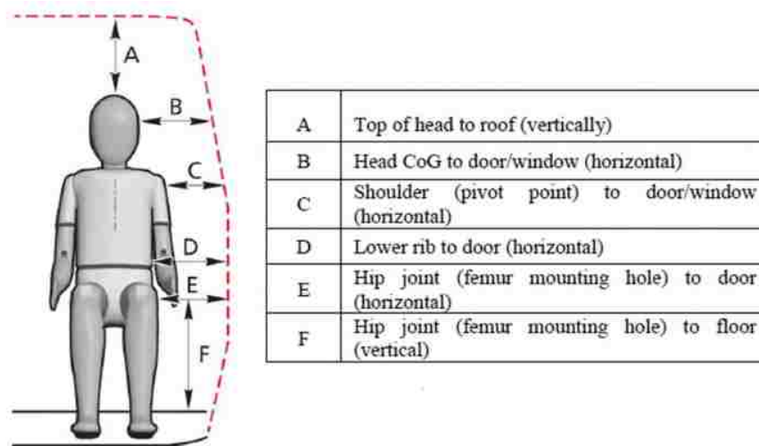
Figure 35 – Q10 dummy measurements [76]
