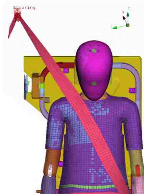
Figure 101 – Front view of the virtual shoulder belt
