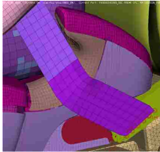
Figure 100 – FE shoulder belt wrapping the booster seat
