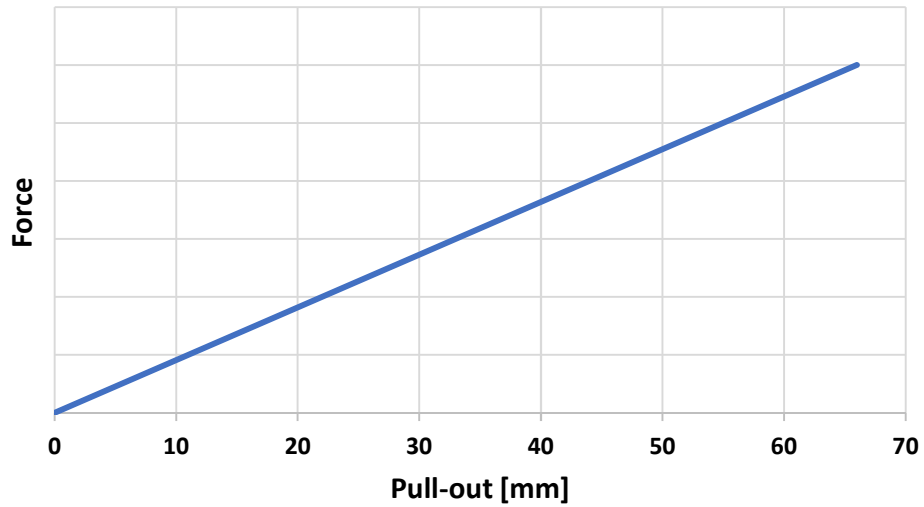
Figure 117 – Retractor unloading curve
