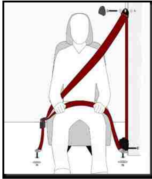
Figure 15 – The standard three-point seat belt [15]
