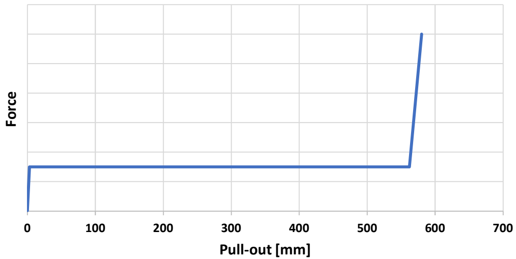
Figure 116- Constant Load Limiter retractor loading curve
