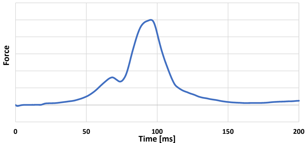
Figure 119 – Load on the lap belt measured during the experimental test
