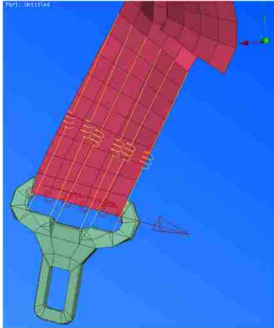
Figure 107 – FE model of the Dynamic Locking Tongue
