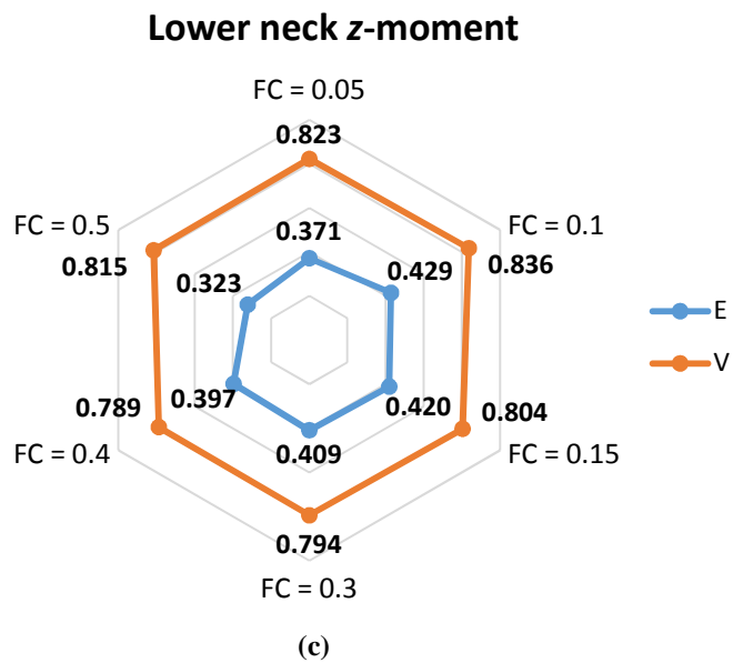
Figure 141 – Sensitivity analysis on the lower neck moment
