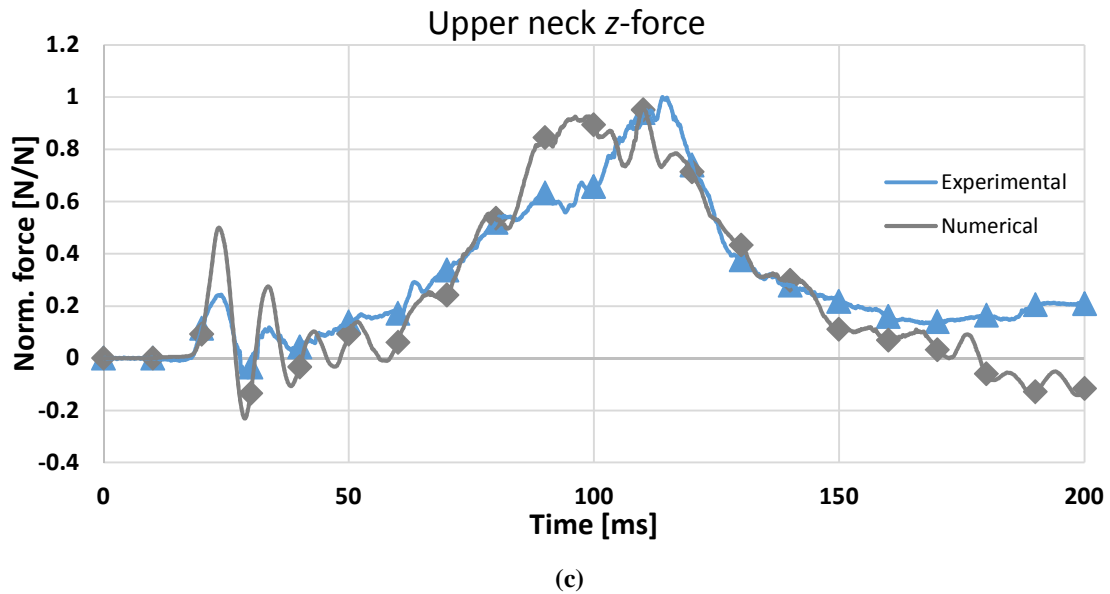
Figure 129 – Experimental and numerical upper neck x (a), y (b) and z (c) forces
