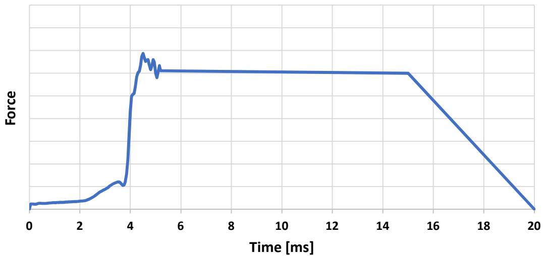
Figure 113 – Pretensioner starting loading curve
