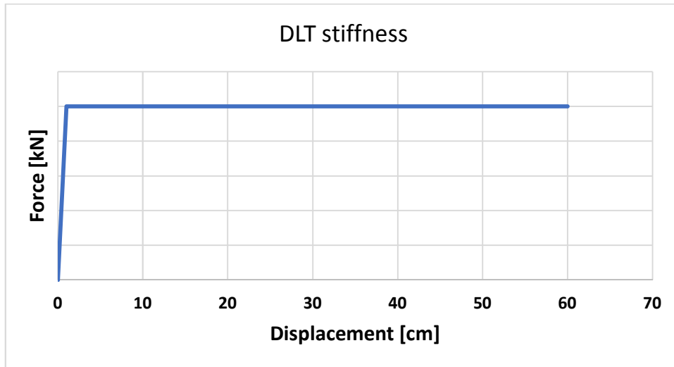
Figure 108 – Nonlinear stiffness of the DLT springs
