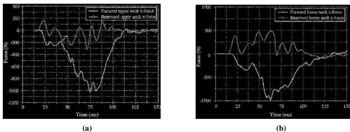
Figure 45 – Upper (a) and lower (b) neck x-force in forward and rearward facing CRS configuration [88]
