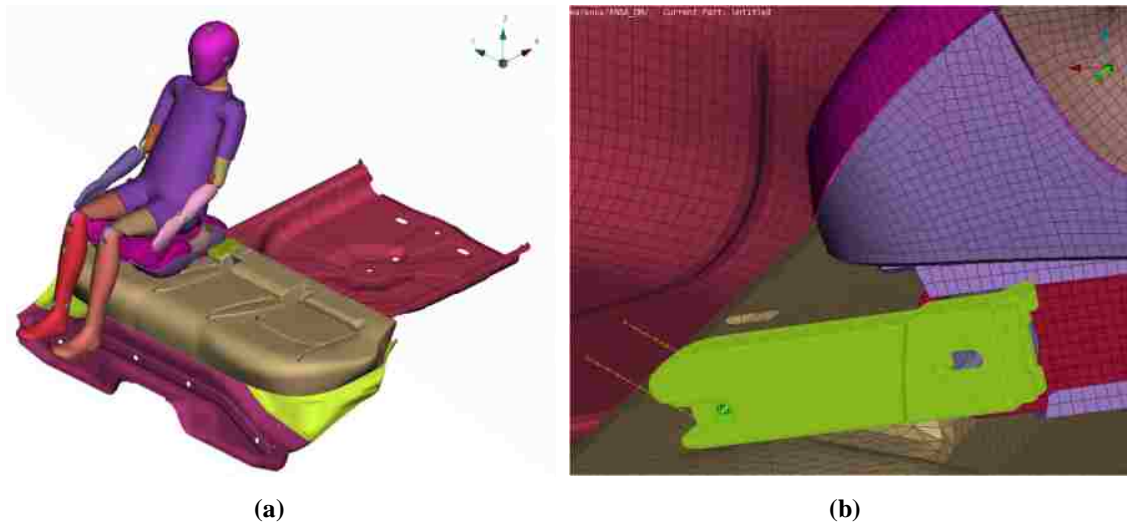
Figure 81 – Isometric view (a) of the LS-DYNA dummy seating simulation setting and detail of the extrapolated ISOFIX anchorage and the respective revolute joint (b)
