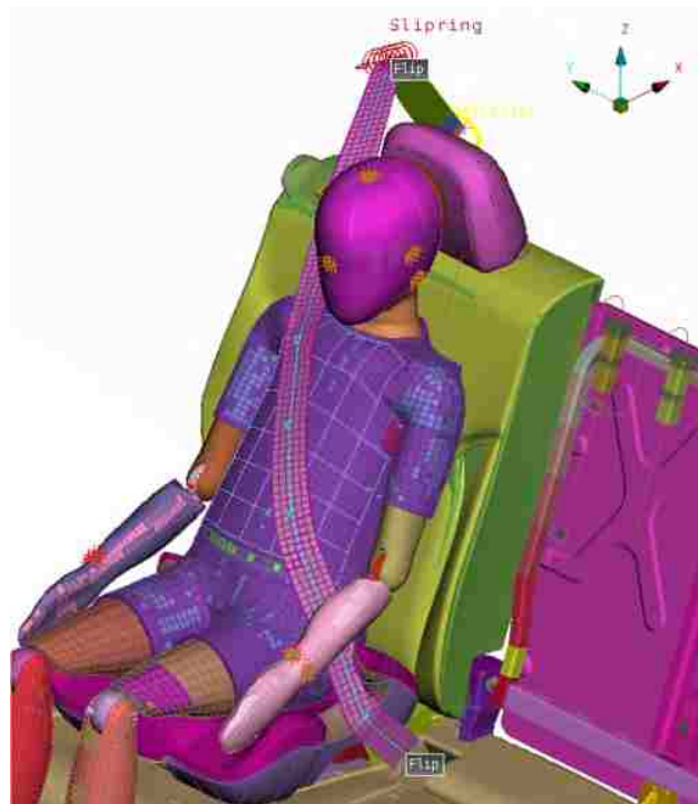
Figure 99 – Interactive edit of the shoulder belt
