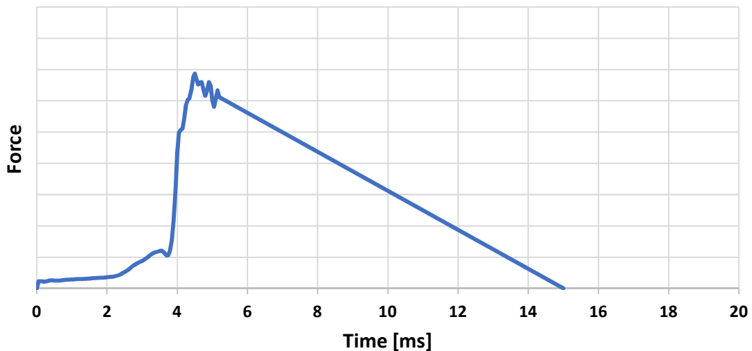
Figure 115 – Definitive pretensioner loading curve
