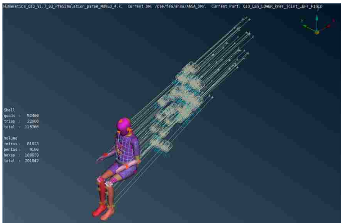
Figure 79 – Humanetics® Q10 presimulation file visualized through ANSA
