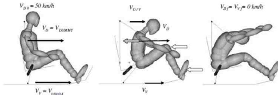
Figure 14 – Restrained occupant during a crash [9]
