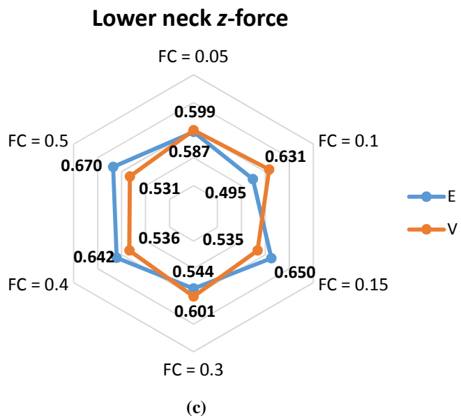
Figure 140 – Sensitivity analysis on the lower neck force
