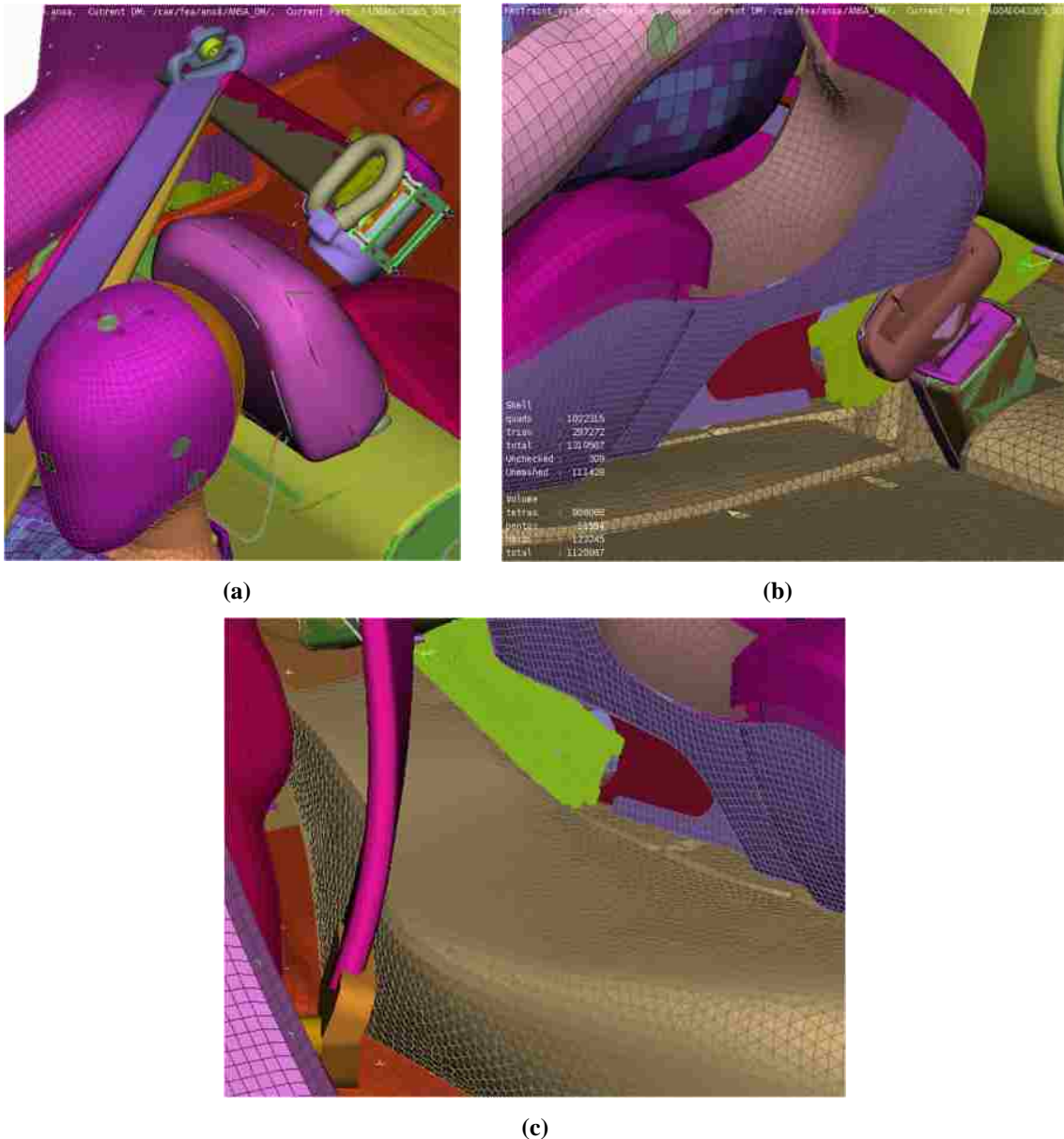
Figure 91 – Location of retractor and upper slip ring (a), locking tongue (b) and anchorage point (c)
