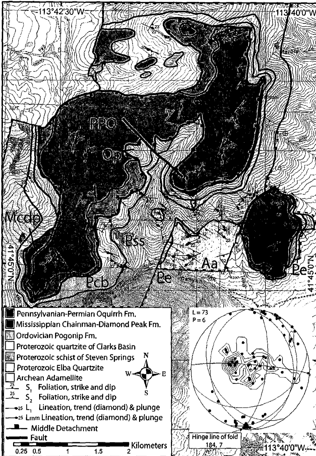
Figure 3. Geologic map of the Marble Peak klippe, showing the distribution and orientation of S 1 , S 2 , L 1 , L mm . Archean to Mississippian rocks show overprint of MMSZ; Pennsylvanian-Permian rocks preserve D 1 . Stereoplot shows lineations in red, poles to S 1 (black dots), S 2 axial cleavages (blue lines), and hinge line of fold (red box with black outline). Dashed grey line marks outline of map area. Contour intervals are 40 feet.
