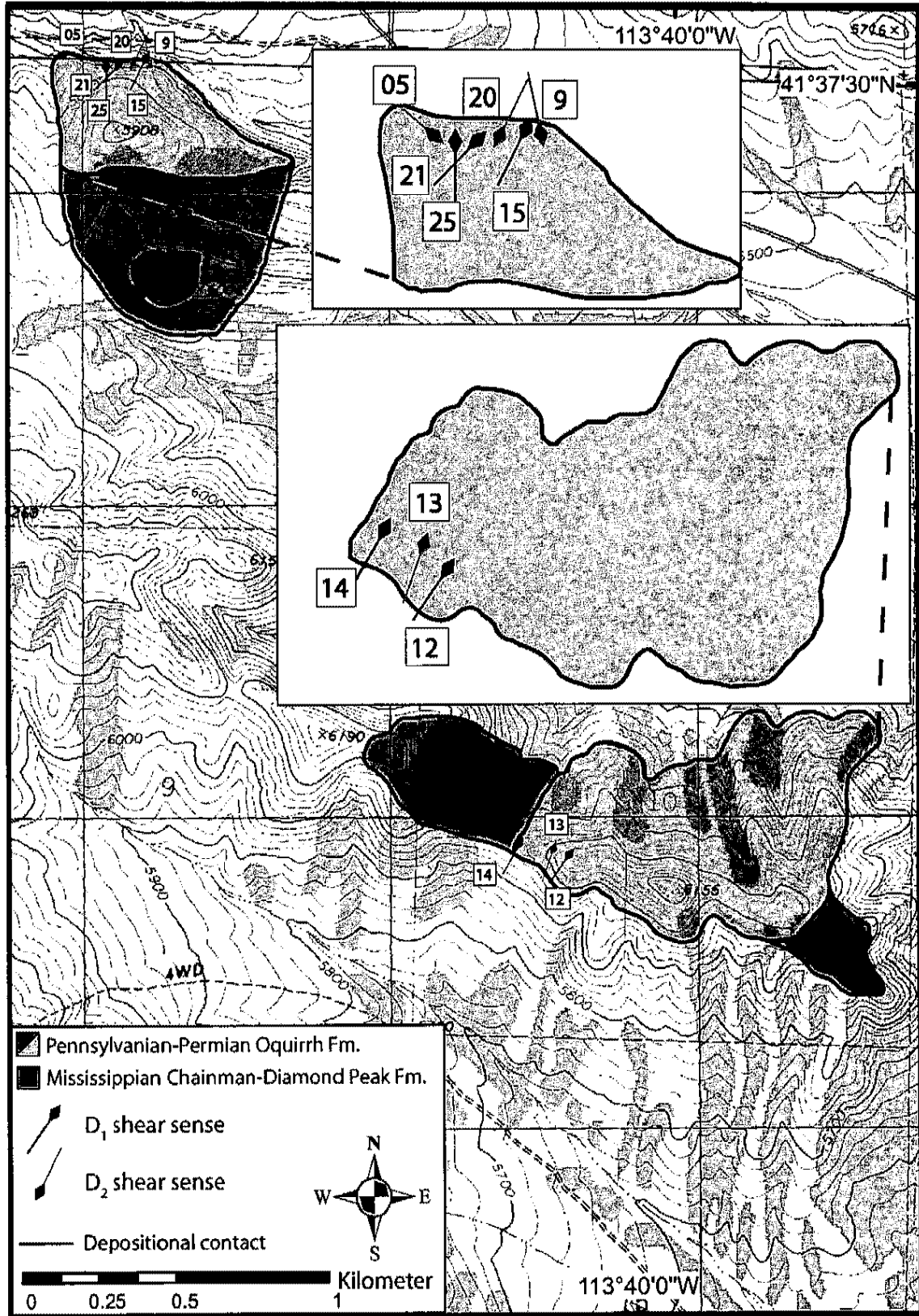
Figure 19. Simplified geologic map of Rosebud, showing D 1 top-to-the-north shear sense and D 2 top-to-the-south shear sense. Sample numbers are next to each arrow.
