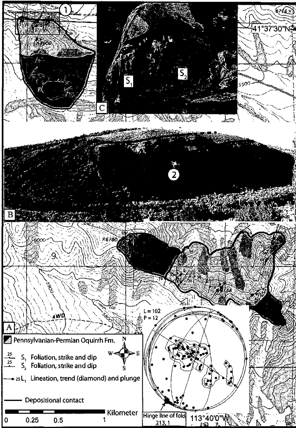
Figure 10. A, geologic map of Rosebud area with stereonet data showing L_1 elongation lineation in red dots, poles to the S_1 planes in black dots, and S_2 axial planar cleavage in blue lines. B, south-facing picture of the Rosebud fold exposed on a cliff face (box around area); red lines represent a form line, view to the south from circle 1. Dashed where interpretative. C, S_1 and S_2 relationship in a parasitic fold on the western limb, looking south at circle 2.
