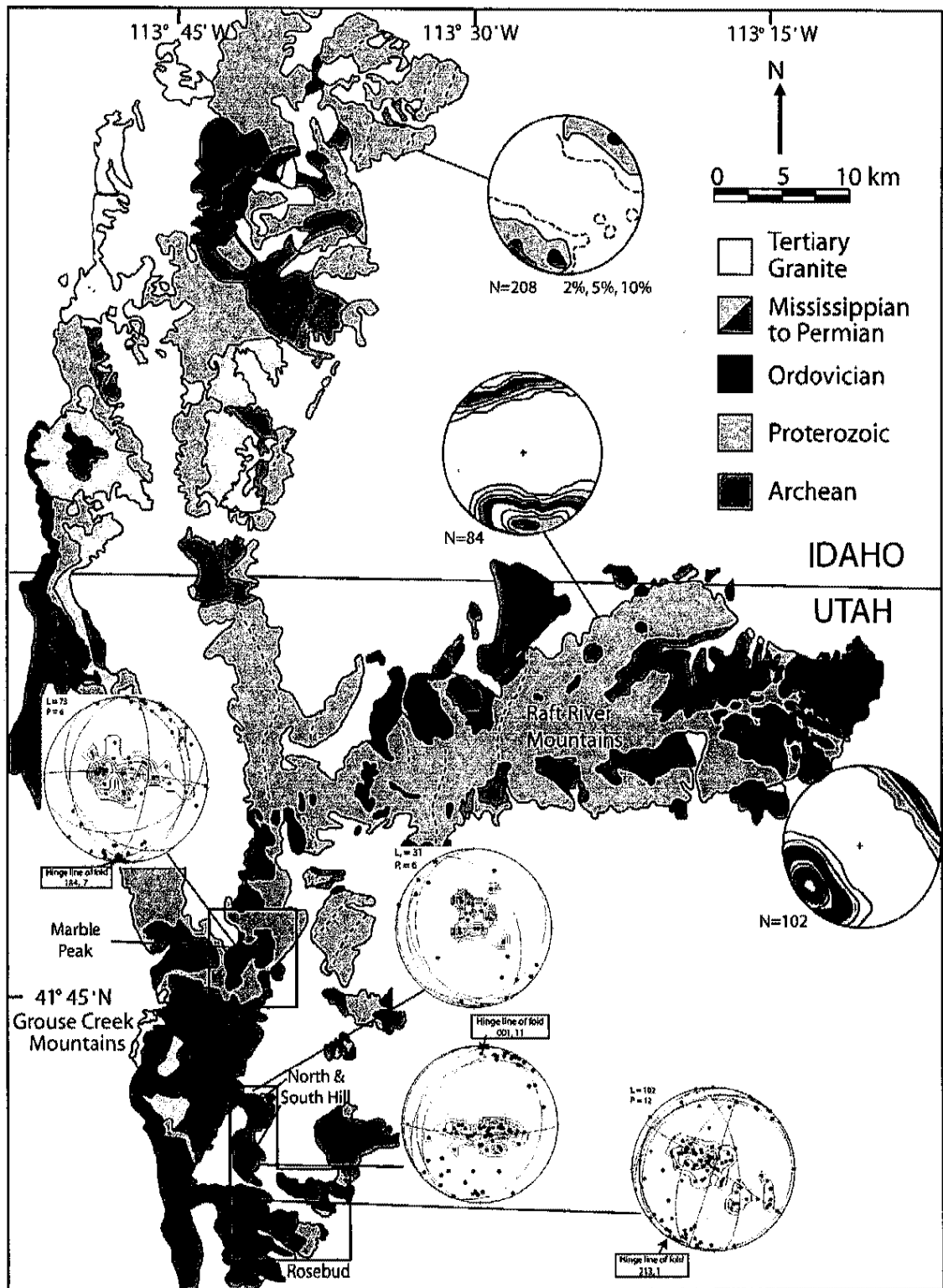
Figure 35. Generalized geologic map of Raft River-Albion-Grouse Creek Mountains (RAG) showing distribution of the L_1 stretching lineation. Field areas (in boxes) are at Marble Peak, North and South Hill and Rosebud area. Stereoplots showing L_1 from Compton (1972, 1975), Miller (1980), Todd (1980), Sheely (2002), Wells (1997), and this study. Modified from Wells et al. (2008).
