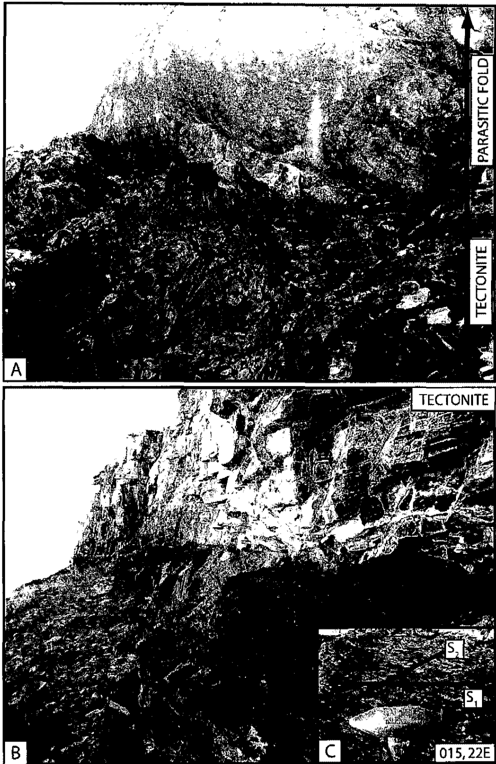
Figure 13. A, contact between the Oquirrh Formation limestone and the Oquirrh Tectonite in a parasitic fold in the South Hill fold. B, quartz rich section below the tectonite. C, relationship between the axial planar S_2 cleavage and the flat-lying S_1 foliation. This relationship along with orientation data indicates that the tectonite at South Hill is in the overturned limb of the east-vergent recumbent fold. Hammer for scale. Photograph facing southwest.
