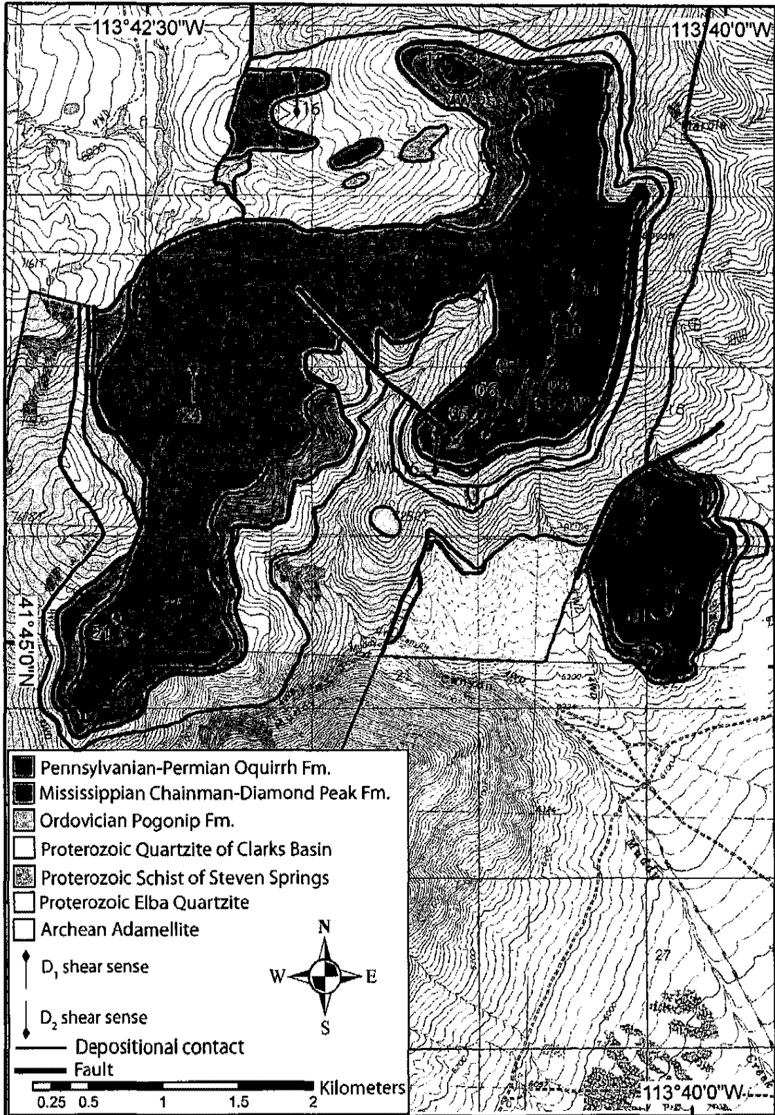
Figure 17. Simplified geologic map of Marble Peak, showing D 1 top-to-the-north shear sense and D 2 top-to-the-south shear sense. Southward shear sense from D 1 fibers was recorded within the Chainman-Diamond Peak Formation in the northern part of the map, overprinted by the D 2 deformation. Sample numbers are next to each arrow.
