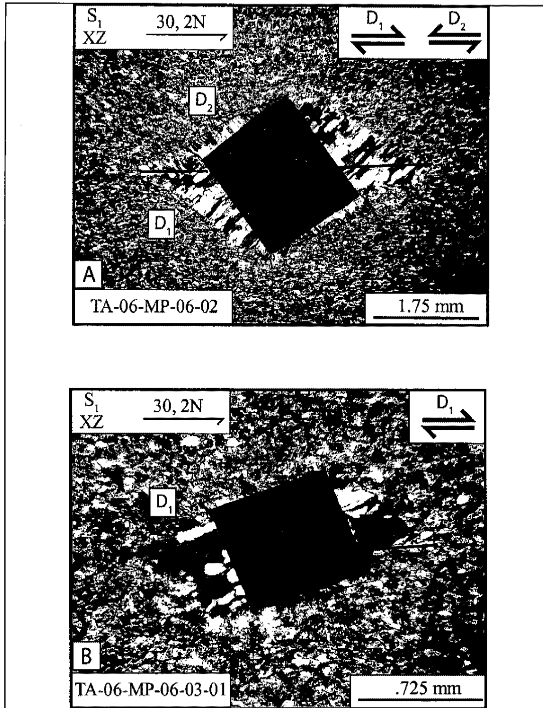
Figure 16. Photomicrograph A is showing both D_1 and D_2 strain fringes within the XZ plane of S_1 at Marble Peak. D_1 displays face-controlled fibers and D_2 exhibits displacement-controlled fibers. D_1 records top-to-the-north and D_2 records top-to-the-south shear sense. Photomicrograph B shows D_1 face-controlled fibers within the XZ plane of S_1 at Marble Peak. D_1 shear sense records top-to-the-north shear sense.
