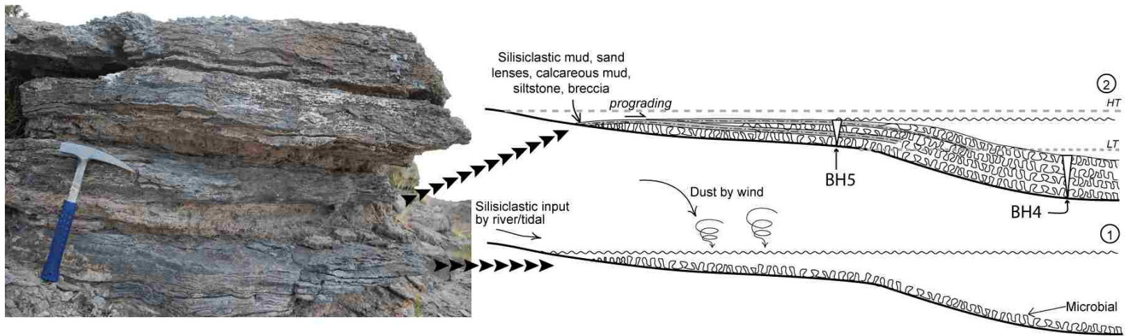
Figure 16. An example showing the formation of microbialite-rich peritidal cycles. Microbial mats occupied the sedimentary substrates in shallow subtidal to intertidal environments, forming flat-wavy microbialites. During the late stage, local subaerial exposure and siliciclastic input forced the migration of the microbial mats. Thus, the upper intertidal facies in section BH5 consists of different internal facies and centimeter-scale cycles, while 200 m away in section BH4, the lower intertidal facies contains only one cycle with homogeneous lithofacies.
