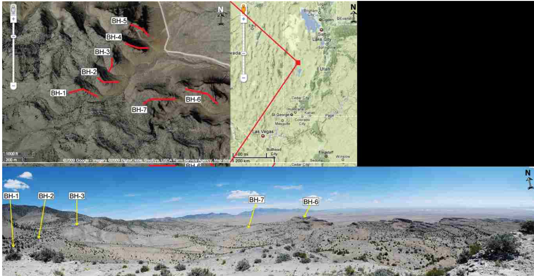
Figure 1. (a) A google earth image and map showing the location of study area in the Little Horse Canyon, western Utah. The location is at N 39^{\circ} 12.412' , W 113^{\circ} 18.450' . (b) The outcrop consists of the Big Horse Member of the Orr Formation, which was deposited during early Furongian time (see Figure 2). The excellent exposure in this area allows for a detailed sedimentological study in closely spaced sections (BH1 – BH7) and for lateral tracing of key surfaces, cycles, and facies.
