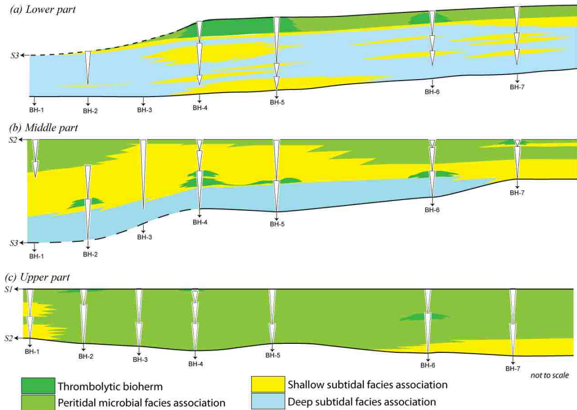
Figure 17. Schematic diagram showing the autogenic origin of cycles and their lateral variations. (a) In the lower part (below S3 in Figures 3 and 4) of the measured sections, the depositional environments were subtidal dominated. Local development and migration of shallow subtidal, carbonate sand shoals/bars formed the grainstone/packstone-capped subtidal cycles. At the end of this interval, carbonate sand shoals extended and covered the entire studying area, with local thrombolite bioherms developed at the top. The end of this interval is represented by a karstic surface (S3), indicating the filling of available accommodation space. Subsequent creation of accommodation space is most likely caused by an episode of tectonic subsidence. (b) After an episode of tectonic subsidence, the middle part of the studied sections (between S3 and S2) had initial transgression and deepening, but shortly changed to shallow-subtidal-dominated environments. Migration of carbonate sand shoals and local development of thrombolite bioherms created meter-scale cycles that are laterally discontinuous. (c) Creation of the accommodation space needed for the deposition of the upper part of the measured sections (between S2 and S1) requires another episode of tectonic subsidence, shortly after the development of surface S2. The background depositional environments representative of this intervals were microbially colonized peritidal environments, within which local development of carbonate sand bars and thrombolite bioherms formed the laterally discontinued cycles.
