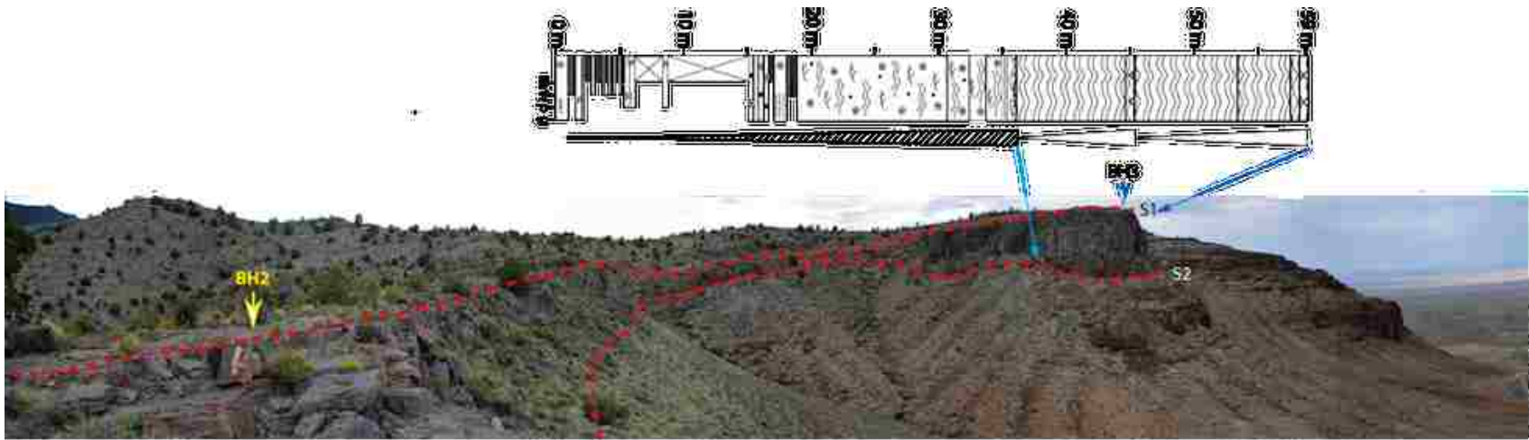
Figure 14. Tracing of carbonate cycles from section BH2 to BH3. The thickness of the interval between S1 and S2 changes significantly over the 250 meter between measured sections.
