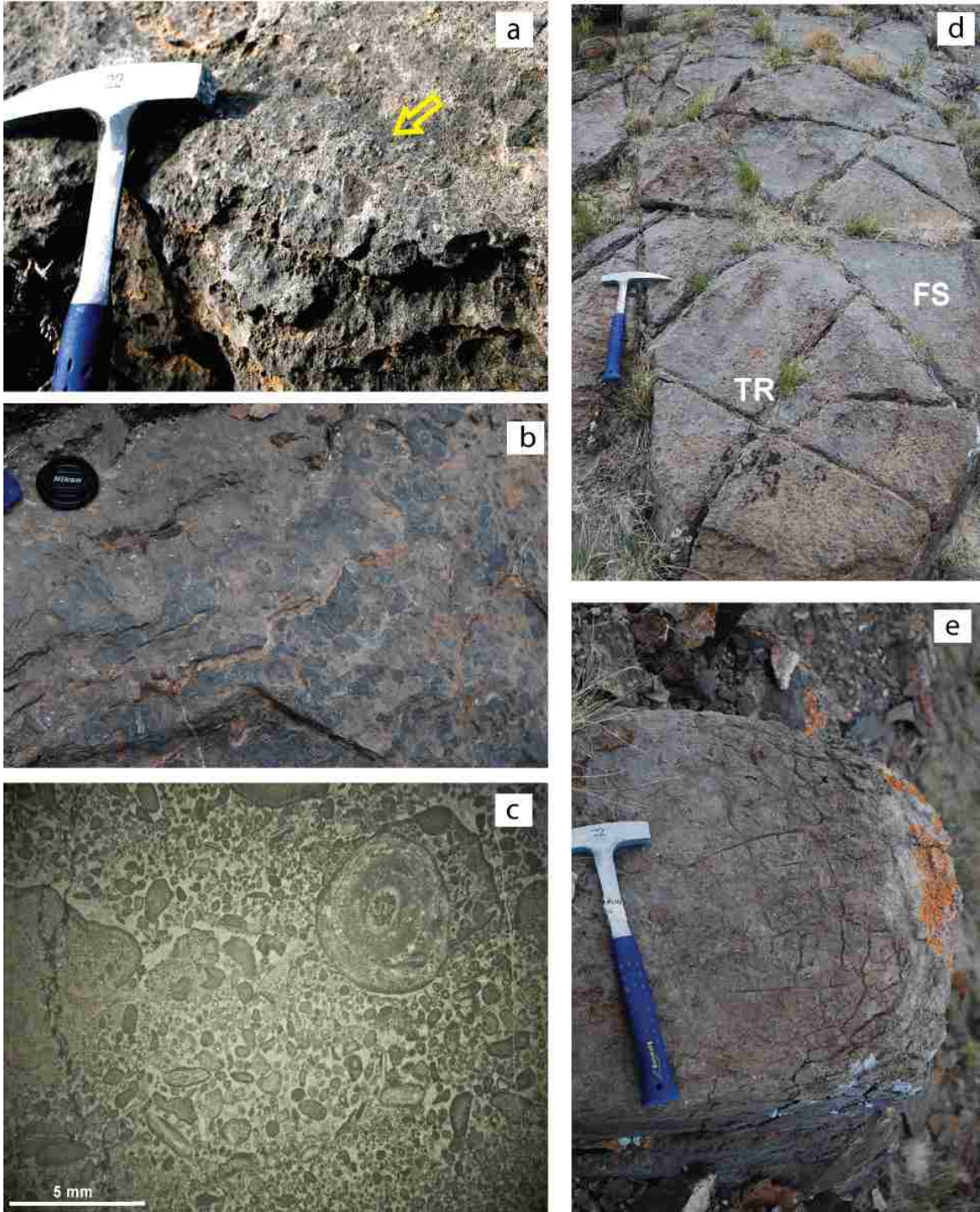
Figure 9. Subaerial exposure features. (a) Lithoclasts (yellow arrow) with silty dolostone matrix (karst breccia) along a karstic surface, occurs at 38 m in section BH1. (b) Cemented coated grains commonly appear as calcrete facies on an exposure surface. Lens cap for scale is 76 mm in diameter. (c) Intraclastic rudstone/floatstone commonly appear discontinuously along an exposure surface and consist of carbonate aggregates, oncoids, pellets, and ooids. Plane polarized light. (d) Thrombolite humps (TR) and rudstone/floatstone (FS) filling the spaces among thrombolite humps (FS, i.e., aggregates, and rudstone).
