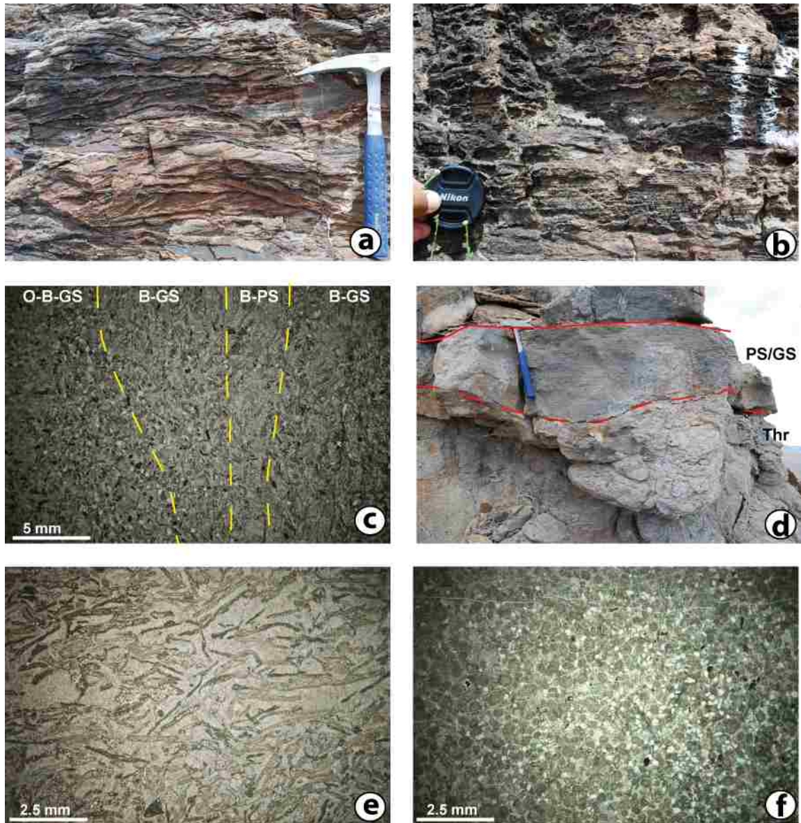
Figure 7. Field and petrographic photos of the shallow subtidal facies association. (a) Bioclastic and oolitic grainstone showing cross stratification (from section BH-3, interval 19 m). Microbial laminae along bedding planes of cross stratification imply the importance of microbial processes in formation and preservation of cross beds. Hammer for scale is 32.5 cm long. (b) Interbedded microbial laminae and cross-stratified grainstone/packstone. Microbial laminae are laterally discontinuous and pinch out towards thick grainstone/packstone beds. (c) Petrographic view of the alternating oolitic-bioclastic grainstone (O-B-GS), bioclastic grainstone (B-GS), and bioclastic packstone (B-PS). Plane polarized light. From section BH-3 at 23.5 m. (d) Relationship between bioclastic-intraclastic packstone/grainstone and thrombolitic bioherm. The karstic surface (dashed line) between the grainstone/packstone layer and its underlying bioherm marks the top of a thrombolite-capped cycle. Hammer for scale is 32.5 cm long. (e) Thin section view of the bioclastic packstone from section BH-4 at 1 m. Bioclasts include fragment of
