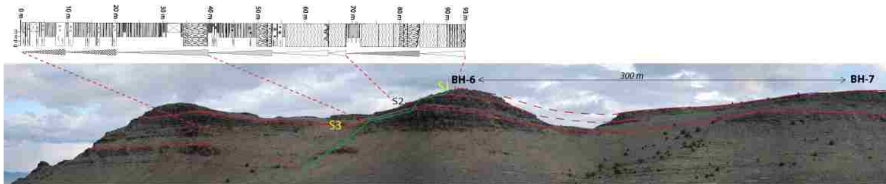
Figure 13. Correlation panel of carbonate cycles in sections BH6 and BH7. The three main surfaces (S1, S2, S3) are traceable from BH-6 to BH-7, but the thickness and facies components are different. The facies below S3 shows a localized thrombolite bioherm.
