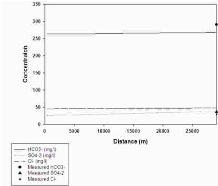
Figure 2.9 Simulated results of anion transport from the Spring Mountains to Amargosa Desert with comparison to the measured anion concentrations. Black solid line- simulated carbonate hydrate concentration; black dot line- simulated sulfate concentration; black dashed line- simulated chloride concentration.
