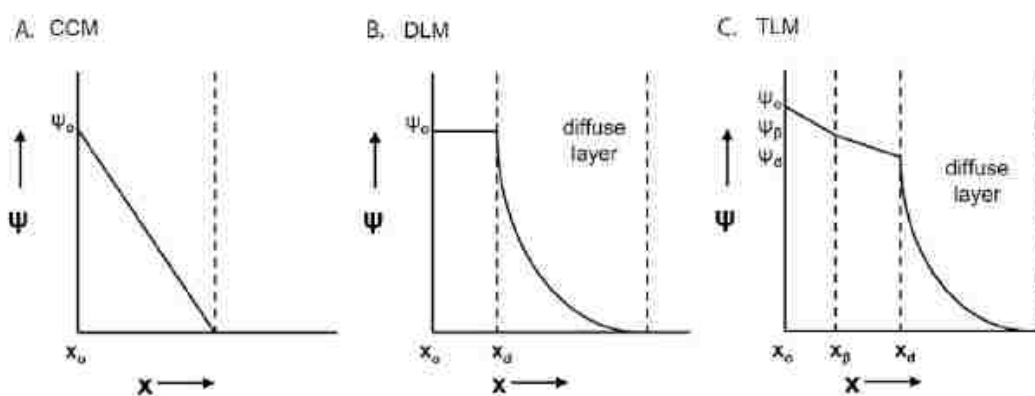
Figure 1.4 Schematics of the interface between solid and solution in A-constant capacitance model (CCM), B-diffuse layer model (DLM), and C-triple layer model (TLM), respectively (from Goldberg et al., 2007). Note that \Psi is the surface potential; x_o is the surface o-plane; x_d is the diffuse layer; x_\beta is the outer \beta -plane; x is the distance from the surface o-plane.
