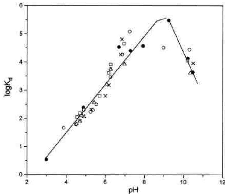
Figure 3.6 Variation of the logarithm of distribution coefficient of Yb with pH: (•) 0.01 mol/l NaNO 3 ; (o) 0.1 mol/l NaNO 3 ; (x) 0.5 mol/l NaNO 3 ; (Δ) 1.0 mol/l NaNO 3 ; (□) 2.0 mol/l NaNO 3 (from Wang et al., 2000)
