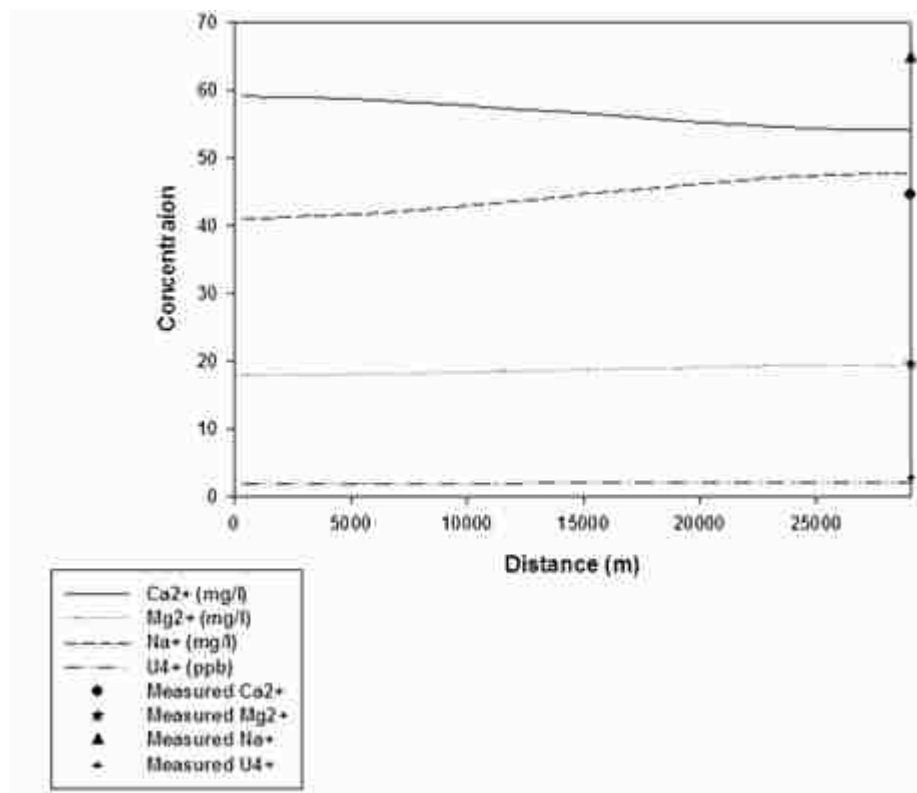
Figure 2.8 Simulated results of cation transport from the Spring Mountains to Amargosa Desert with comparison to the measured cation concentrations. Black solid line- simulated calcium concentration; black dot line- simulated magnesium concentration; black dashed line- simulated sodium concentration; black dot dashed line- simulated uranium concentration.
