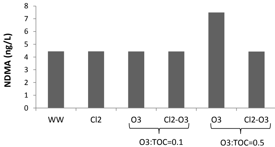
Figure B.3: NDMA concentration for site B after chlorination and ozonation at two O 3 :TOC
