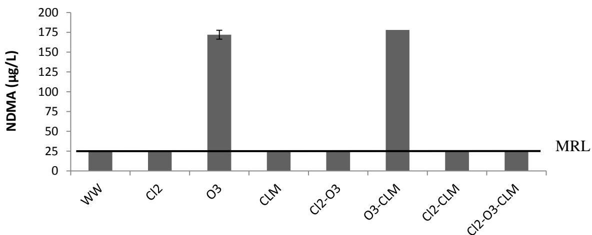
Figure 5.4: NDMA formation after disinfection treatment schemes for Site F wastewater spiked with ozone-reactive NDMA precursors. Error bar is the standard deviation (n = 2). The horizontal line is the method reporting limit (MRL).
