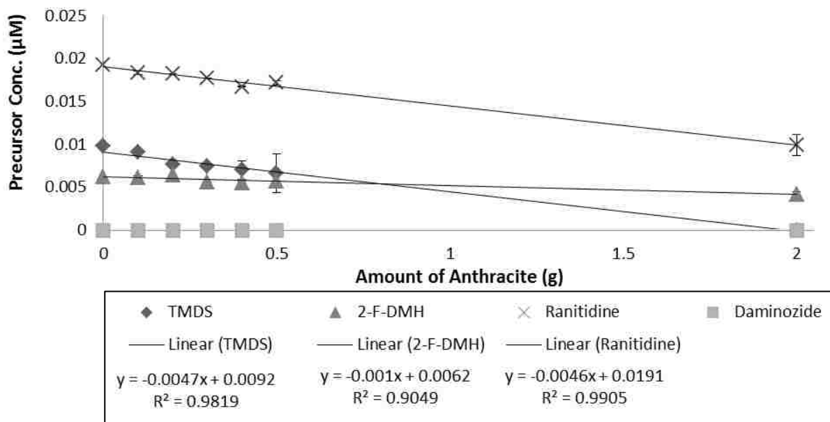
Figure 6.3: Batch sorption results and linear regressions for NDMA precursors in tertiary-treated wastewater at pH 6.9 after 24 hours in contact with fresh anthracite.
