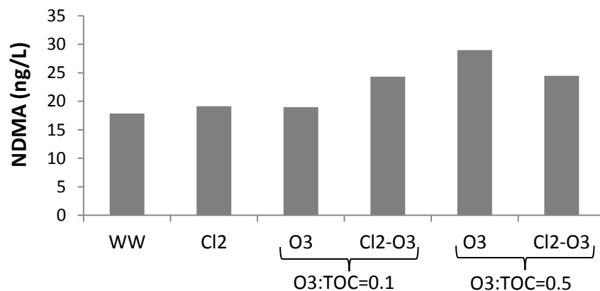
Figure 5.1: NDMA concentration for site C after chlorination and ozonation at two O 3 :TOC ratios. Similar results were obtained for sites A and B (Appendix B).
