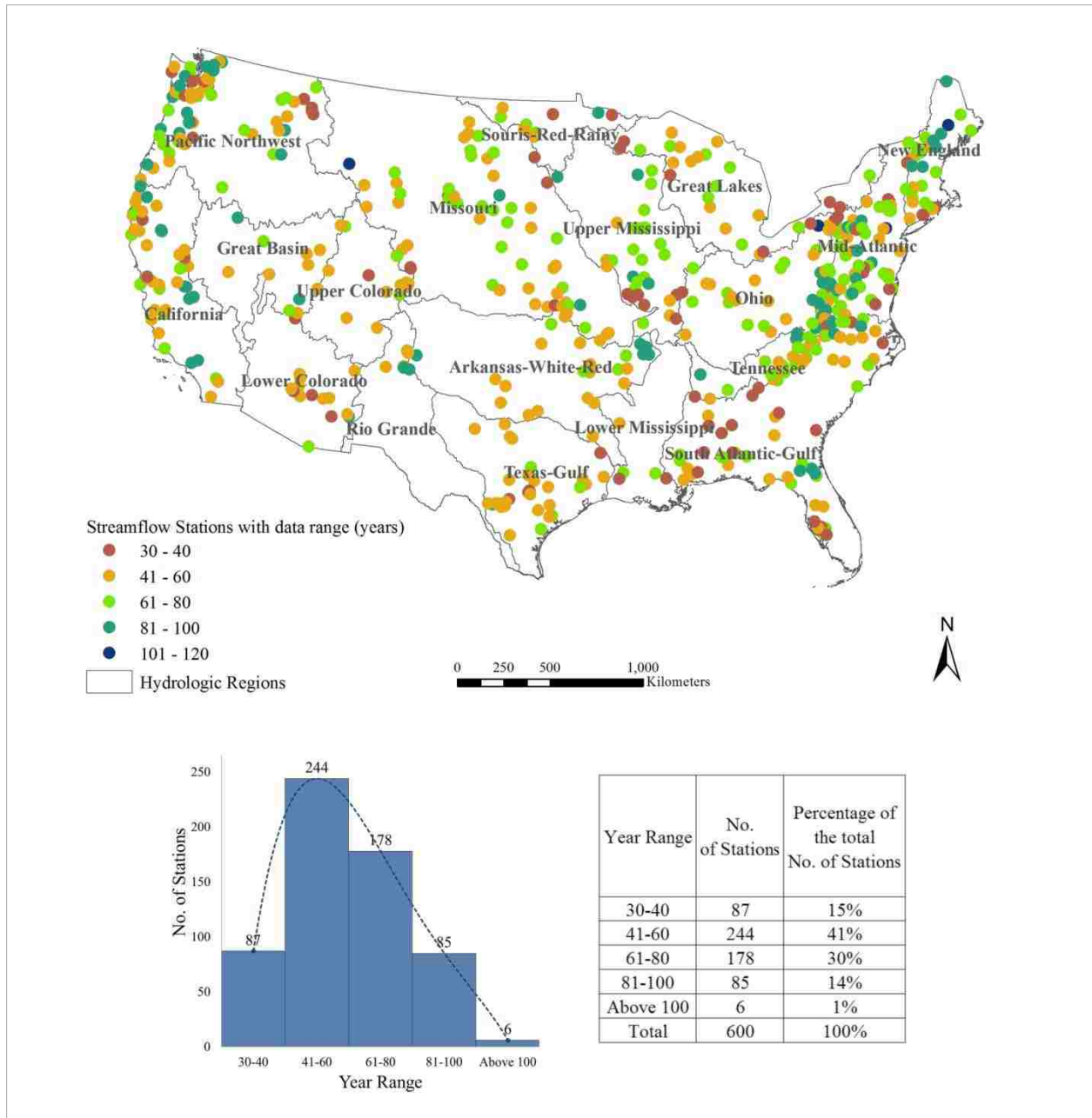
Figure 2.1: (Top) Map of the continental U.S. with 600 unimpaired streamflow stations across 18 hydrologic regions with available data range in years. (Bottom left) Distribution of the number of stations with varying ranges of data availability from 30 to 40 years, from 41 to 60 years, from 61 to 80 years, from 81 to 100 years and above 100 years. (Bottom right) Table showing the comparative percentages of the stations in each range of years.
