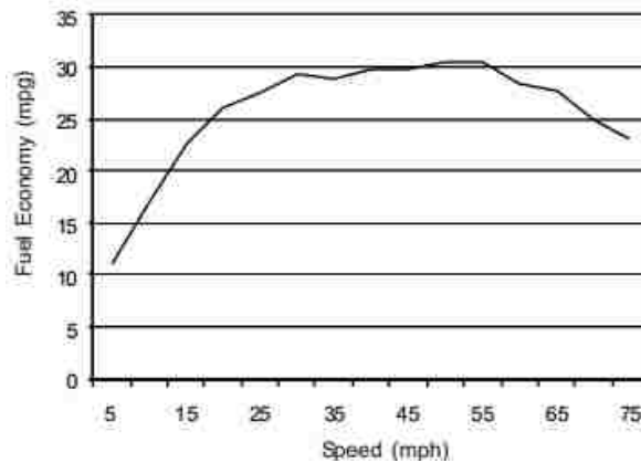
Figure 3-1. Fuel Economy and Speed (Source: USDOE)
