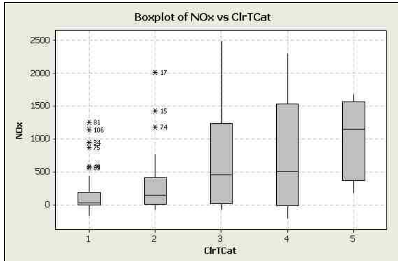
Figure 7-30. Box-plot: Excess NO x emissions (in Grams) vs. Incident Duration
