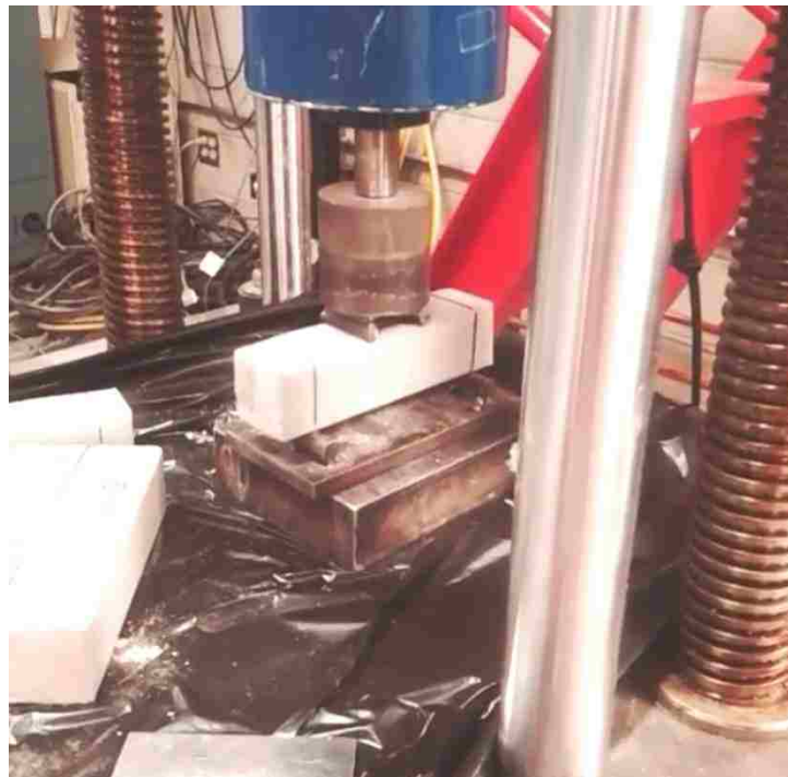
Figure 2.13. Four-Point Flexural Strength Test Set-Up
