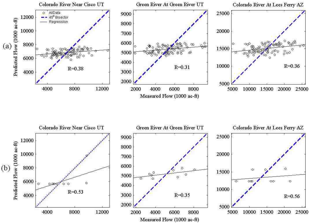
Figure 25: ANN predicted streamflow volumes at ‘t+3’ for model I for (a) training phase and (b) testing phase at the three selected gages. Dashed line is the 45^{\circ} bisector and solid line is true regression line between the measured and predicted streamflow volumes.
