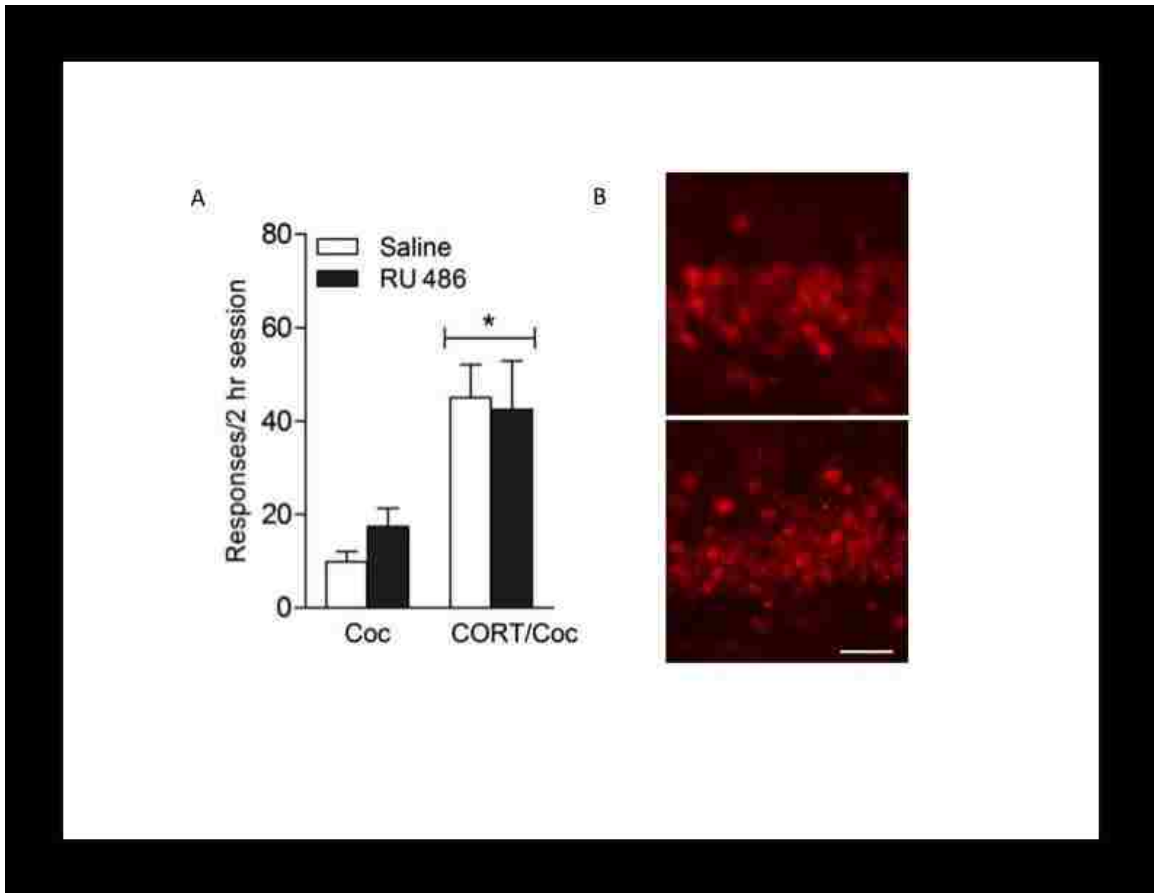
Figure 8. Effects of the glucocorticoid receptor antagonist RU38486 and corticosterone treatment on cocaine-induced reinstatement. (A) Rats (n=10) were given an injection of RU38486 (12.5 mg/kg, sc) or vehicle 60 minutes prior to an injection of corticosterone (2.0 mg/kg, ip) or vehicle. This was followed 40 minutes later by an injection of cocaine (2.5 mg/kg, ip). Data represent mean \pm SEM of active lever responses over a 2-hour period following the final injection. Significant increases in responding were seen in animals which received corticosterone and cocaine, regardless of RU38486 pretreatment. * p < 0.05 compared to saline/coc and RU38486/coc conditions. (B) Photomicrograph of GR immunofluorescence in the dentate gyrus of ADX rats treated with vehicle (top) or RU38486 (bottom). RU38486 induced nuclear translocation of GR. Scale bar = 25 \mu m
