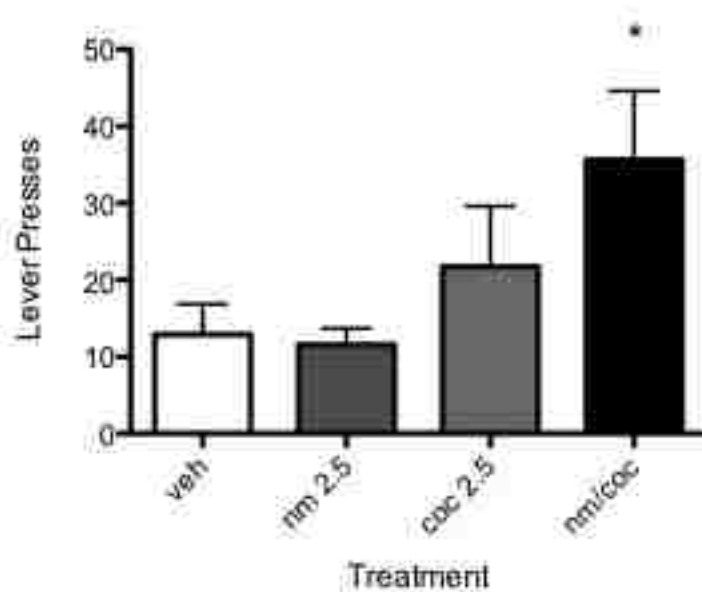
Figure 15. OCT3 inhibition enhances cocaine-induced reinstatement. Animals received vehicle or the OCT3 inhibitor normetanephrine (nm, 2.5 mg/kg, ip), followed by a low dose of cocaine (2.5 mg/kg) or vehicle. Normetanephrine potentiated low-dose cocaine-induced reinstatement. (Repeated measures ANOVA with Tukey post hoc test. * indicates p < 0.05 compared to veh and nm 2.5 groups).
